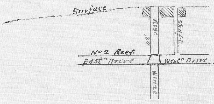
Long Section
