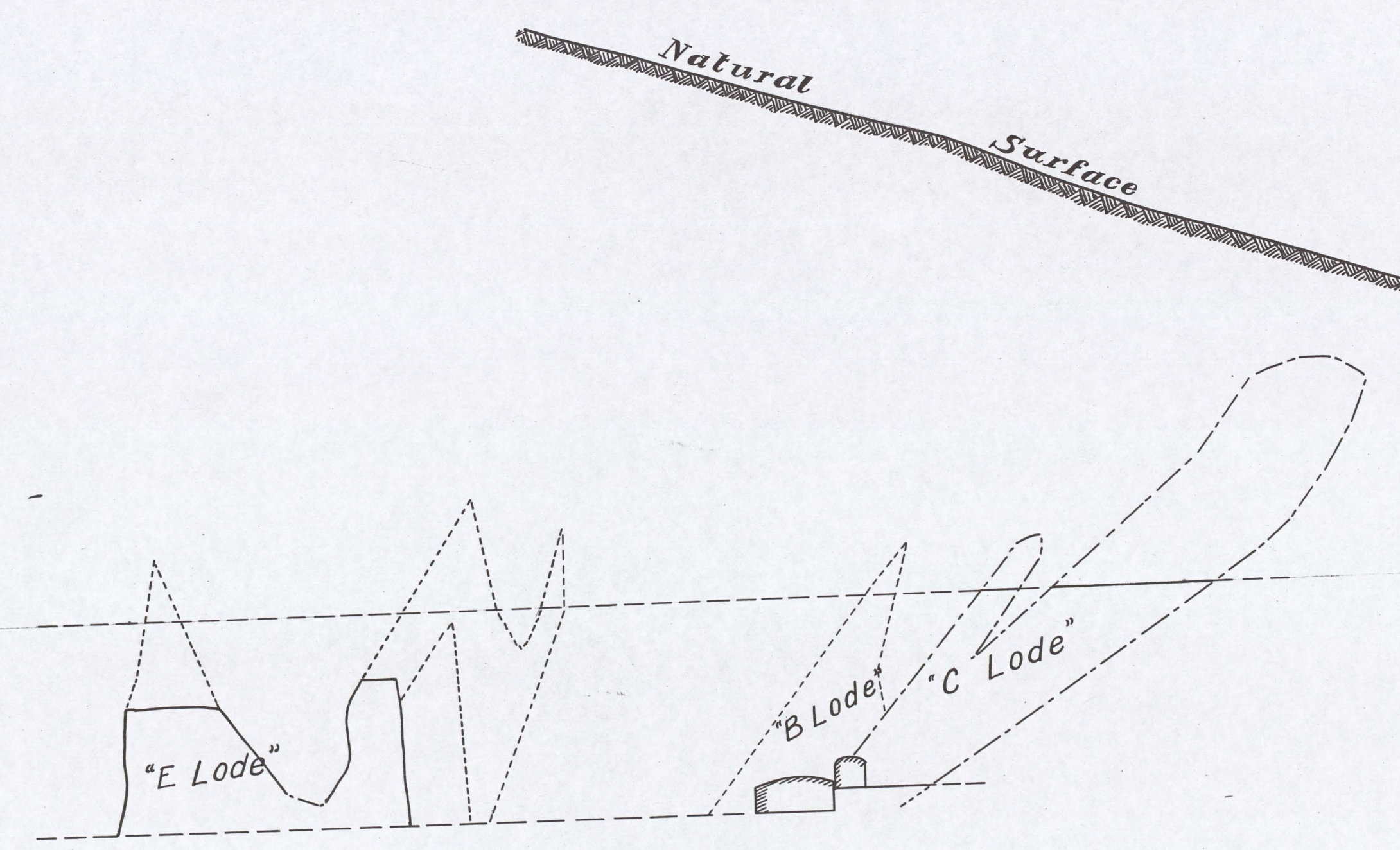
Nº5 SECTION
