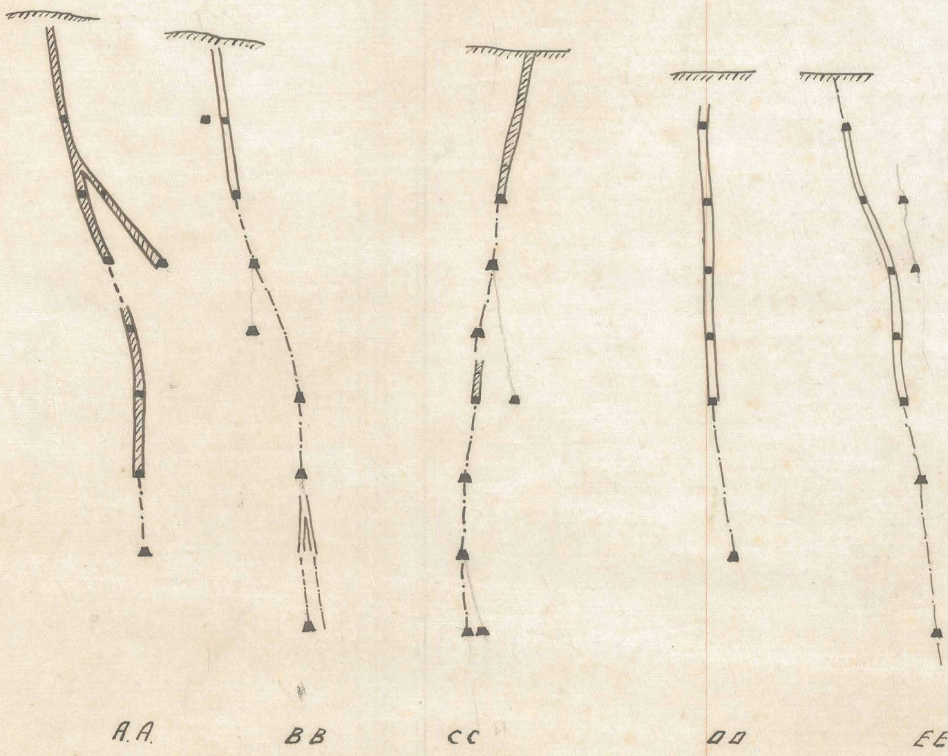
Cross Sections of N°1 Lode
