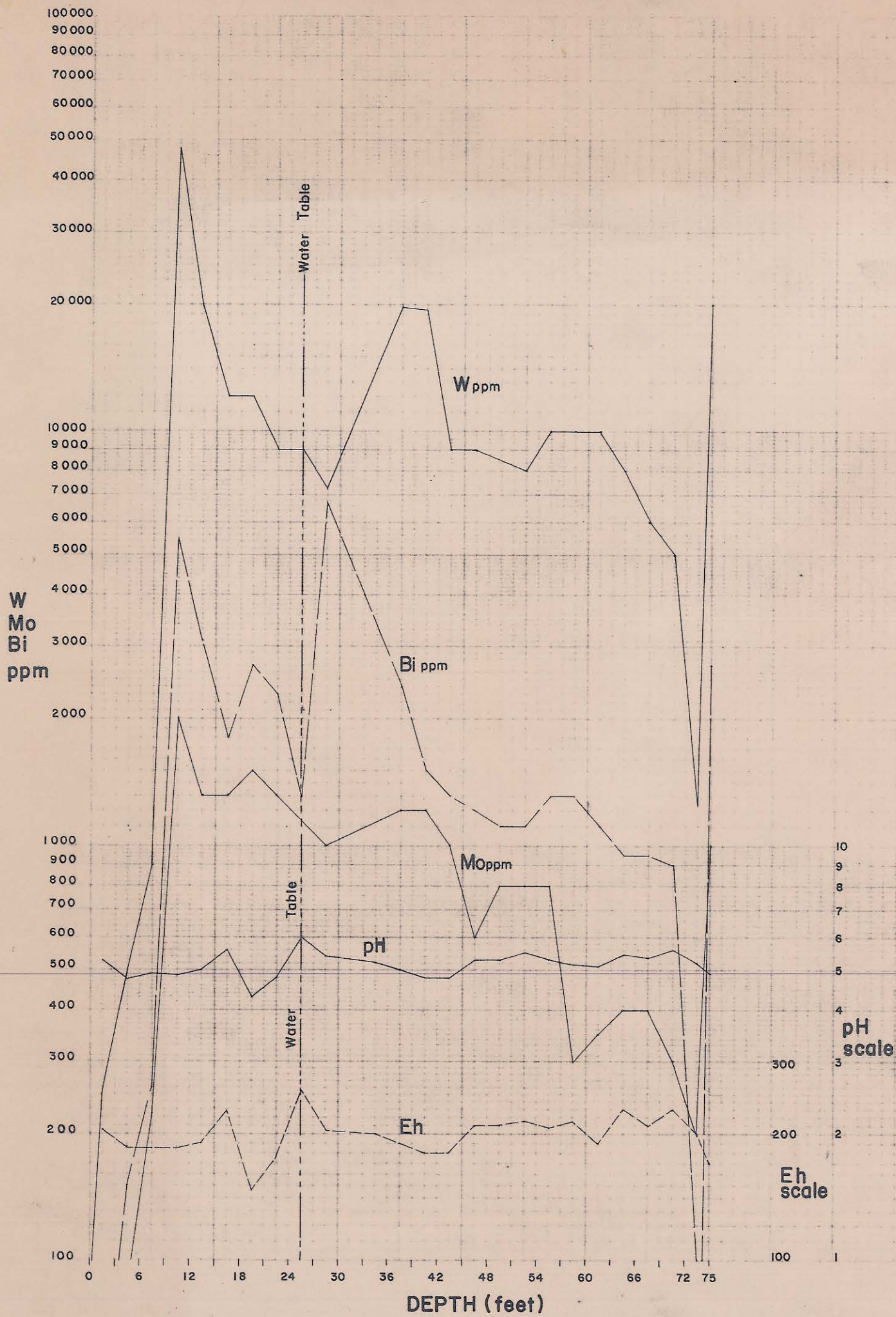
Fig. 7 Downhole geochemical profiles for W, Mo, Bi, and pH, Eh for drill hole (10100N, 400E).
