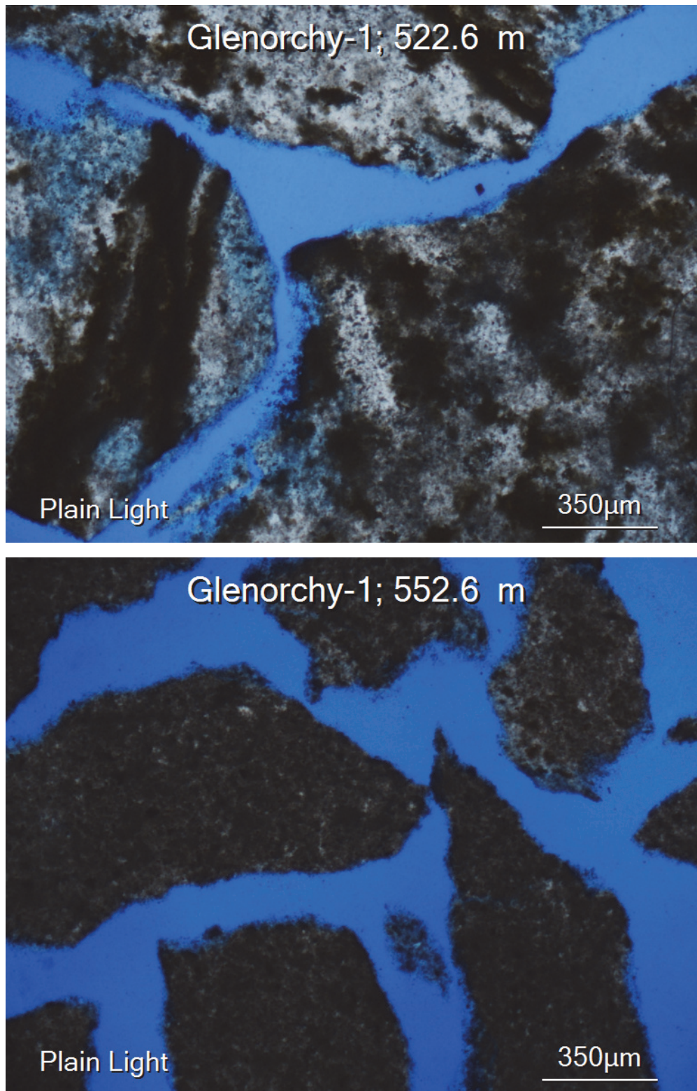
Figure 14: Photomicroscopy from Glenorchy-1
