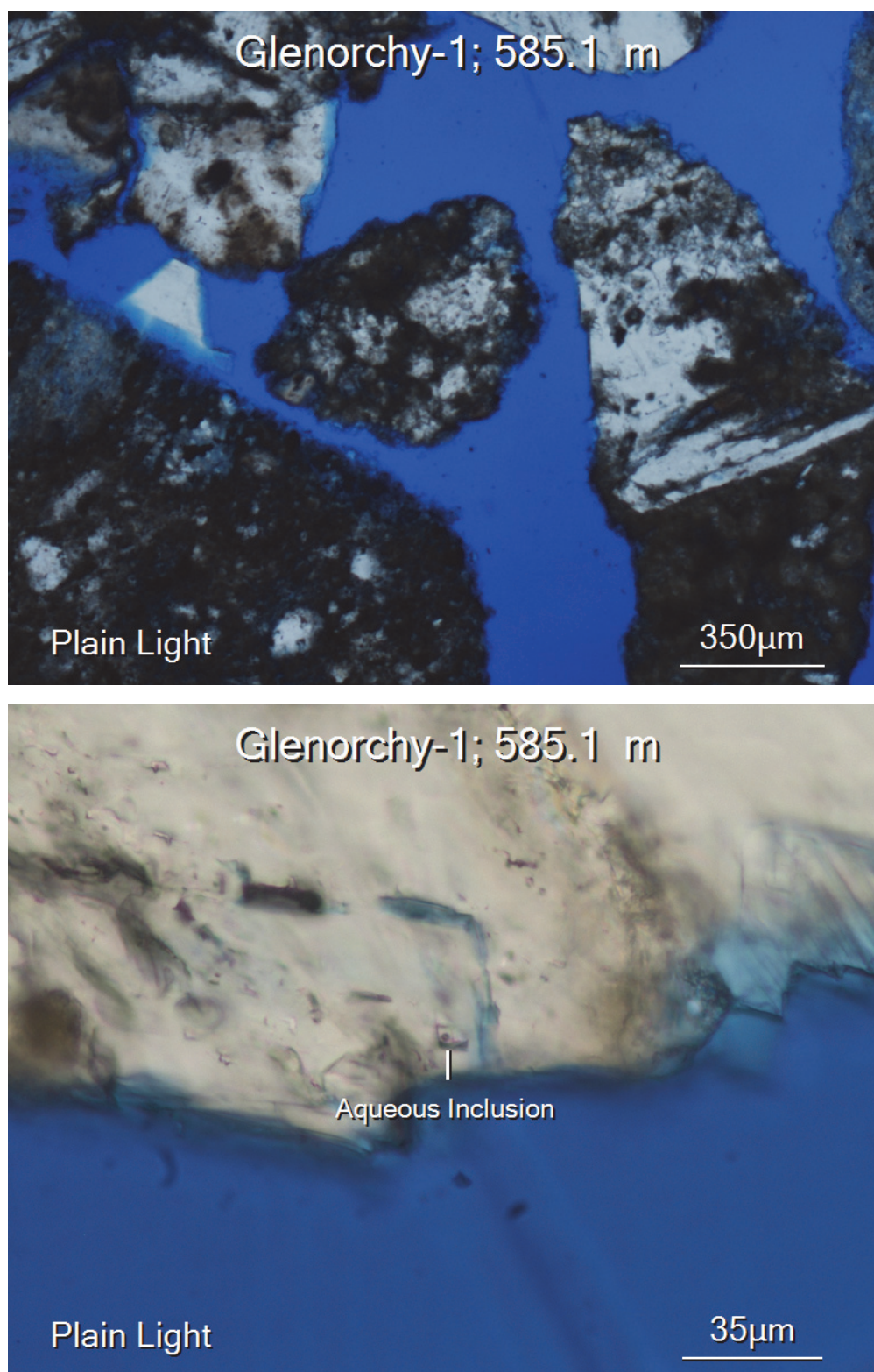
Figure 15: Photomicroscopy from Glenorchy-1
