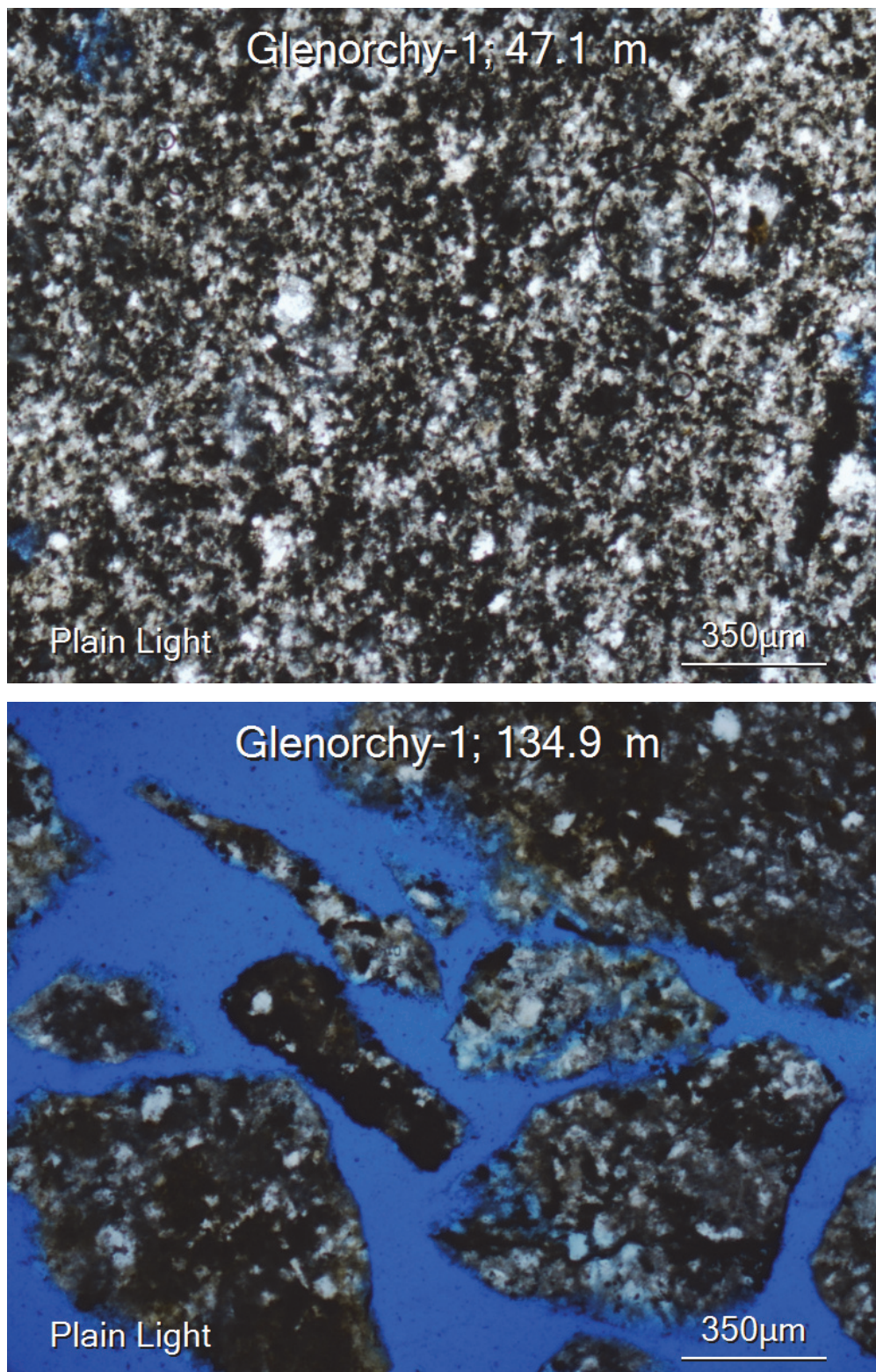
Figure 12: Photomicroscopy from Glenorchy-1
