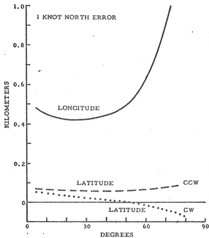
Fig. 5. Satellite Fix errors at Latitude 32^{\circ}\text{N} , Due to Forced Dead Reckoning Errors.
