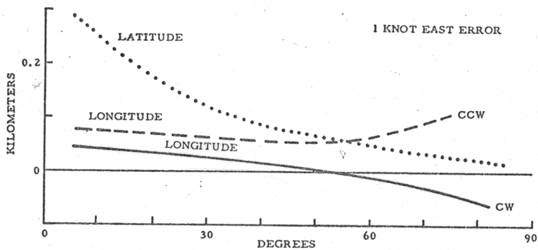
Fig. 6. Satellite Fix Errors at Latitude 32^{\circ}\text{N} , Due to Forced Dead Reckoning Errors.
