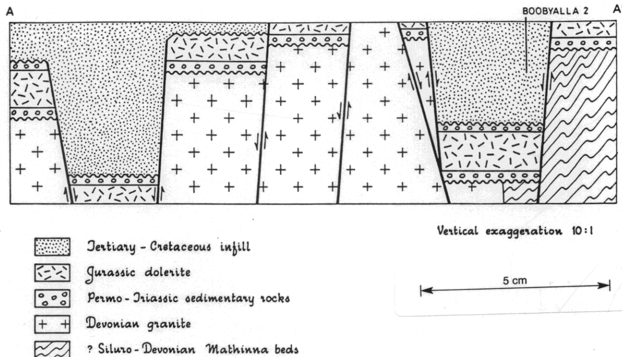
Figure 7 — Diagrammatic cross-section constructed along line A-A' of Figure 5.
