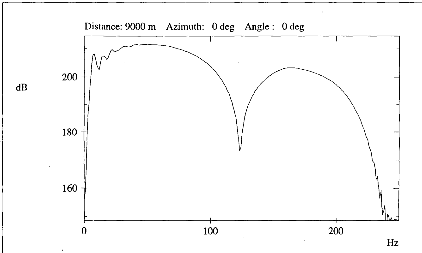
Amplitude spectrum of far-field signature of array: S266060a
