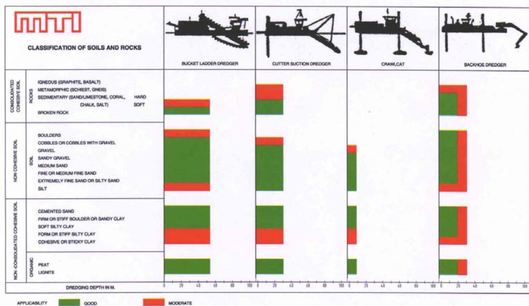
DREDGING EQUIPMENT AND APPLICABILITY
