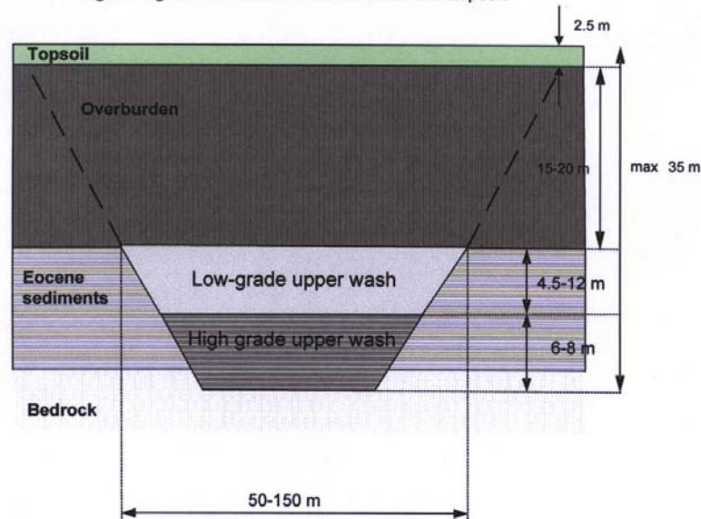
Figure 1: Cross-section Scotia deposit
