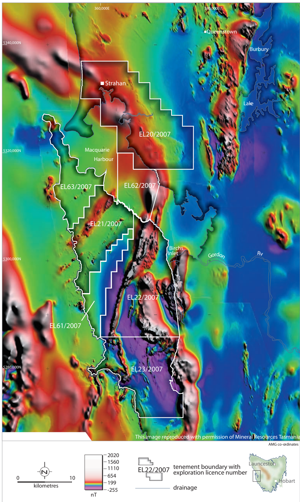
FIGURE 2: Magnetic Map Macquarie Harbour Area
