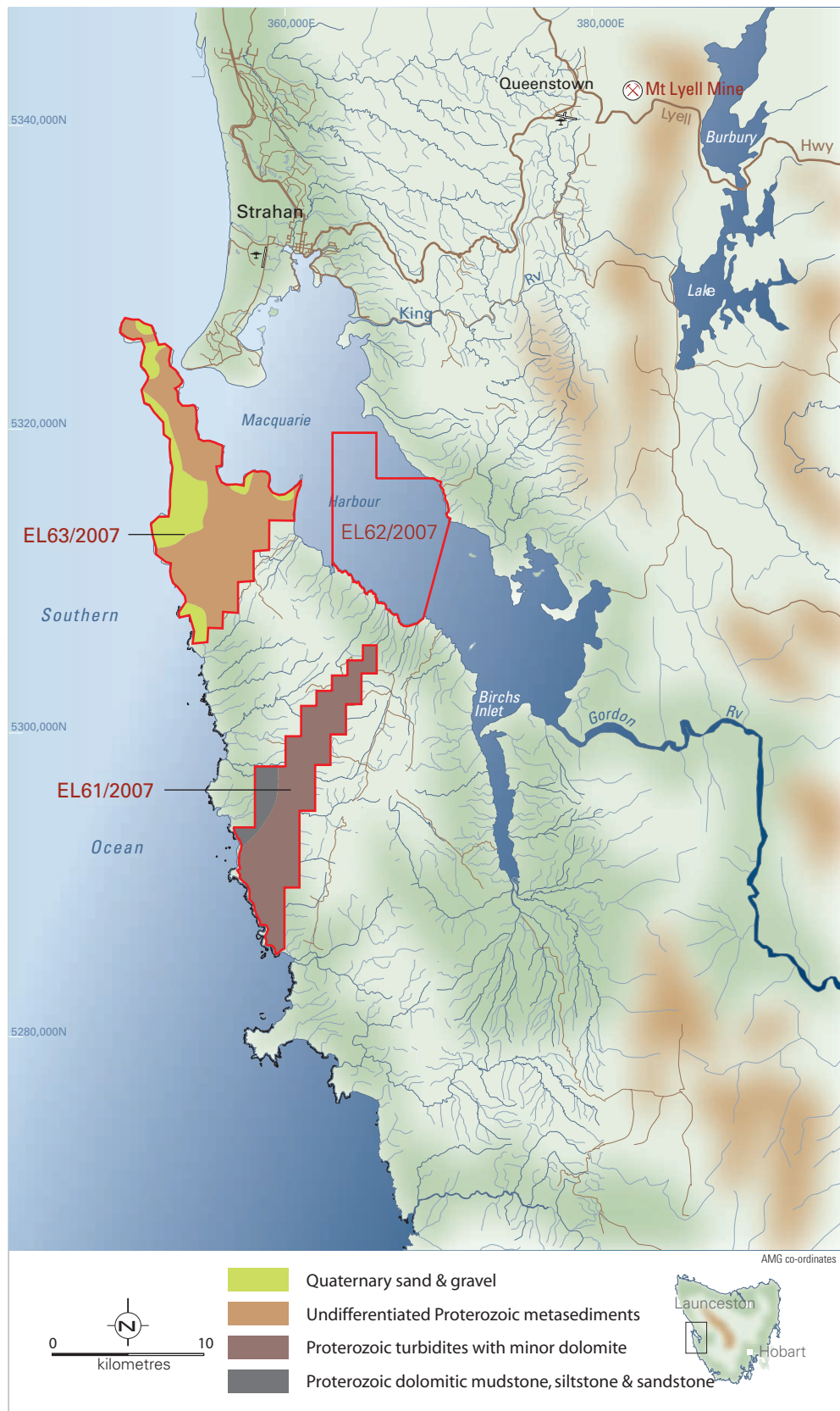
FIGURE 3: Geology of EL's 61 & 63/2007
