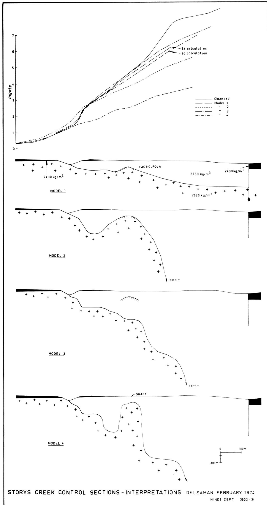
Figure A4.2 – Storeys Creek Control Section: Proposed subsurface structure models derived from gravity data over Storeys Creek (reproduced from Report TR19_55_81, Figure 18)
