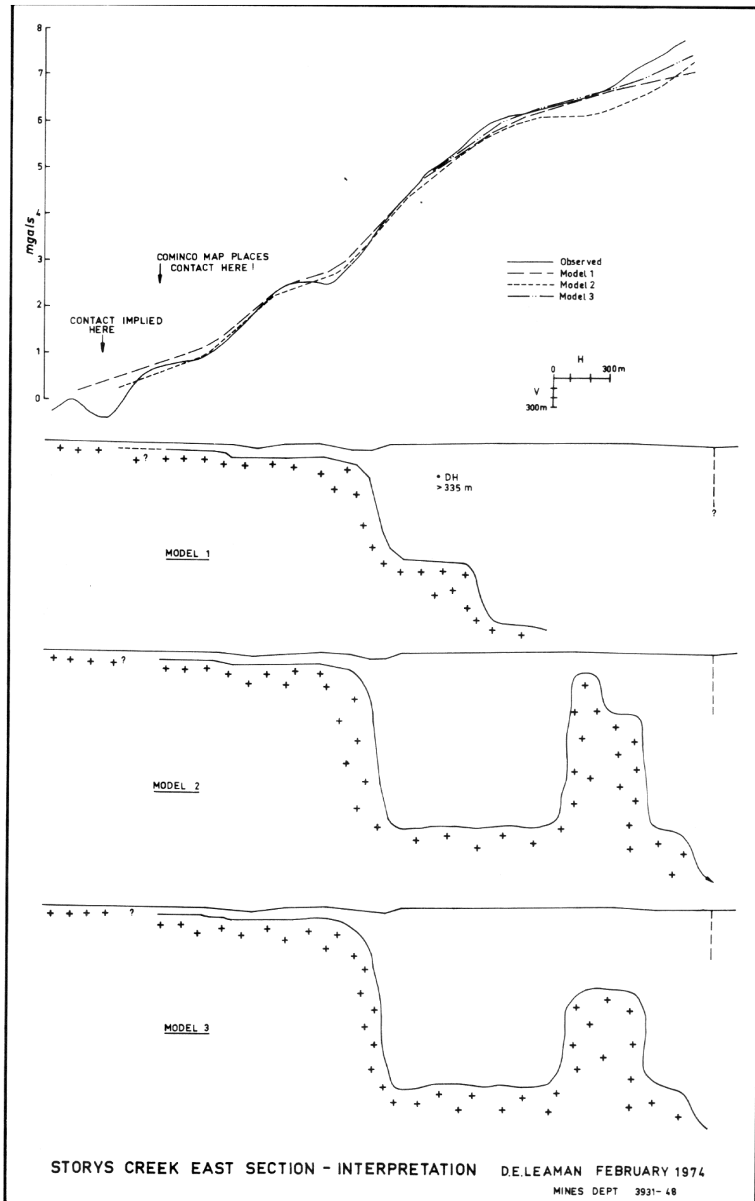
Figure A4.3 – Storeys Creek East Section: Proposed subsurface structure models derived from gravity data over Storeys Creek East Section (from Leaman Report, Figure 19, TR19_55_81)
