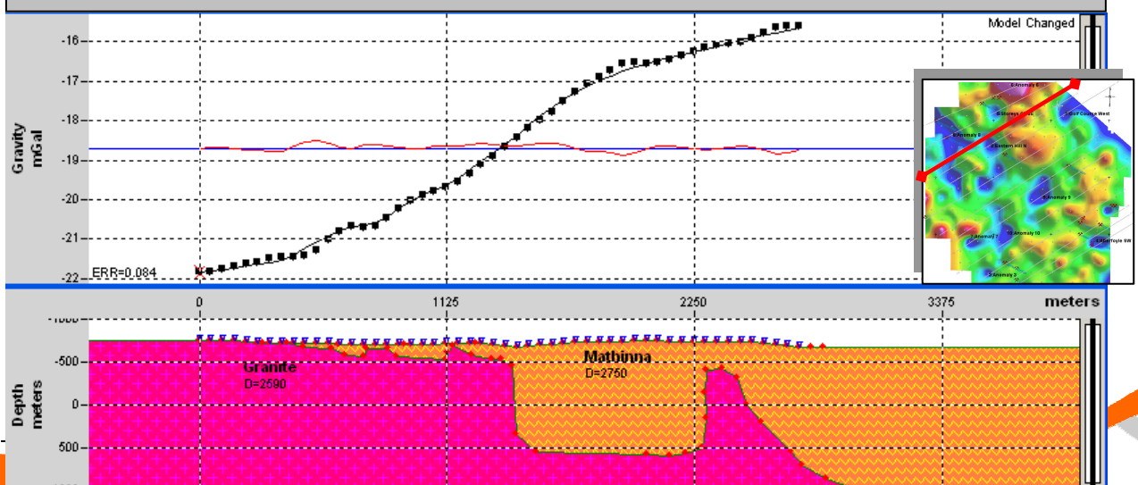
Figure 3.6: Line 2 – Anomaly 5 (Storeys Creek South section 2)
