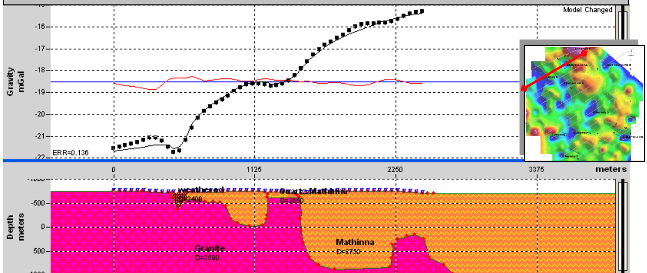
Figure 3.5: Line 1 – Anomaly 5 (Storeys Creek South section)
