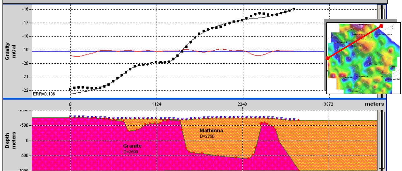
Figure 3.7: Line 3 – Anomaly 1 (Golf Course W – north section) and Anomaly 2 (Eastern Hill)
