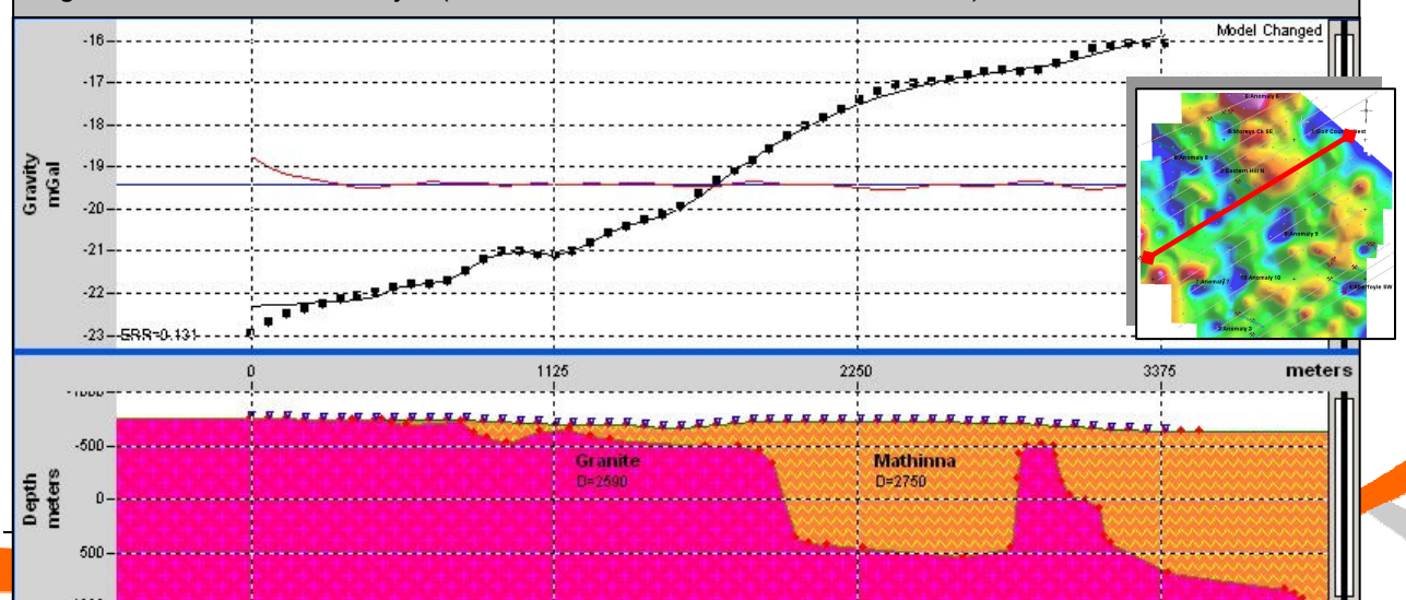
Figure 3.9: Line 5 – Anomaly 1 (Golf Course West – south model section)
