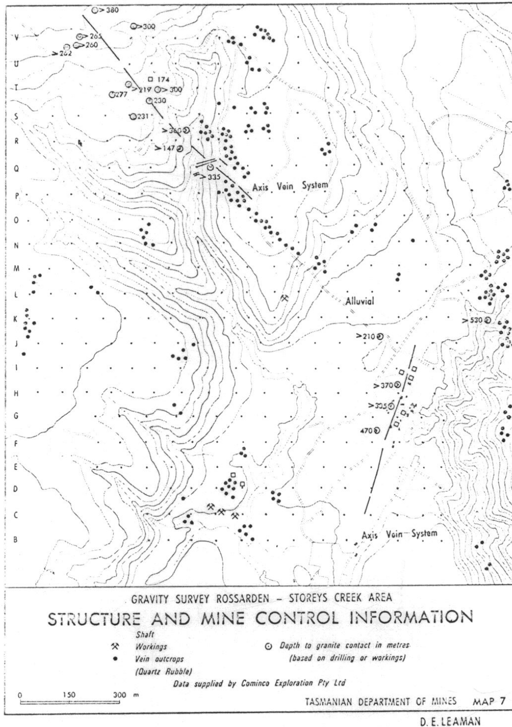
Figure A4.4 – Structure and mine control information for the Rossarden – Storeys Creek Area (MRT report, Map 7, UR1974_14)
