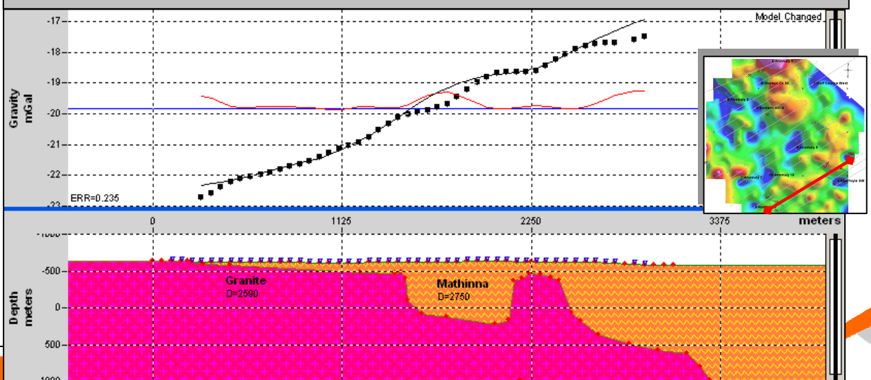
Figure 3.15: Line 12 – Anomaly 4 (Aberfoyle North section)
