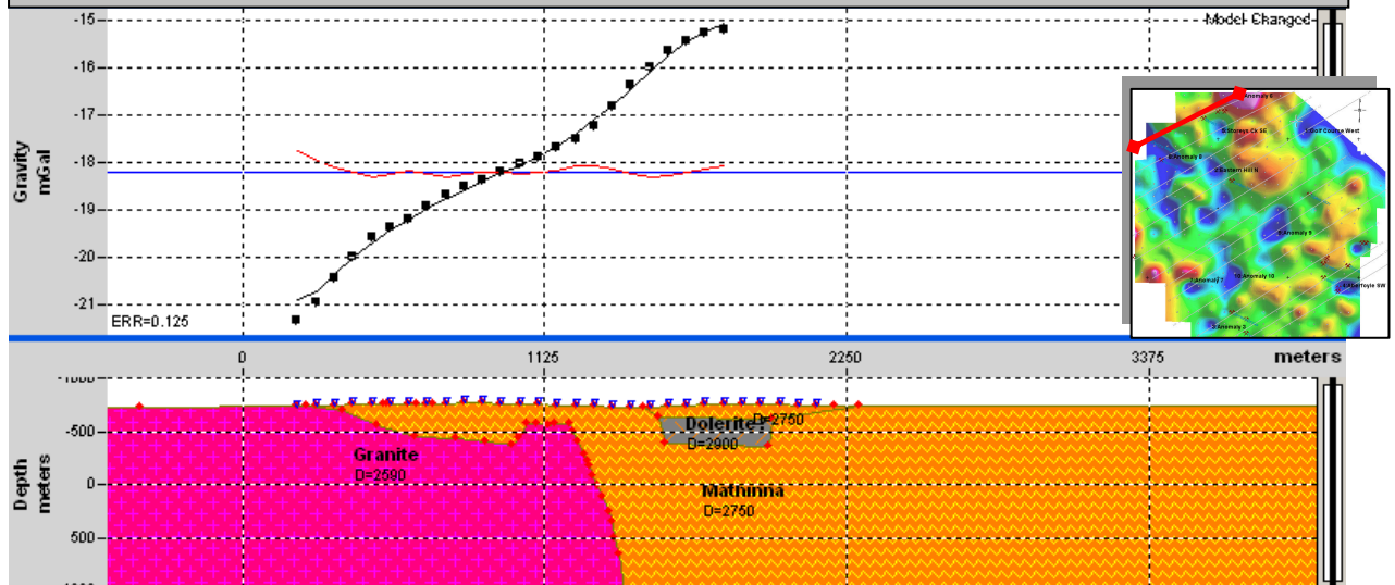
Figure 3.4: Line 0 – Anomaly 5 (Storeys Creek control section) and Anomaly 6
