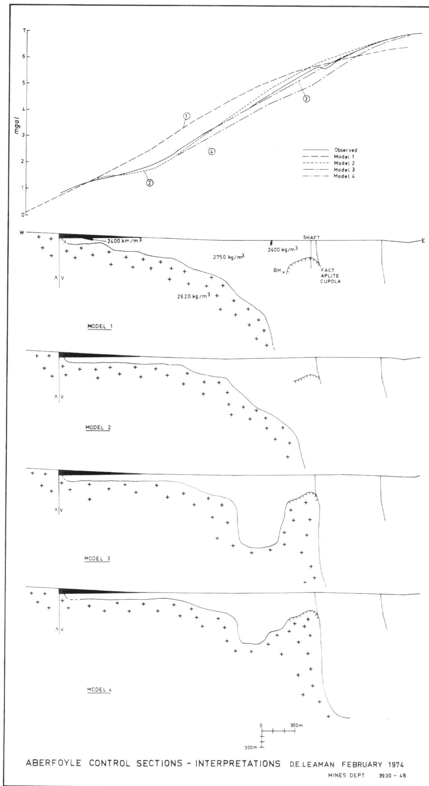
Figure A4.1 – Aberfoyle Control Section: Proposed subsurface structure models derived from gravity data over Aberfoyle Mine (reproduced from Report TR19_55_81, Figure 17)
