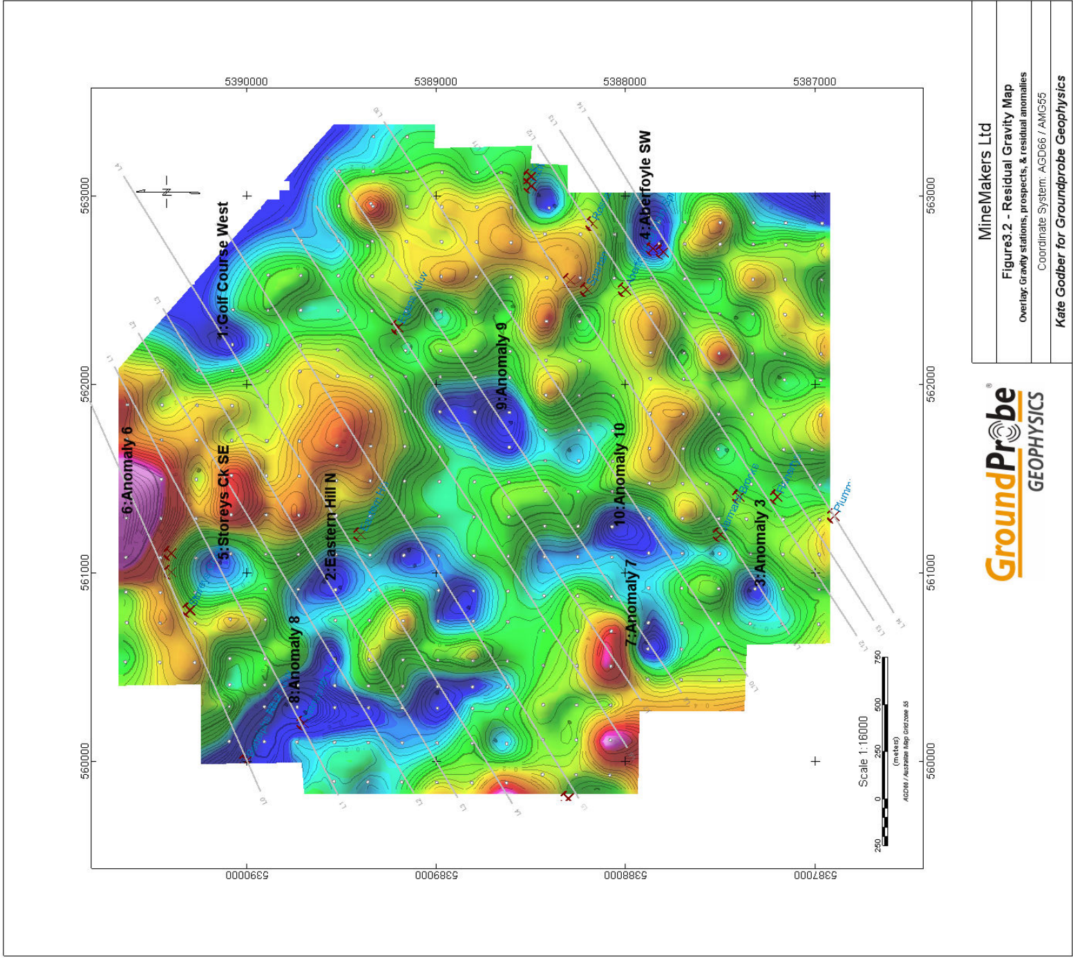
Figure 3-2: Residual gravity map showing identified residual anomalies and modelling sections.
