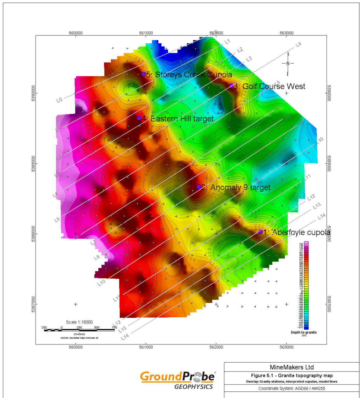
Figure 5-1: Map of the interpreted granite topography showing the major cupola targets, gravity stations, and modelling sections from which the granite topography grid is derived.
