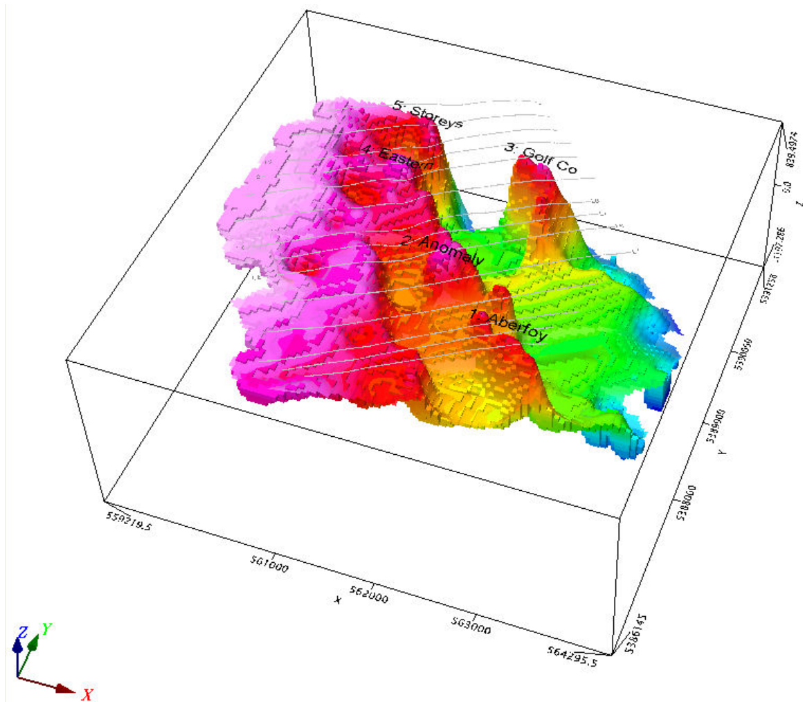
Figure 5-2: 3D map of the interpreted granite topography showing identified cupolas.
