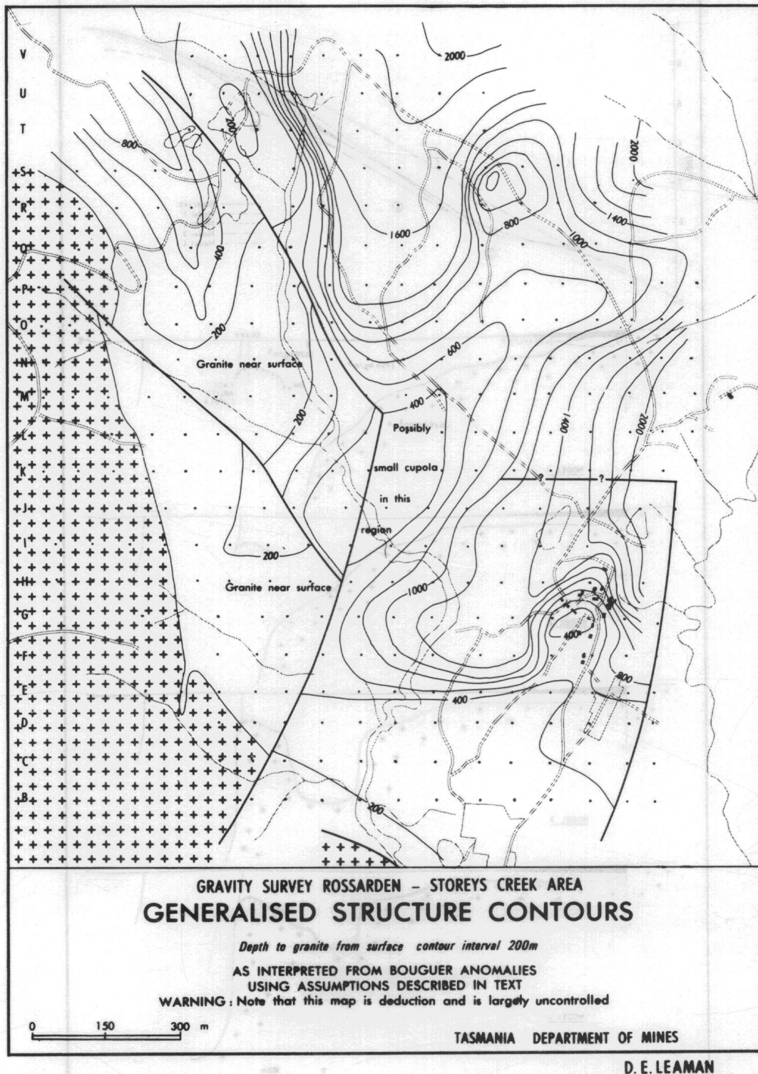
Figure A4.3 – Generalised structure contours proposed for the Rossarden – Storeys Creek Area (from Leaman Report, Figure 16, TR19_55_81)
