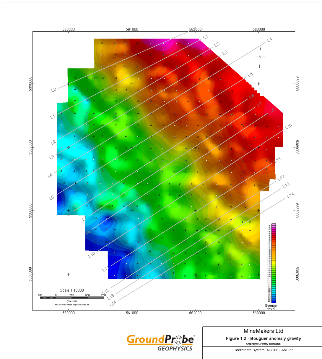
Figure 1-2 – Aberfoyle - Storeys Bouguer anomaly map showing model sections.
