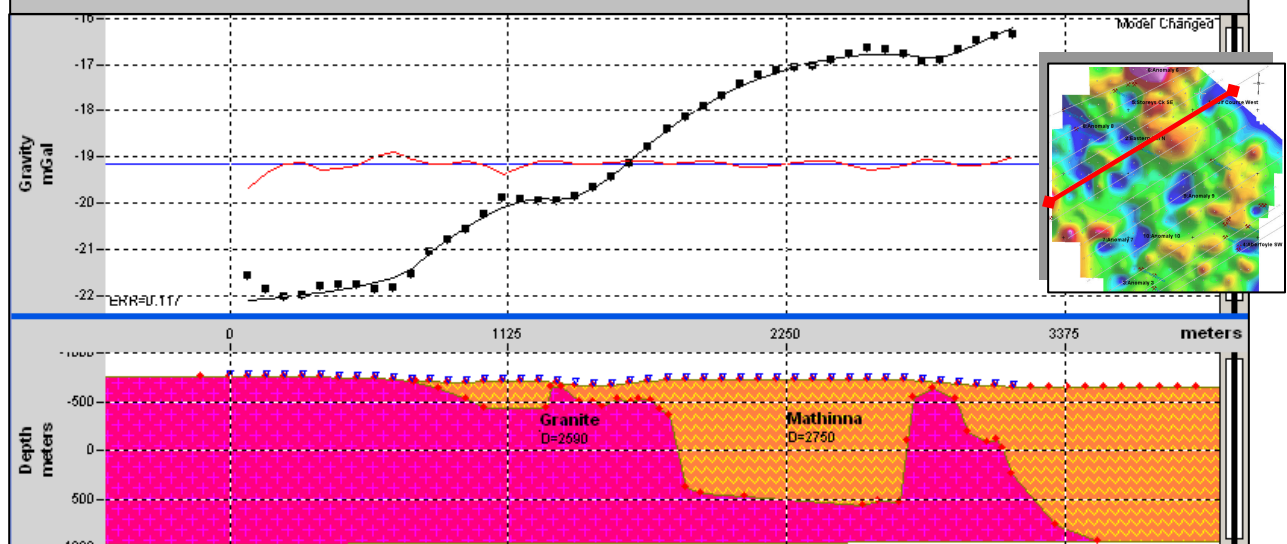
Figure 3.8: Line 4 – Anomaly 1 (Golf Course West) and Anomaly 2 (Eastern Hill-south section)
