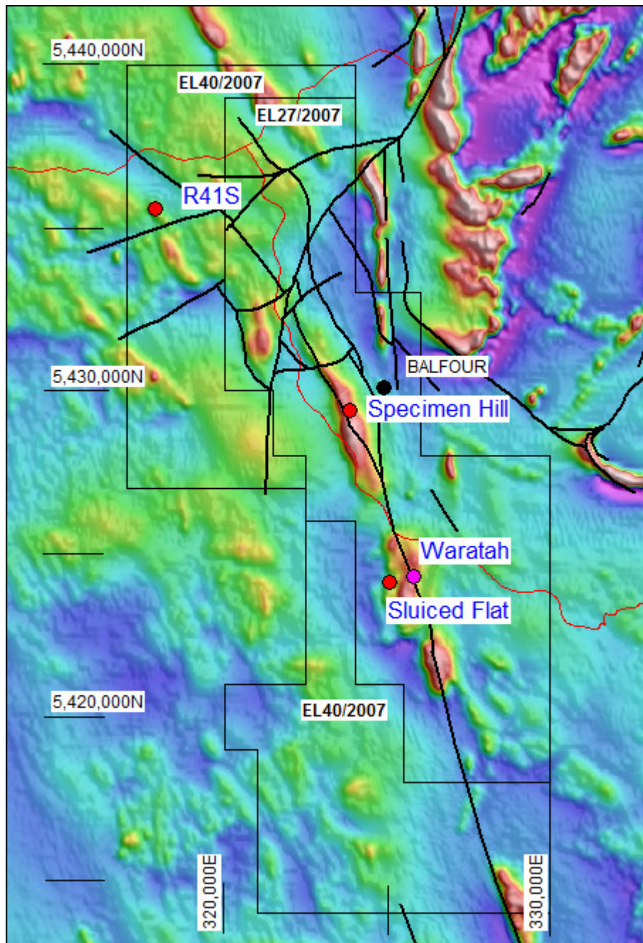
Figure 1. Balfour Tenement Location plan and Total Magnetic Intensity Image.
