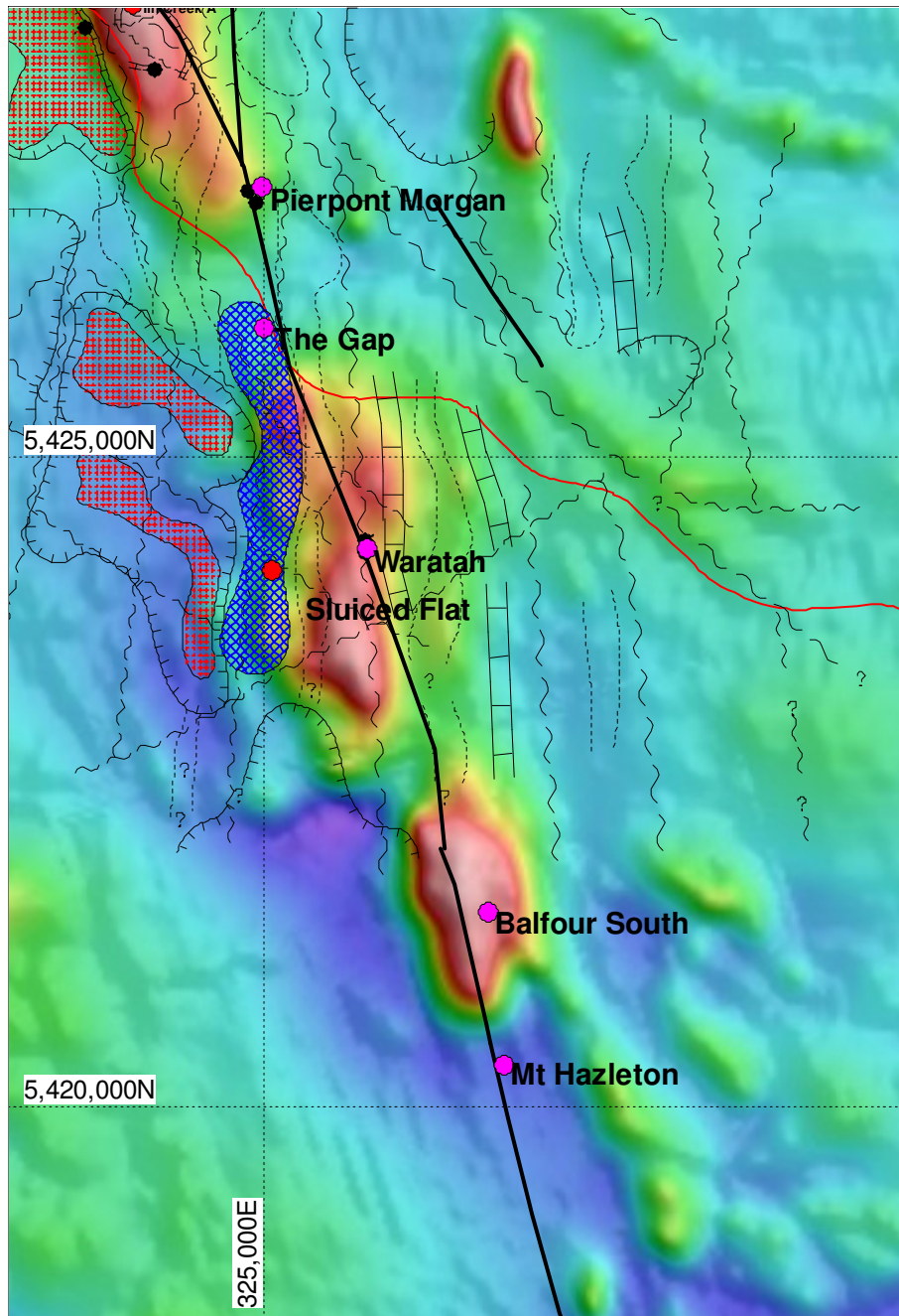
Figure 7. South Balfour-Sluiced Flat, TMI and mineralised prospects (purple = copper, red = tin) and diamond drill holes (black).
