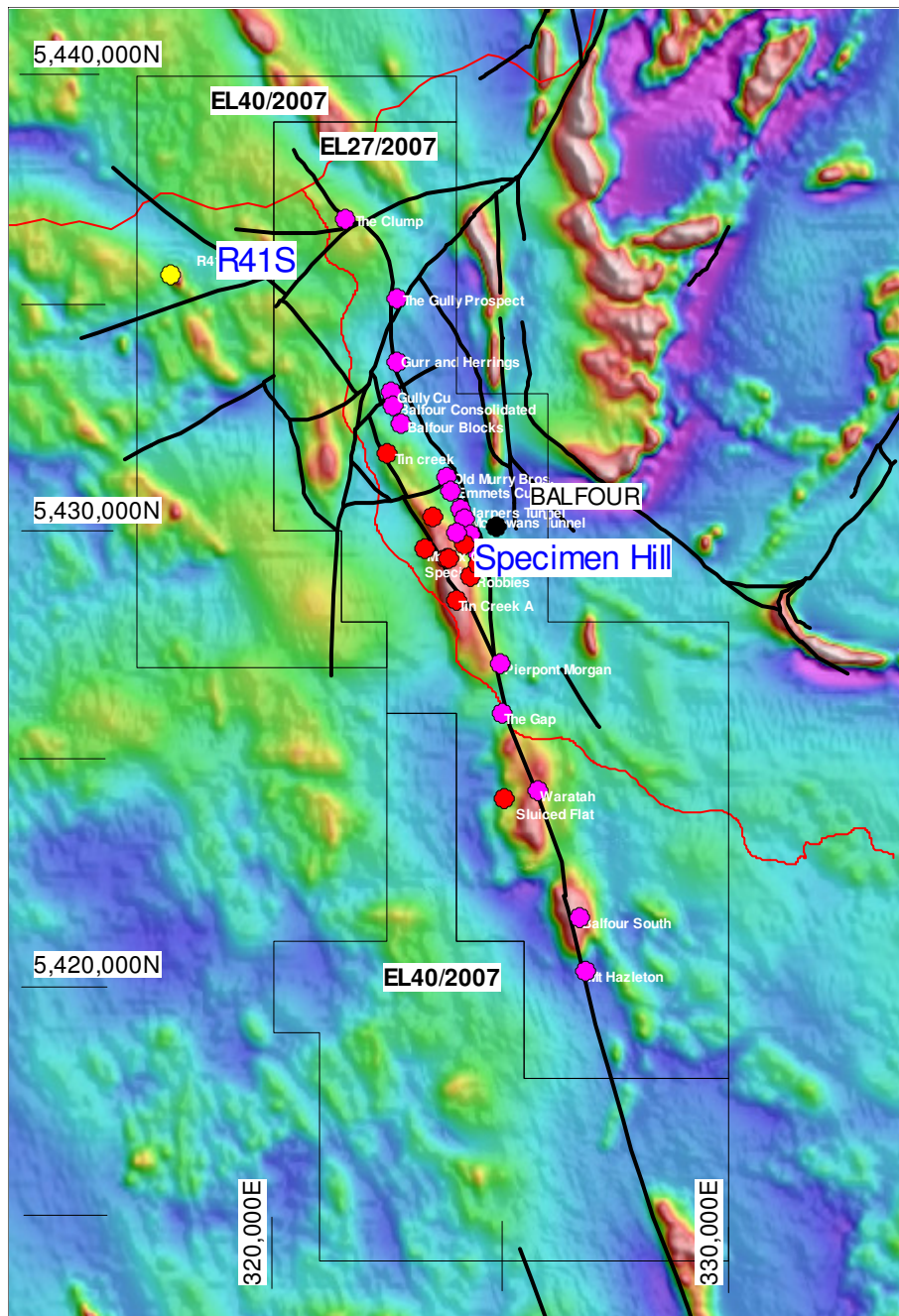
Figure 1. Balfour tenement location plan, total magnetic intensity image and known mineral deposits.
