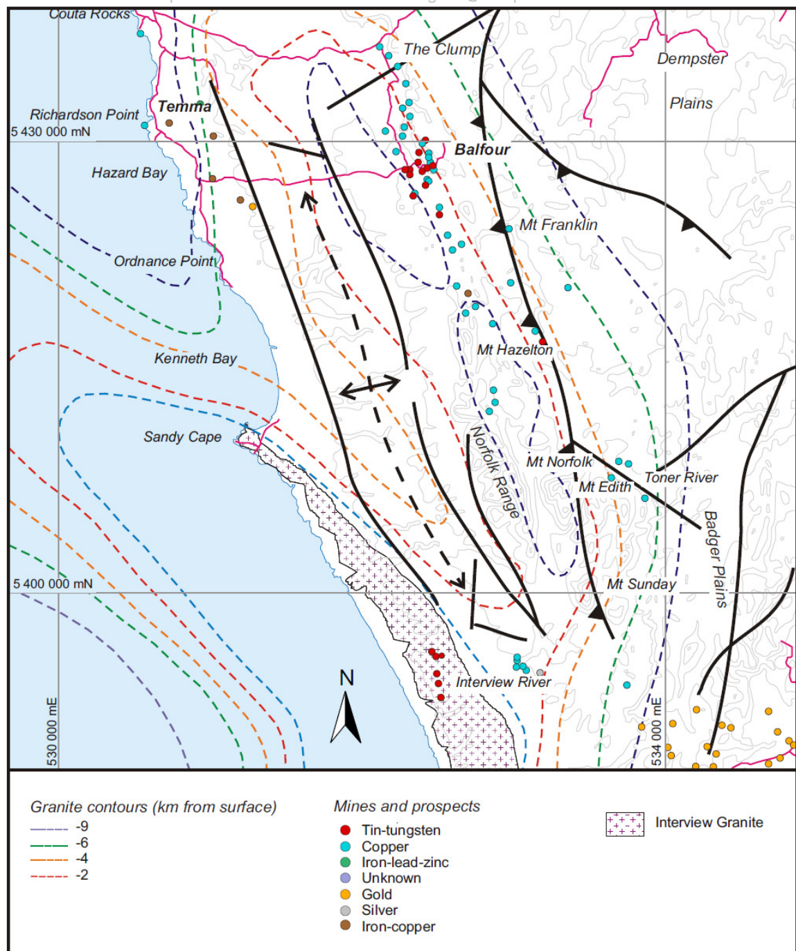
Figure 3. Granite Contours, Structure and Mineral deposits of the Balfour District, (Bottrill and Taheri, 2003).
