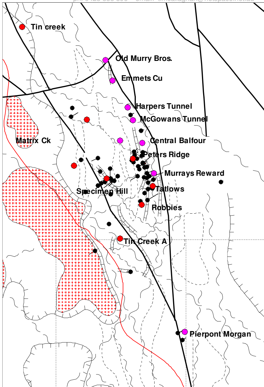
Figure 5. Balfour-Specimen Hill gravity interpretation (red hatched = gravity low), mineralised prospects (purple = copper, red = tin) and diamond drill holes (black).
