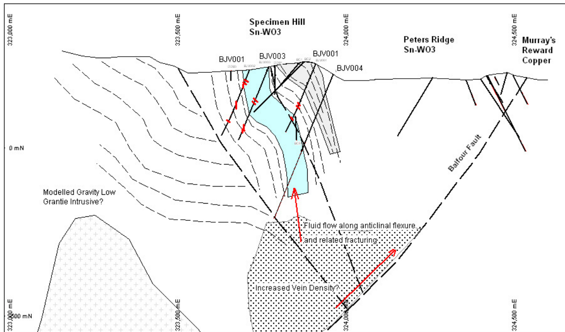
Figure 4. Section 5429350, Drill hole locations and Geology Interpretation. The tin mineralisation probably represents the distal margins of a deeper granite related mineralizing system. The Balfour copper mineralisation has been demonstrated to be due to Devonian granitic/meteoric fluids and is therefore likely to be part of the same mineralizing event.
