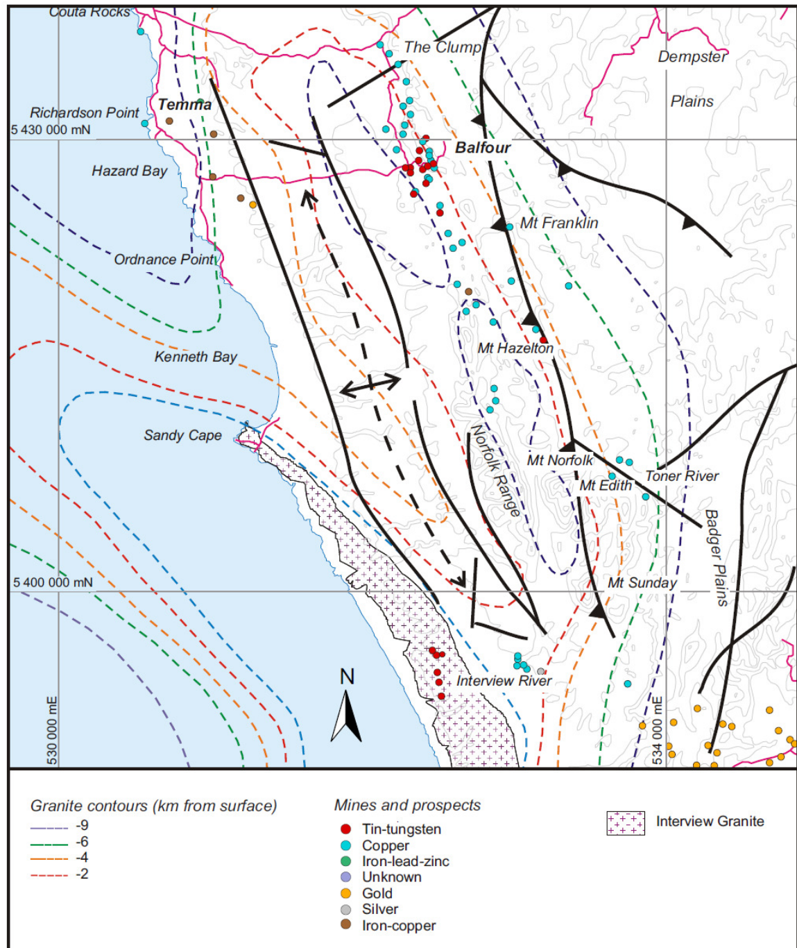
Figure 3. Granite Contours, Structure and Mineral deposits of the Balfour District, (Bottrill and Taheri, 2003).
