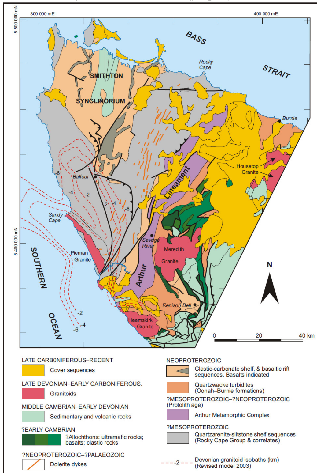
Figure 2. Regional Geology Northwest Tasmania (Everard et al , 2007).
