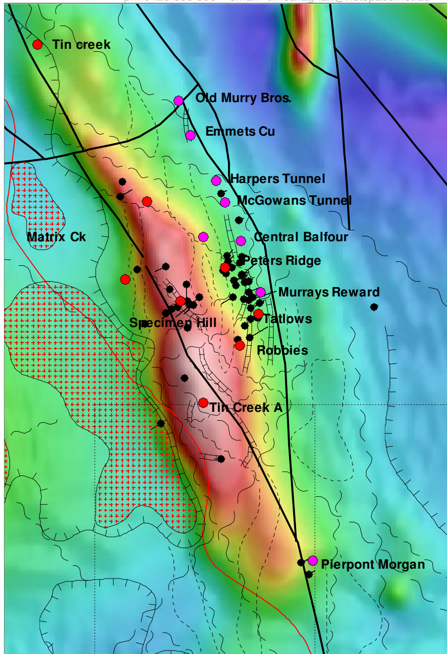
Figure 6. Balfour-Specimen Hill TMI, mineralised prospects (purple = copper, red = tin) and diamond drill holes (black).
