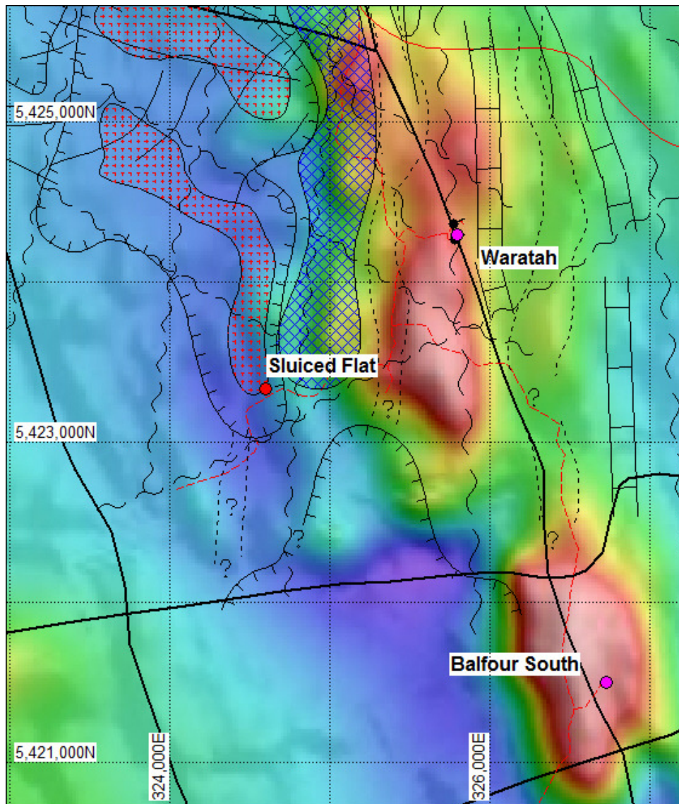
Figure 5. South Balfour-Waratah, TMI and mineralised prospects, gravity interpretation (purple = copper, red = tin) and diamond drill holes (black). Blue Shade = Gravity Low, Red Shade = Gravity High.
