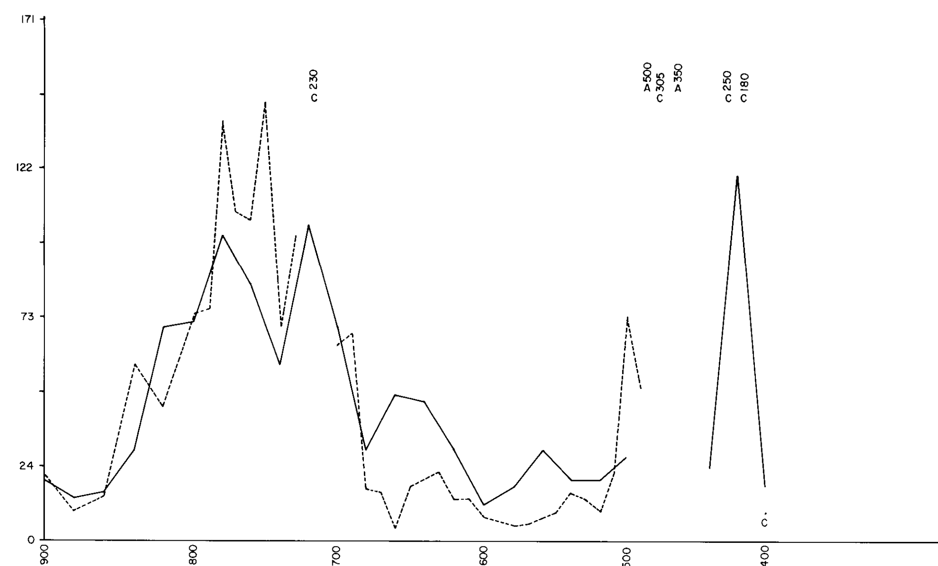
LEAD
