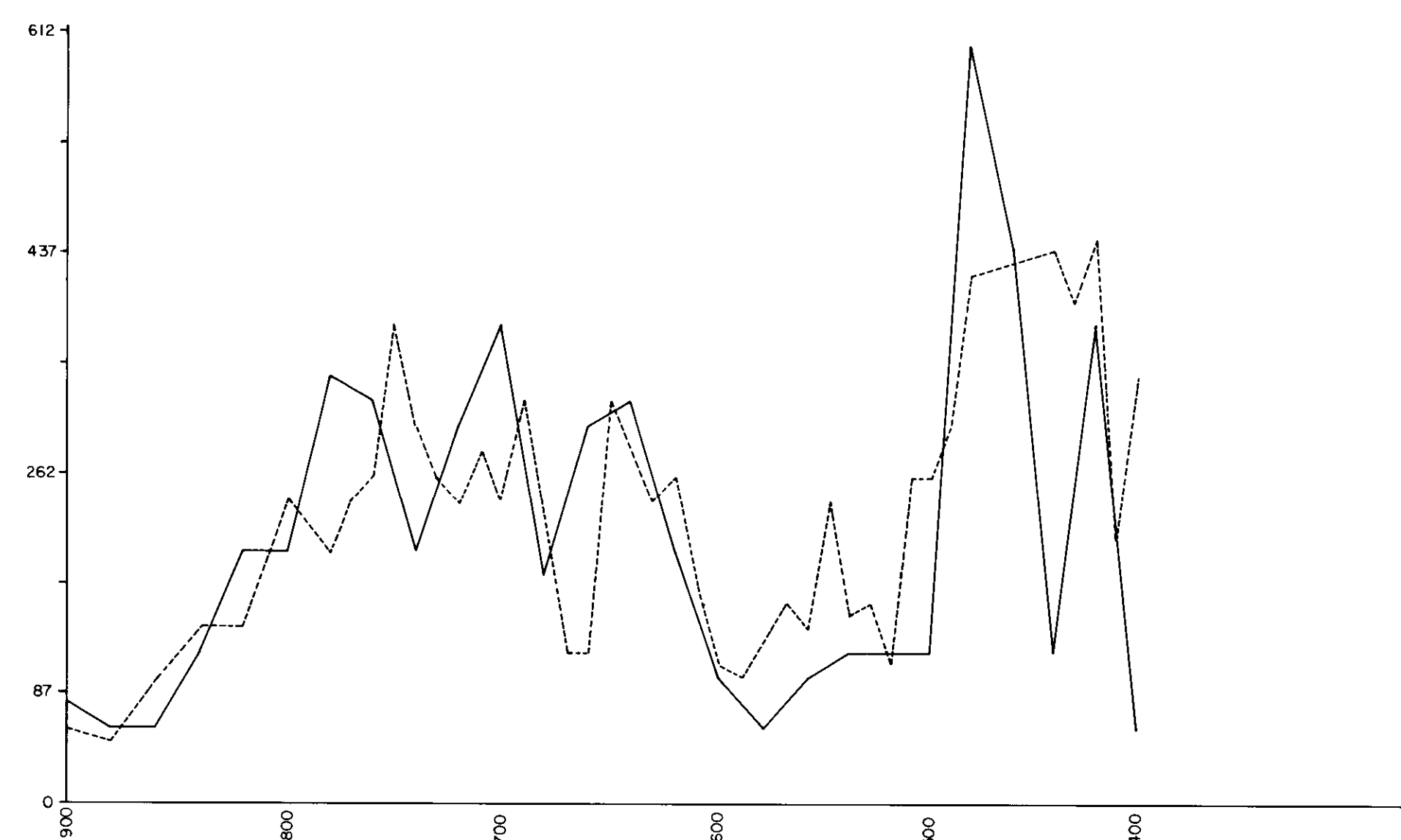
BARIUM
