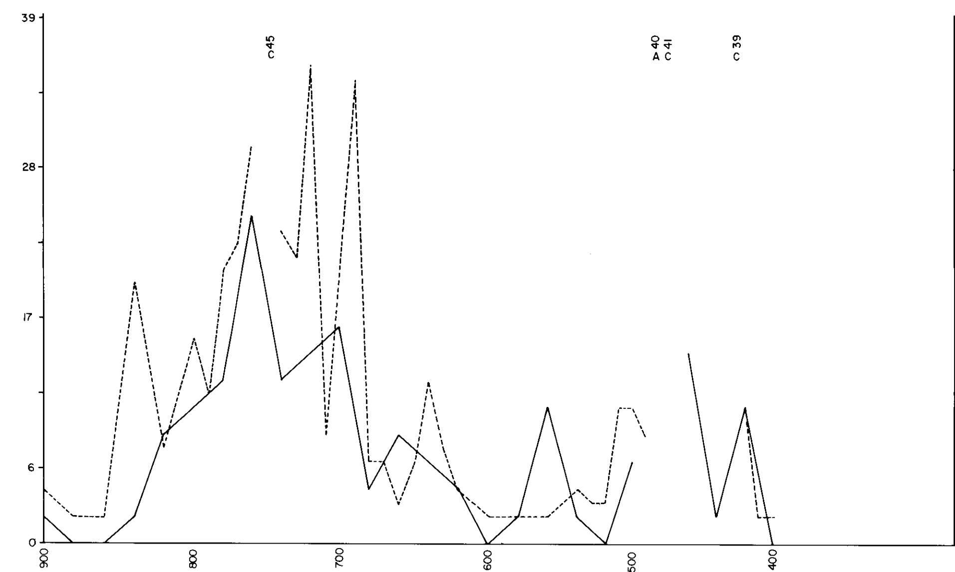
COPPER
