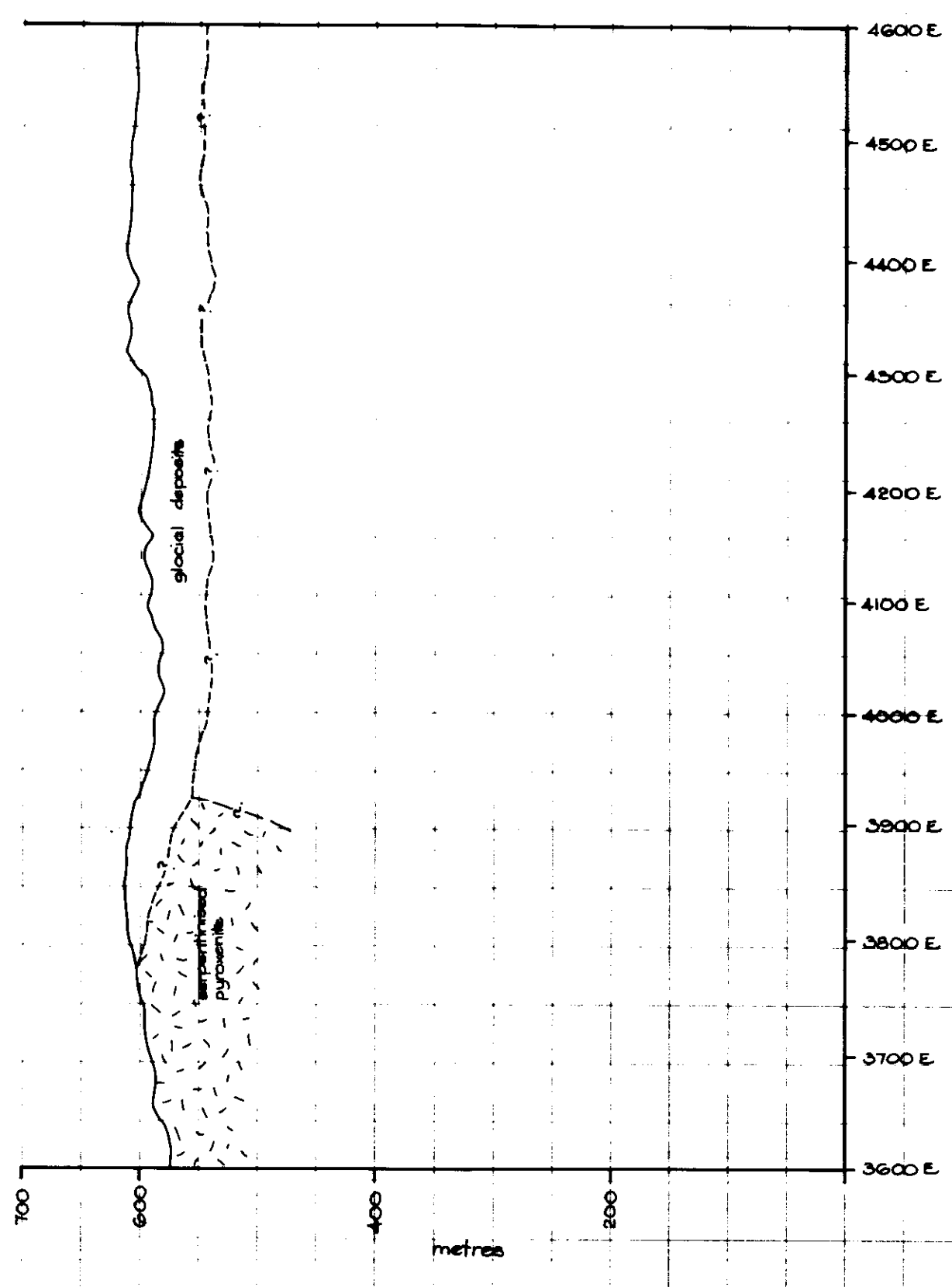
GEOLOGY LINE 3000N
