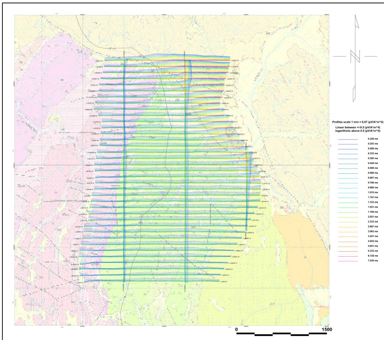
Moores Block - VTEM dB/dt Z Component Profiles, Time Gates 0.220 to 7.036 ms
