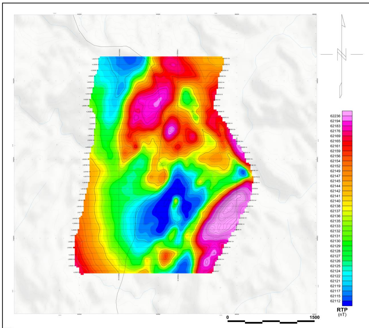
Moores Block - Reduced to Pole of TMI (RTP)
