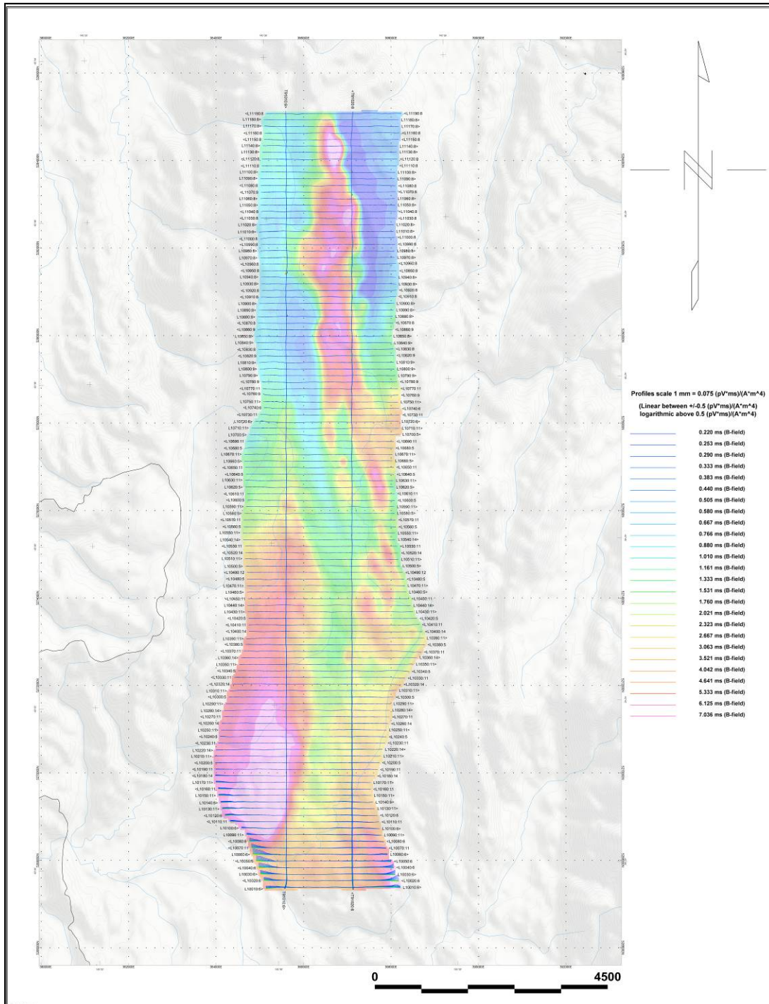
Daguiar Block - VTEM B-Field Z Component Profiles, Time Gates 0.220 to 7.036 ms
