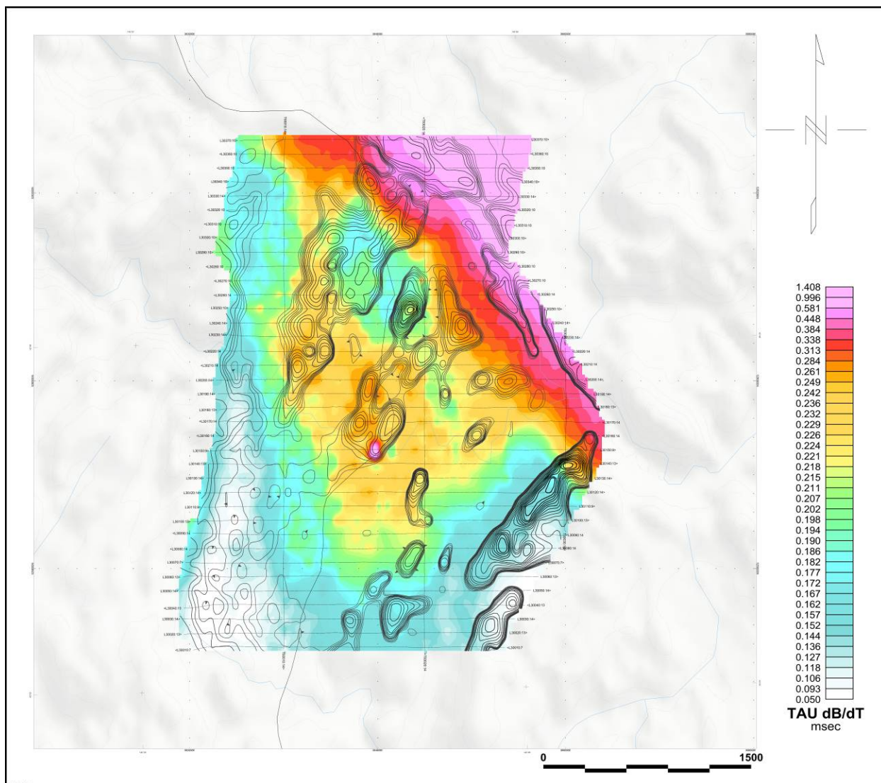
Moores Block - dB/dT Calculated Time Constant (Tau) with contours of anomaly areas of the Calculated Vertical Derivative of TMI
