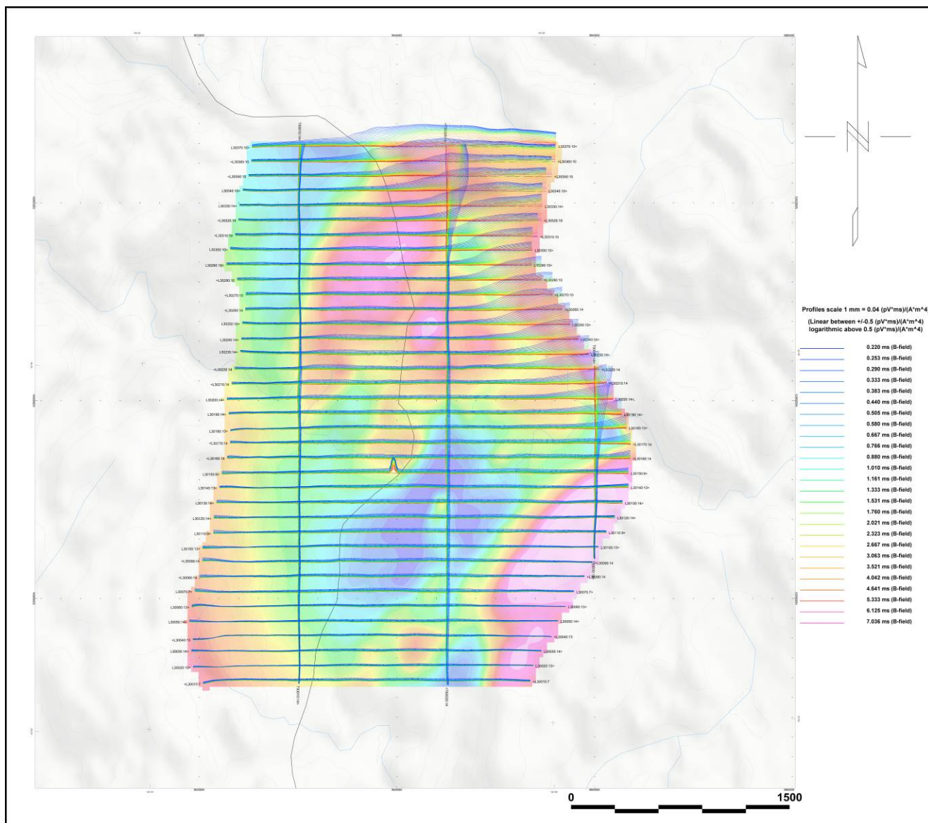
Moores Block - VTEM B-Field Z Component Profiles, Time Gates 0.220 to 7.036 ms
