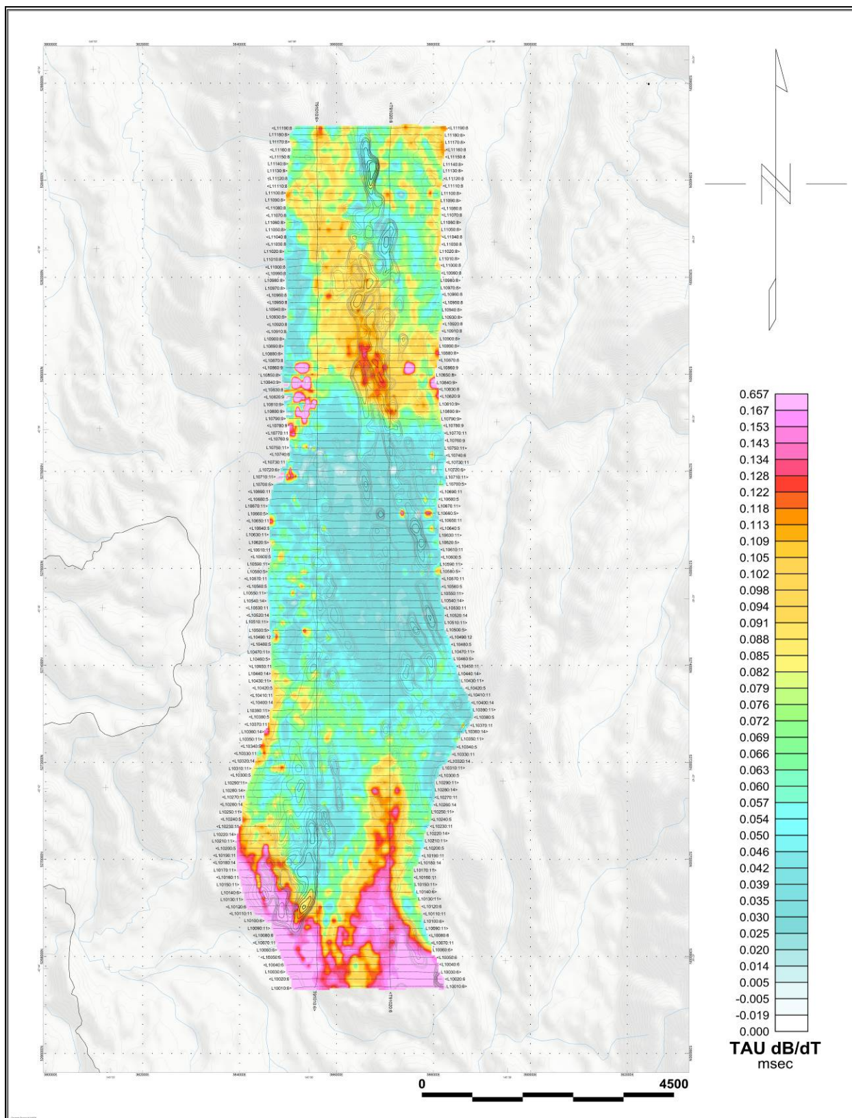
Daguar Block - dB/dt Calculated Time Constant (Tau) with contours of anomaly areas of the Calculated Vertical Derivative of TMI
