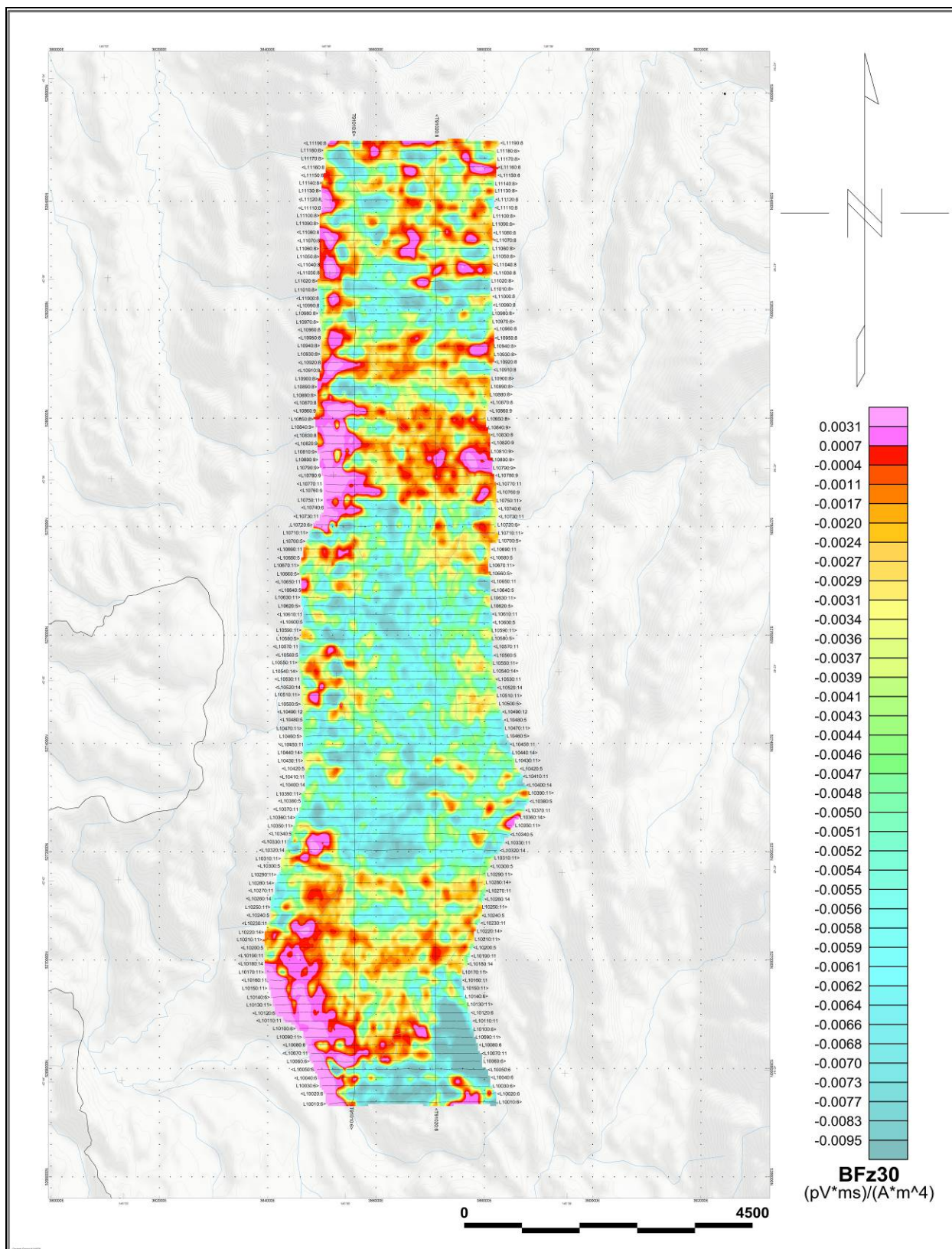
Daguiar Block - VTEM B-Field Z Component Channel 30, Time Gate 0.880 ms
