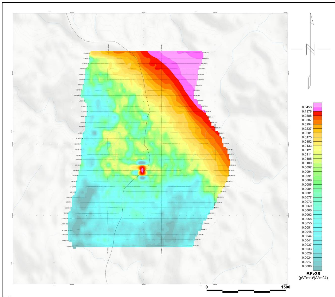
Moores Block - VTEM B-Field Z Component Channel 36, Time Gate 2.021 ms
