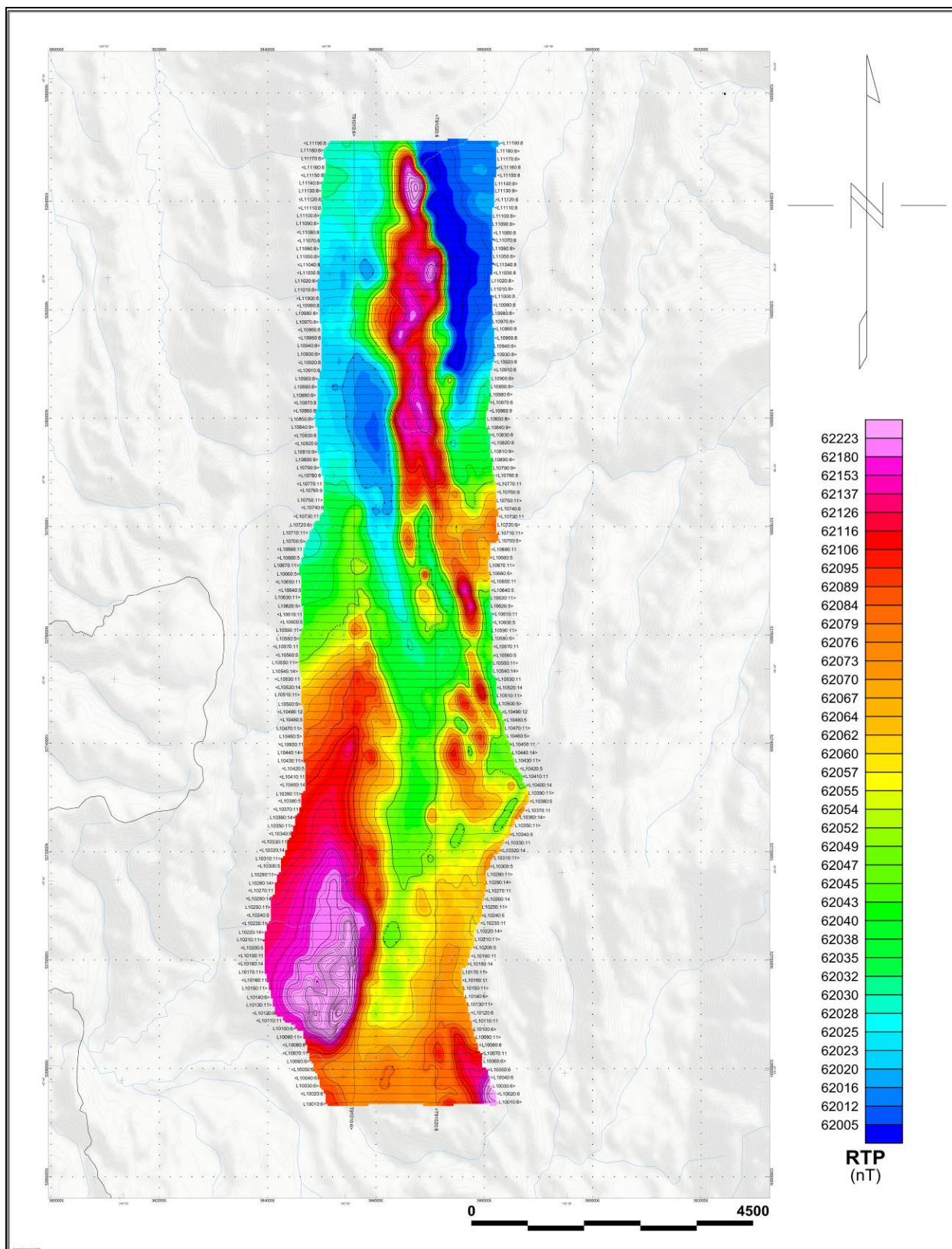
Daguiar Block - Reduced to Pole of TMI (RTP)
