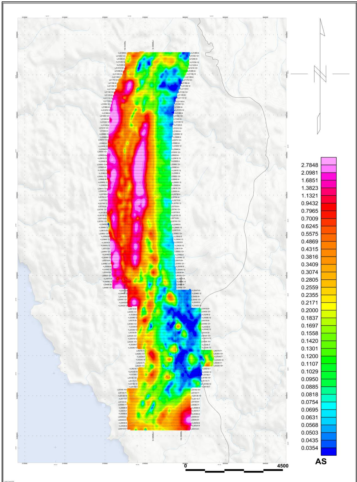
WartHill Block – Analytic Signal (AS)
