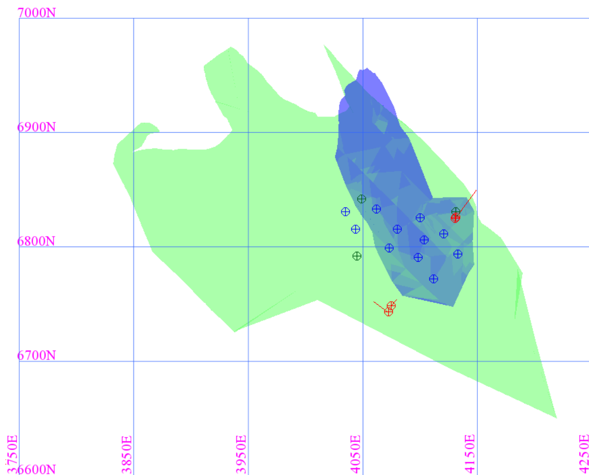
Figure 8. Comparison of previous wireframe (green) and current mineralised wireframe (blue) (plan view). Drill collars shown (1996 programme=green, 2005 programme=red, 2011 programme=blue collars). Note position of the two 2005 and one 1996 drill holes outside the 2013 wireframe. The AMC modelled wireframe passes below these holes.
