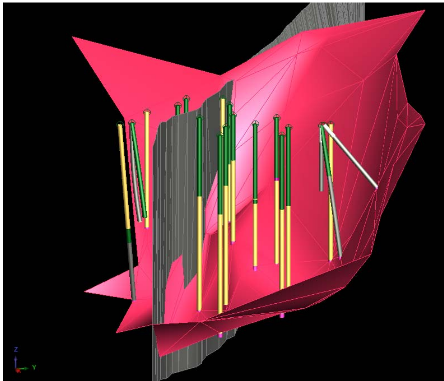
Figure 4. Modelled Pioneer Beds surface (Pink) and King Lyell Fault extension (grey) looking west. Drill holes displayed (Pioneer Beds = pink, Gordon Group clays = tan, Undifferentiated clays = dark grey, Alluvium and tailings = light grey, Recent fill = green).
