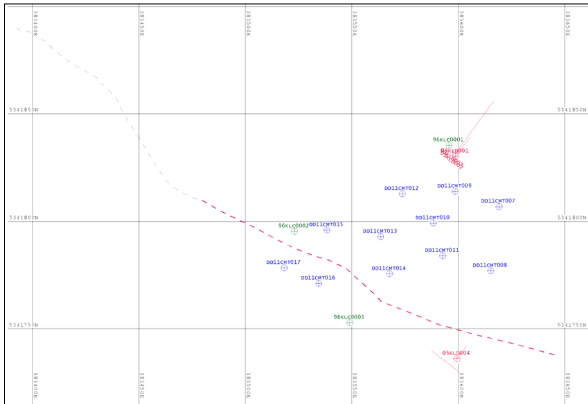
Figure 3. King Lyell Fault as mapped (grey dashed) and King Lyell Fault extension (red dashed). 1996 programme=green, 2005 programme=red, 2011 programme=blue collars.
