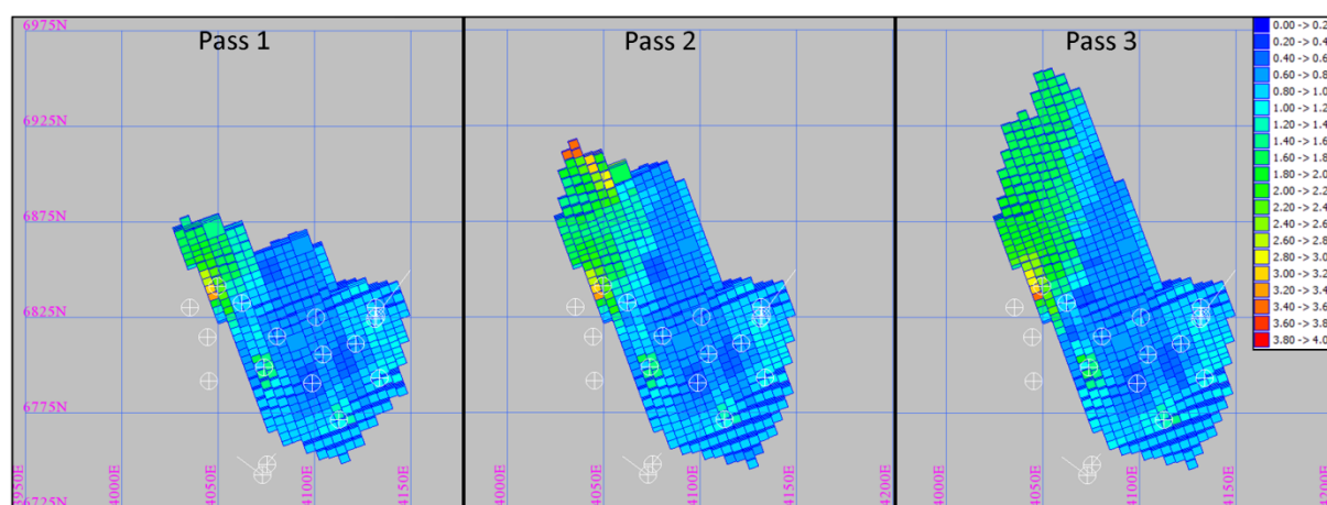
Figure 6. Plan view of results of Pass 1, 2 and 3 search parameters. Drill-hole collars in white. Inset - copper grade legend.
