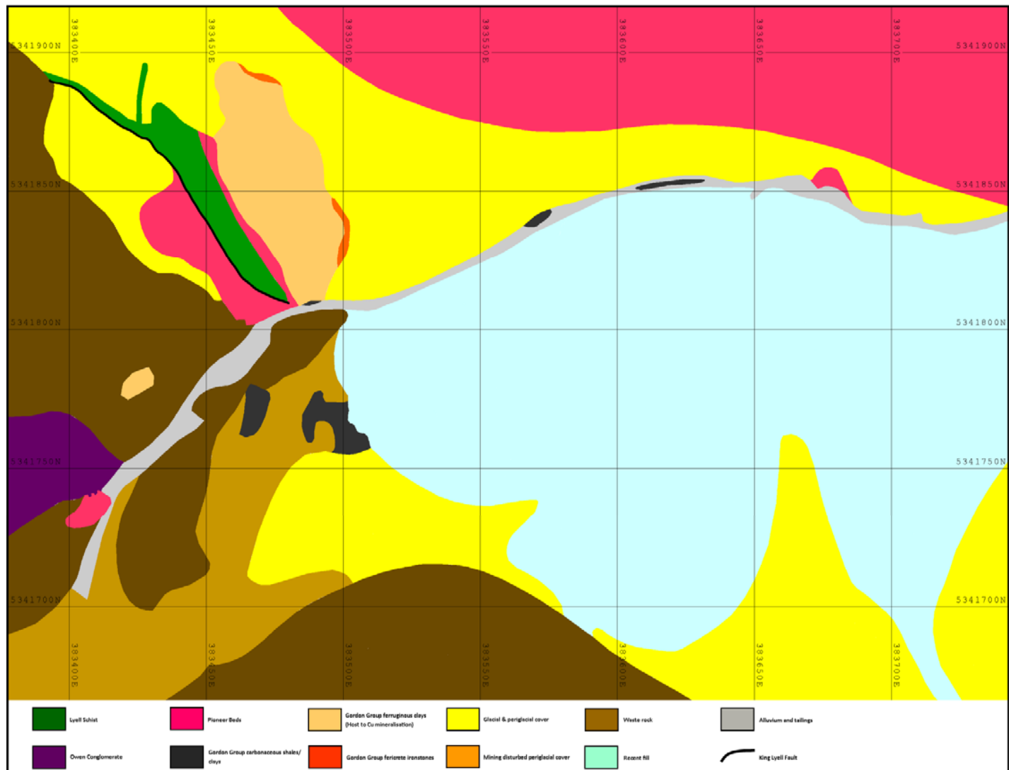
Figure 2. Surface geology map of the King Lyell area.
