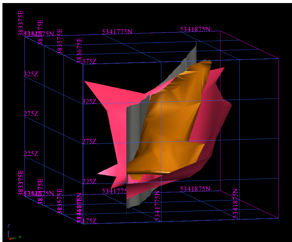
Figure 5. Modelled mineralised wireframe (brown), constrained by Pioneer Beds (pink) and King Lyell Fault extension (grey).
