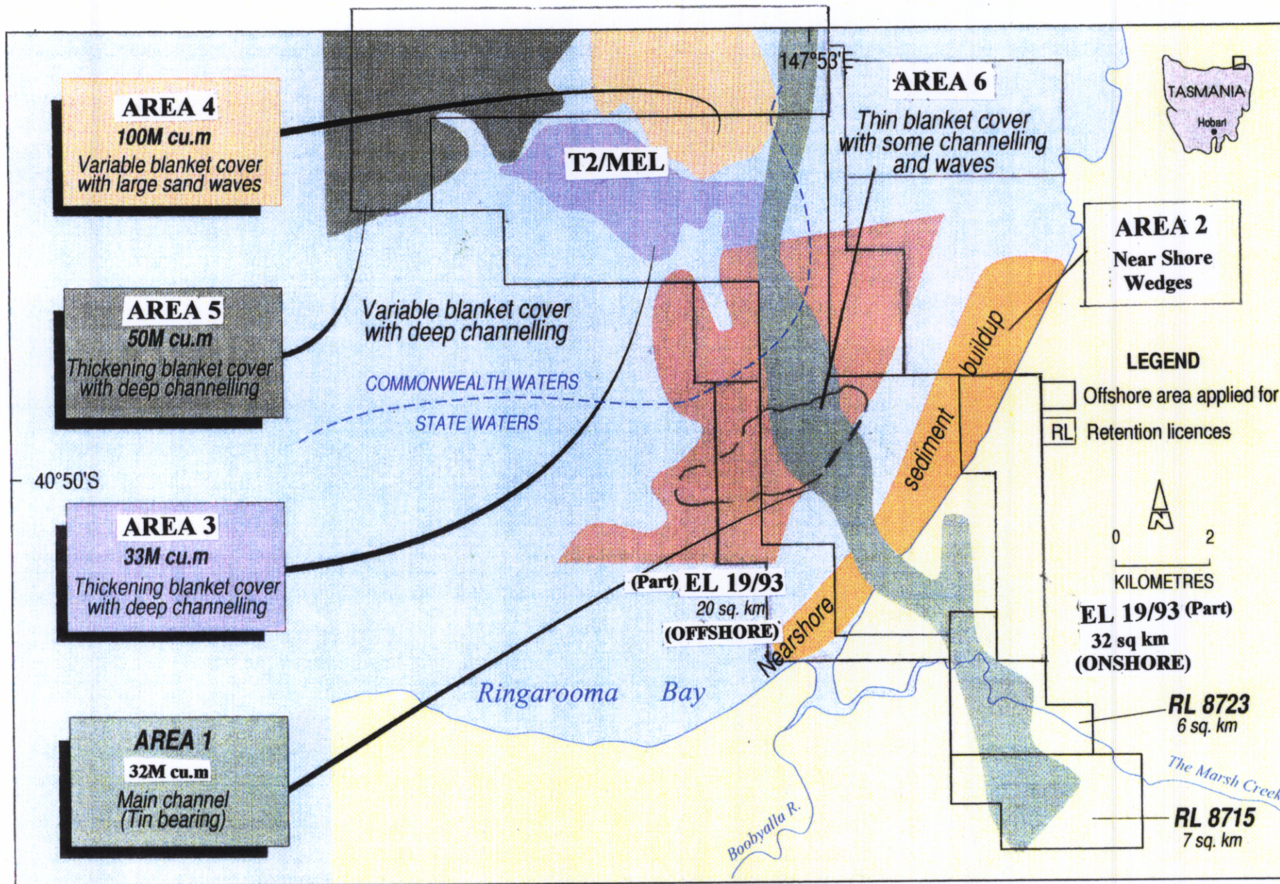
THE RINGAROOMA ALLUVIAL TIN PROPERTY – TENEMENT PLAN AND POTENTIAL TIN RESOURCES
