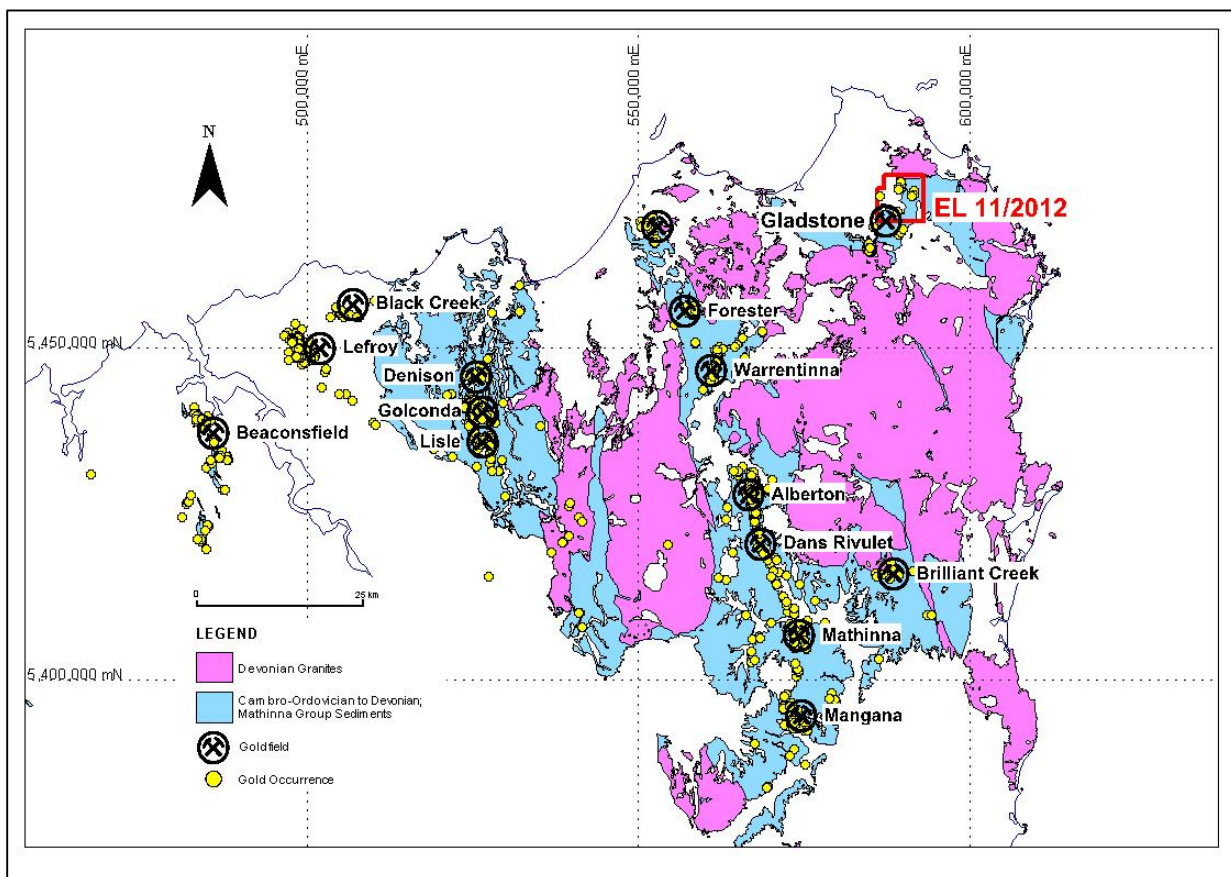
Figure 5. Map showing the goldfields of northeastern Tasmania with simplified Ordovician to Devonian geology.
