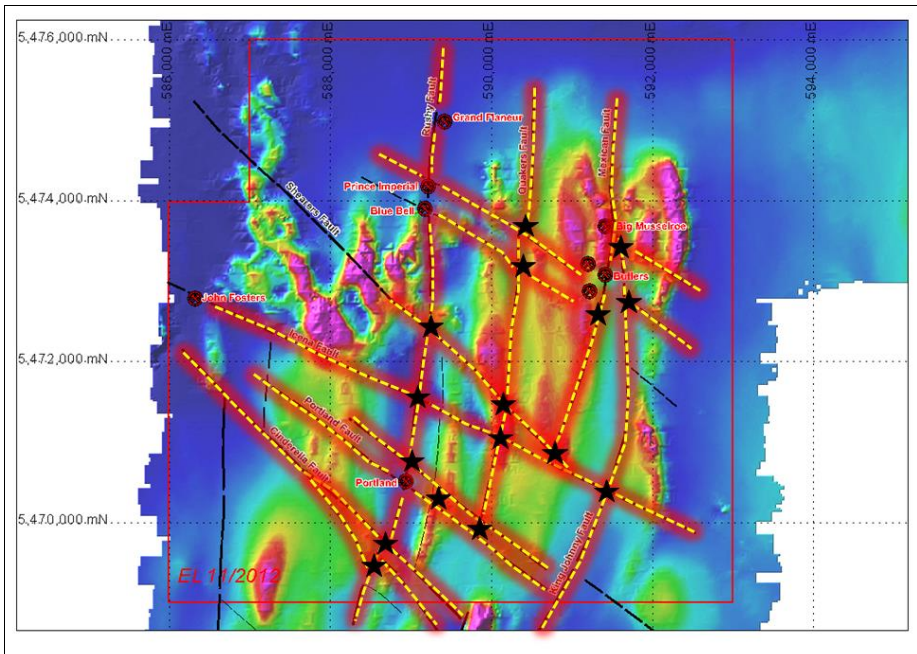
Figure 10. Map showing district-scale magnetics (TMI), historical gold mines, key structural trends and priority exploration targets (stars) at intersections of NNE- and NW-trending structures. Geophysics Data Source: 1987 Gladstone survey (MRT Survey ID: gladstone1987, Placeco, 125 m line spacing)
