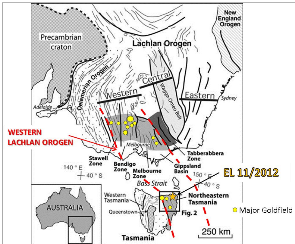
Figure 4. Map illustrating the inferred tectonic correlation between northeastern Tasmania and the western zone of the Lachlan Orogen in Victoria (modified after Bierlein et al, 2005).
