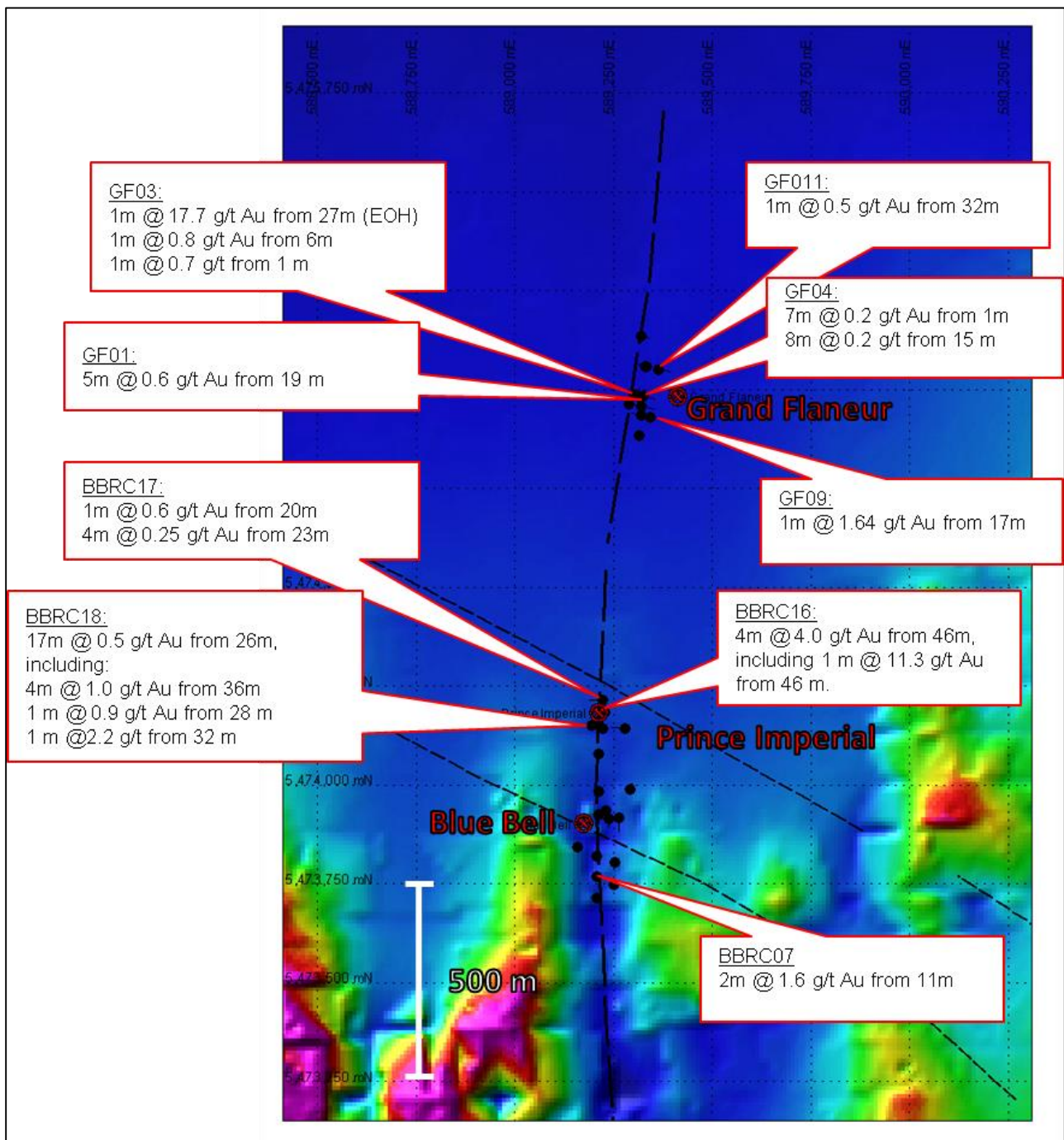
Figure 7. Significant RC drillhole intercepts in the Blue Bell-Prince Imperial-Grand Flaneur trend. Underlay image is of magnetics (TMI). Geophysics Data Source: 1987 Gladstone survey (MRT Survey ID: gladstone1987, Placeco, 125 m line spacing).
