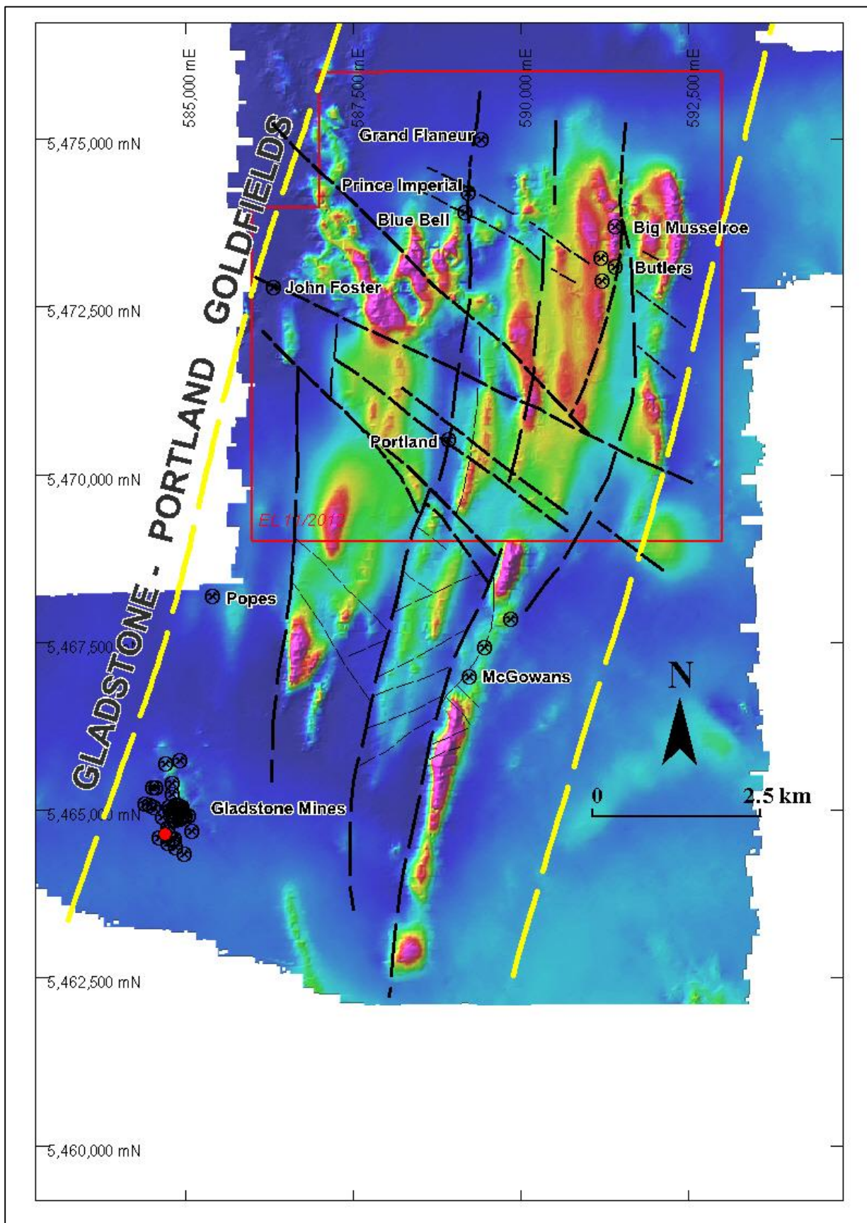
Figure 8. District-scale magnetics image (TMI) with historical gold mines and interpreted structures. Geophysics Data Source: 1987 Gladstone survey (MRT Survey ID: gladstone1987, Placeco, 125 m line spacing).
