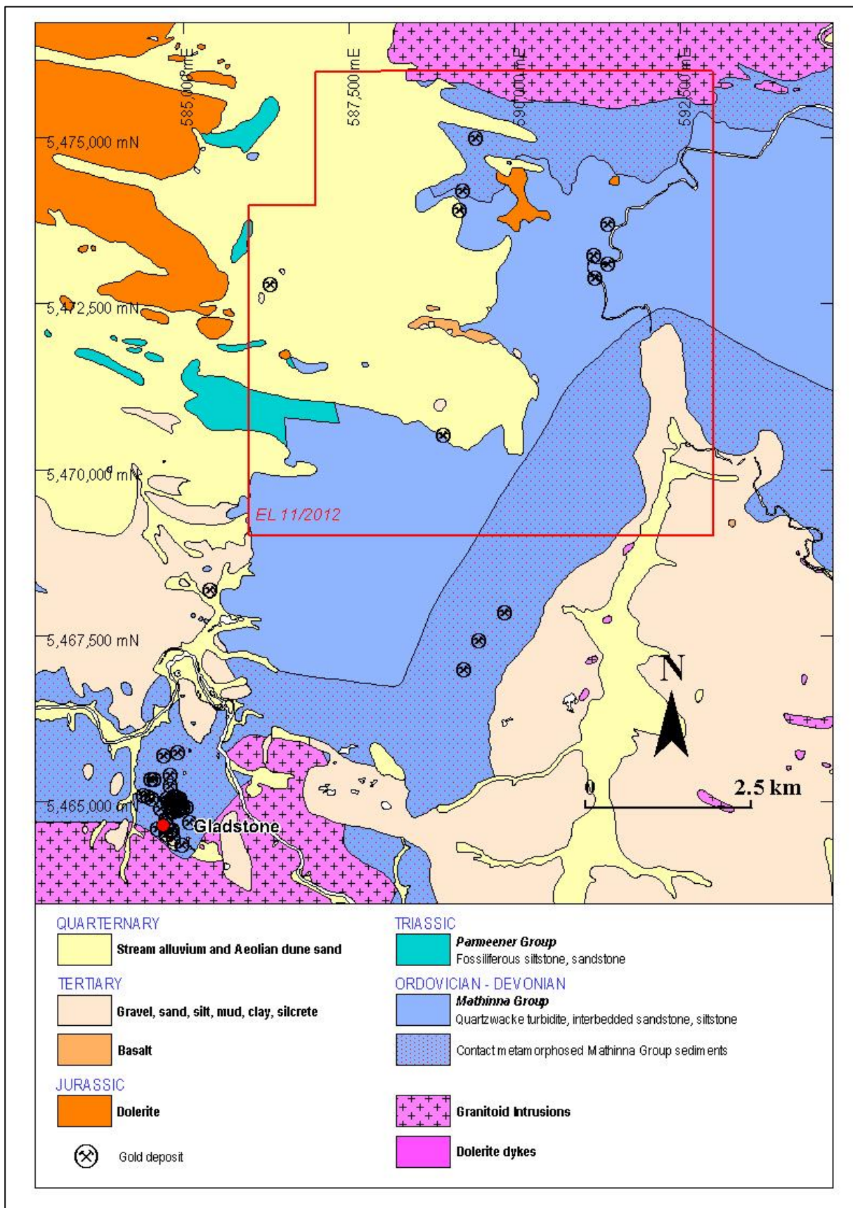
Figure 3. Geology map of the Gladstone-Portland goldfields area.
