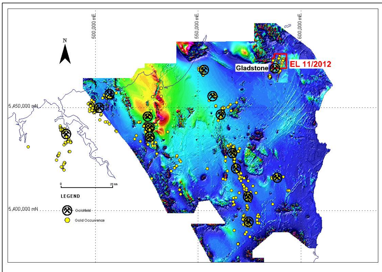
Figure 6. Regional magnetics image (TMI) and goldfields of northeastern Tasmania.
