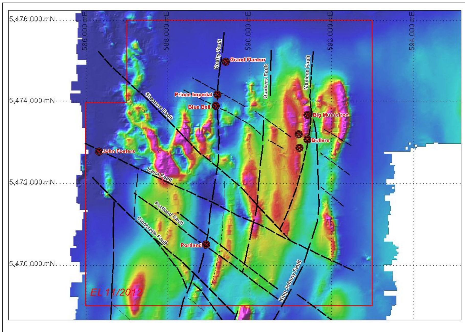
Figure 9. Map showing district-scale magnetics (TMI), historical gold mines and new structural interpretation over the Portland goldfields area. Geophysics Data Source: 1987 Gladstone survey (MRT Survey ID: gladstone1987, Placeco, 125 m line spacing).
