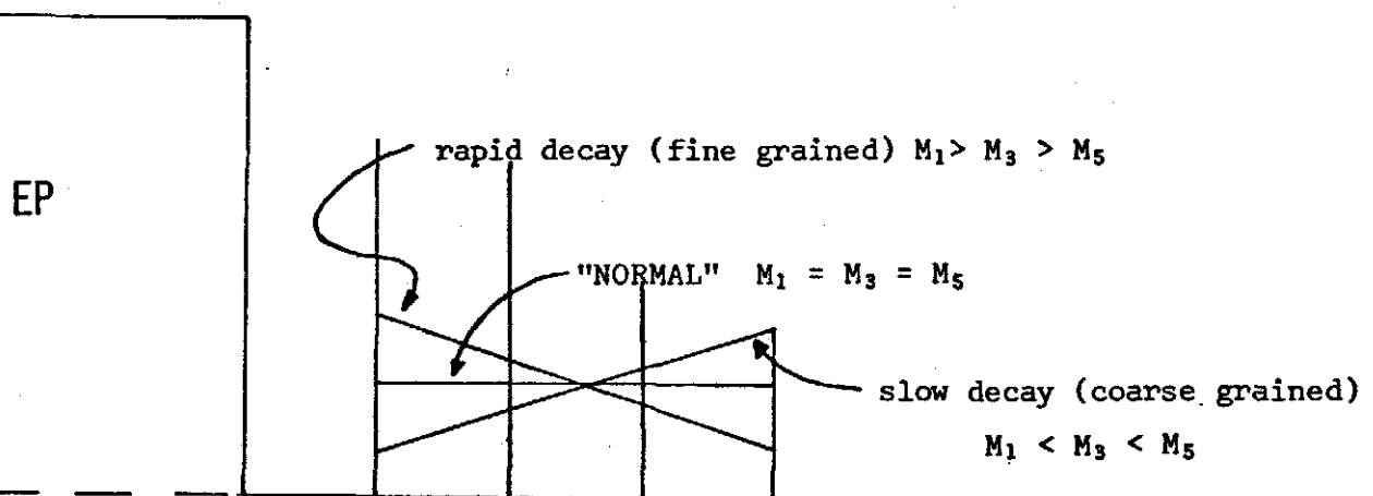
(B) DECAY AS OBSERVED BY IPR-8 MIP RECEIVER AFTER NORMALISATION FOR A "NORMAL" DECAY FORM
