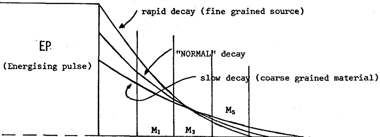
(A) DECAY AS OBSERVED BY IPR-8 MIP RECEIVER PRIOR TO PROCESSING
