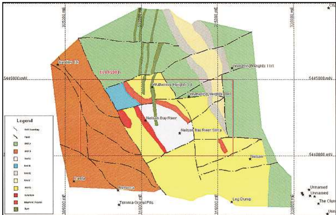
Figure 6: Interpreted Geology Map of EL41/2004
