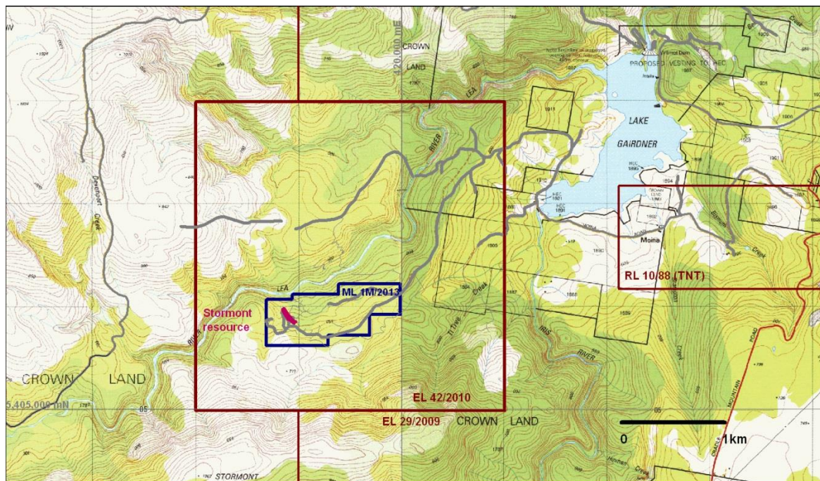
Figure 1.4: EL 42/2010 "River Lea" and previous ML 1/2013 (now reabsorbed into EL 42/2010) showing topography, tracks and prospects – base is 1:25,000 Tasmap (Lea and Cethana sheets).
