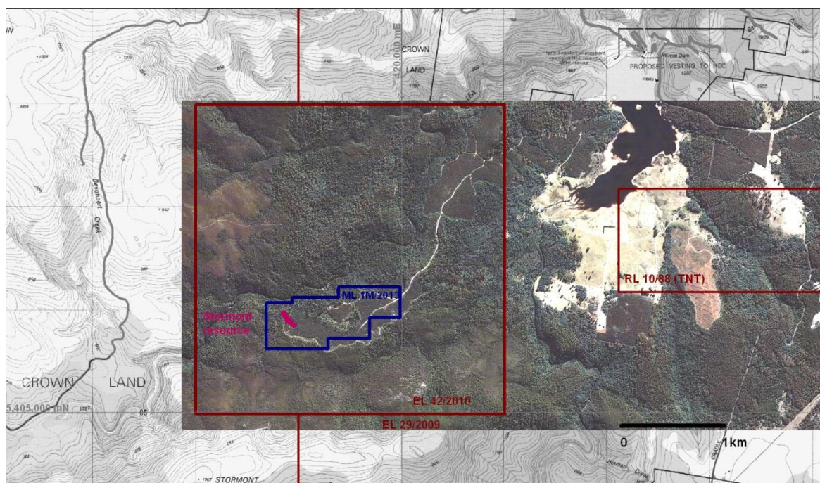
Figure 1.5: EL 42/2010 "River Lea" and previous ML 1/2013 (now reabsorbed into EL 42/2010) showing topography, tracks and prospects – base is orthorectified airphoto
