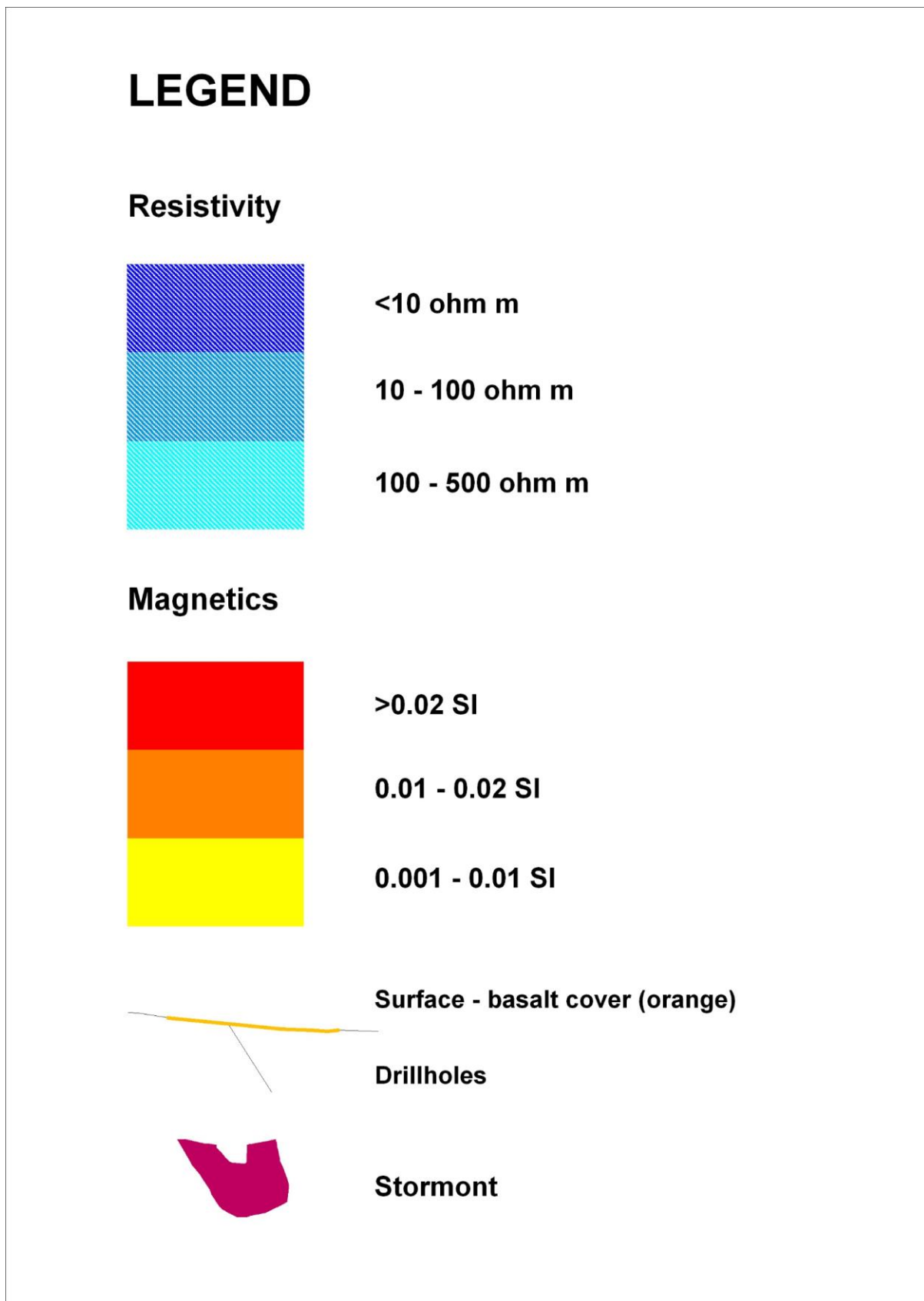
Figure 4.1: Legend for following figures
