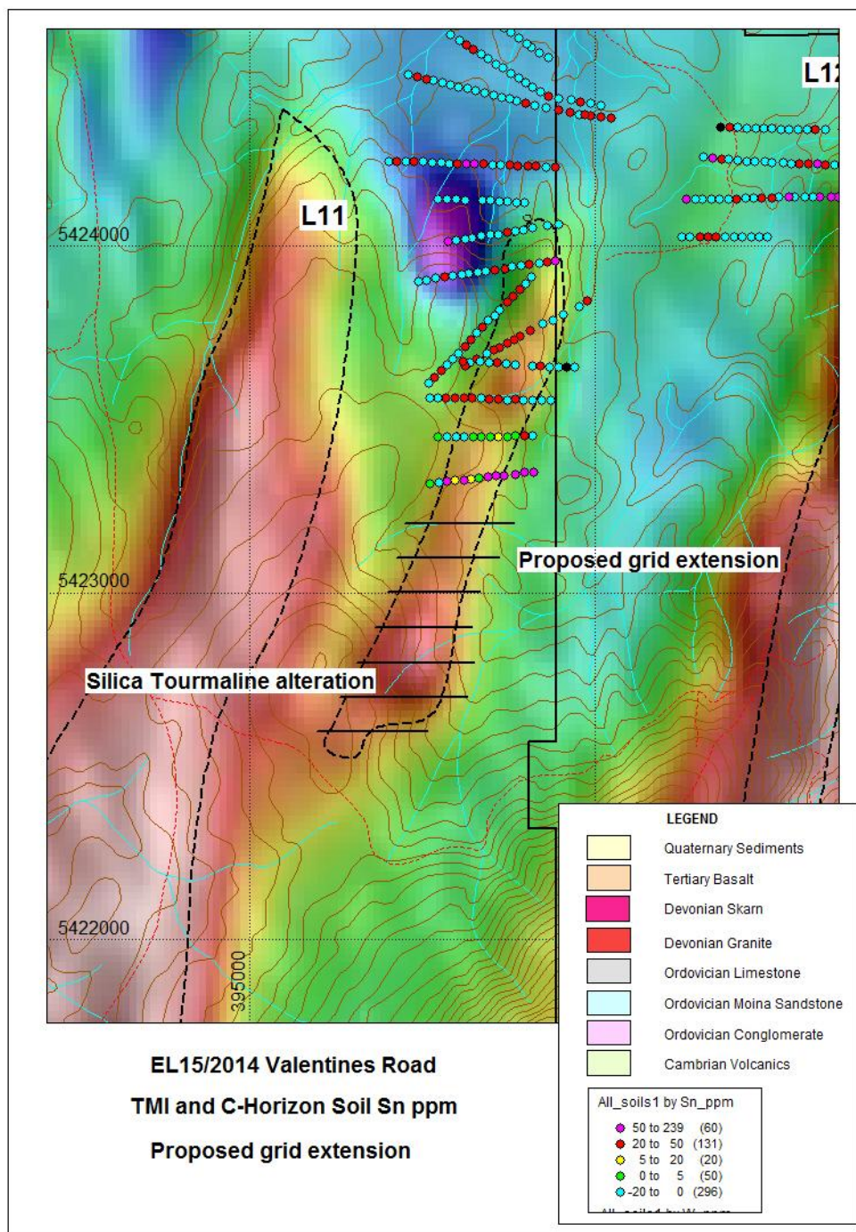
Figure 6. Proposed L11 grid extension, existing soil geochemistry Sn and TMI.
