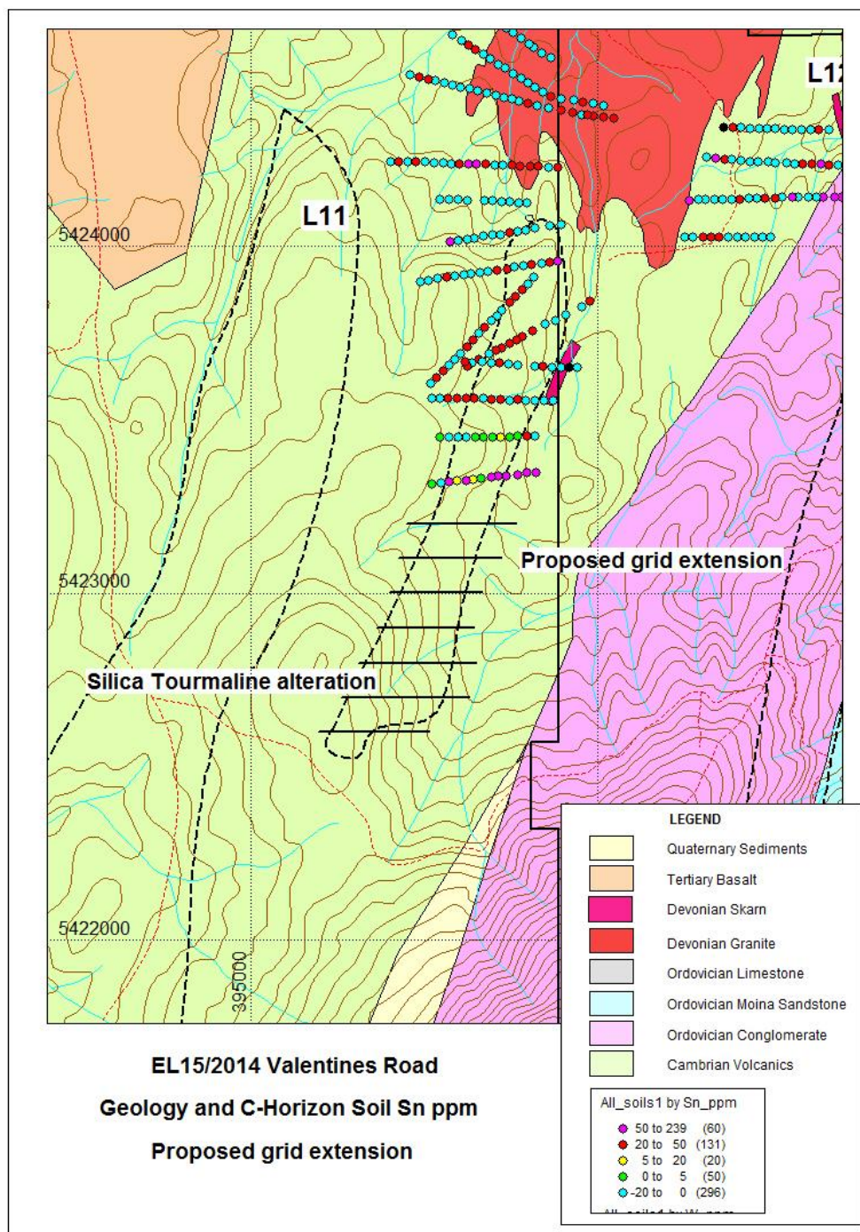
Figure 5. Proposed L11 grid extension, existing soil geochemistry Sn and geology.
