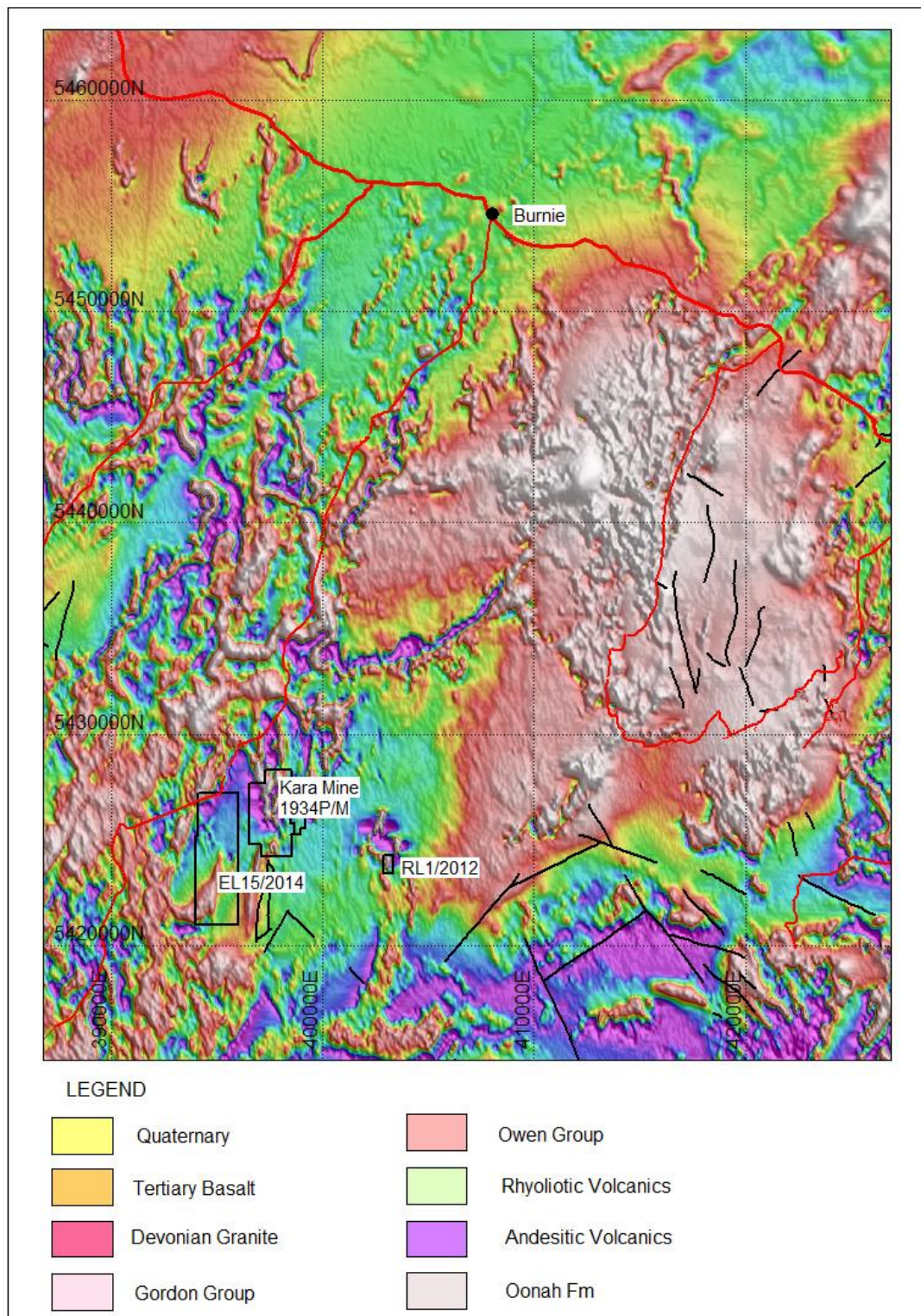
Figure 2. EL15/2014, Kara Mine Lease location and TMI image.
