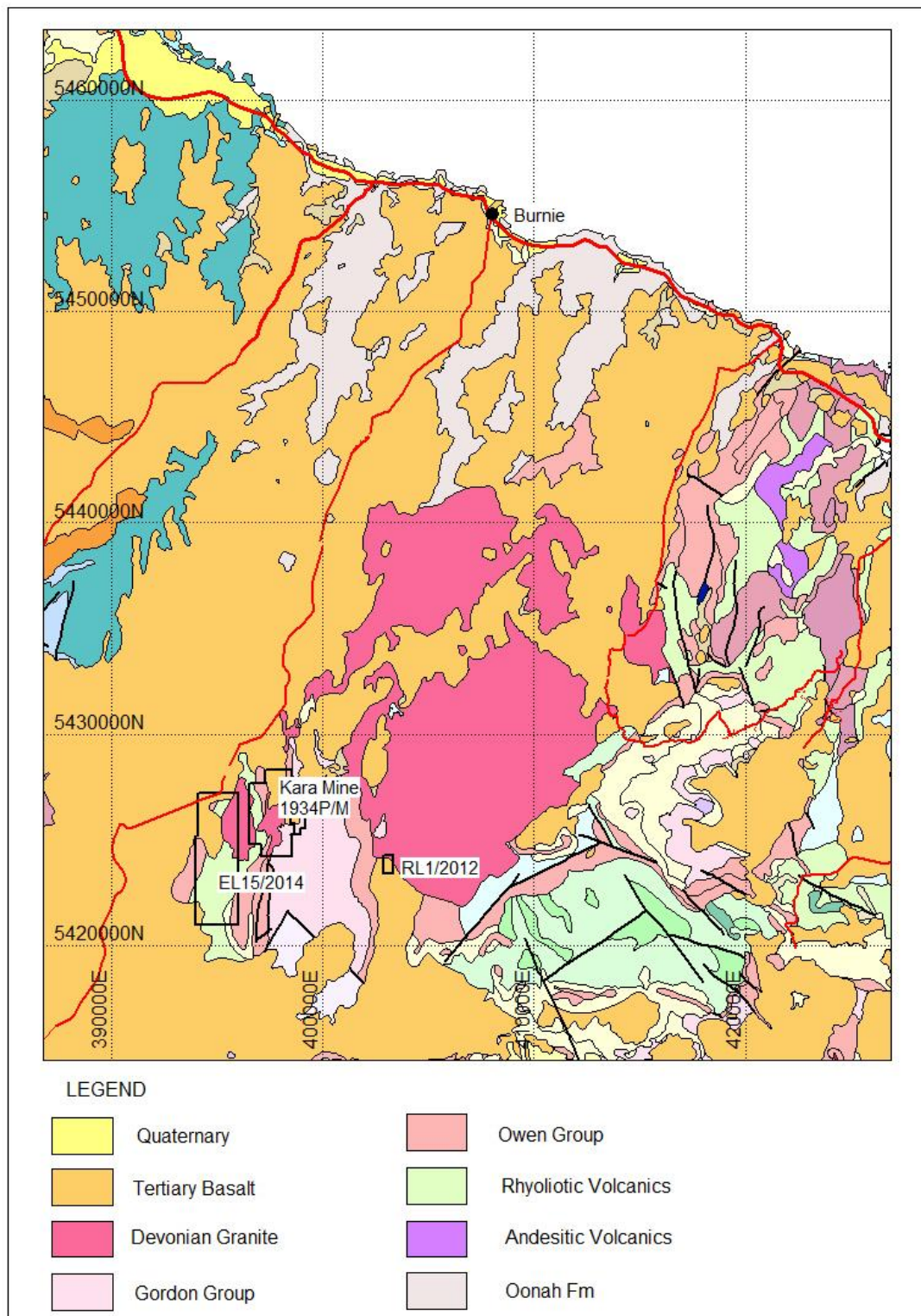
Figure 1. EL15/2014, Kara Mine Lease location and MRT 250k Geology.
