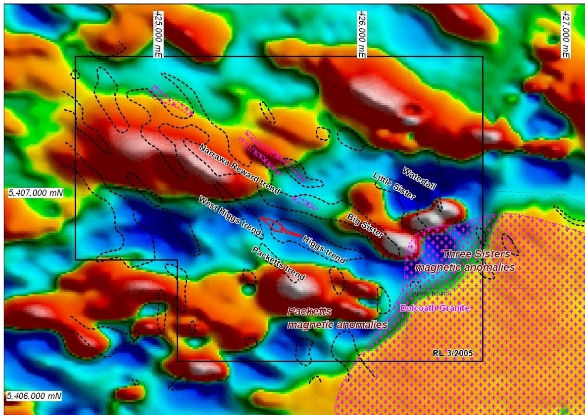
Figure 2.3: RL 3/2005 “Narrawa Creek” area showing 3D IP survey conductivity trends (black dashed lines with black names) as defined by resistivity at 50m depth (closer spaced Narrawa Creek grid data) superimposed on Jervois helimagnetics 2VD RTP colour image showing the Three Sisters magnetics anomalies and the Packetts anomaly. Dolcoath Granite as pink crosses with dashed pink outline, also granitic dykes shown. Higgs resource as maroon outline shown as reference.
