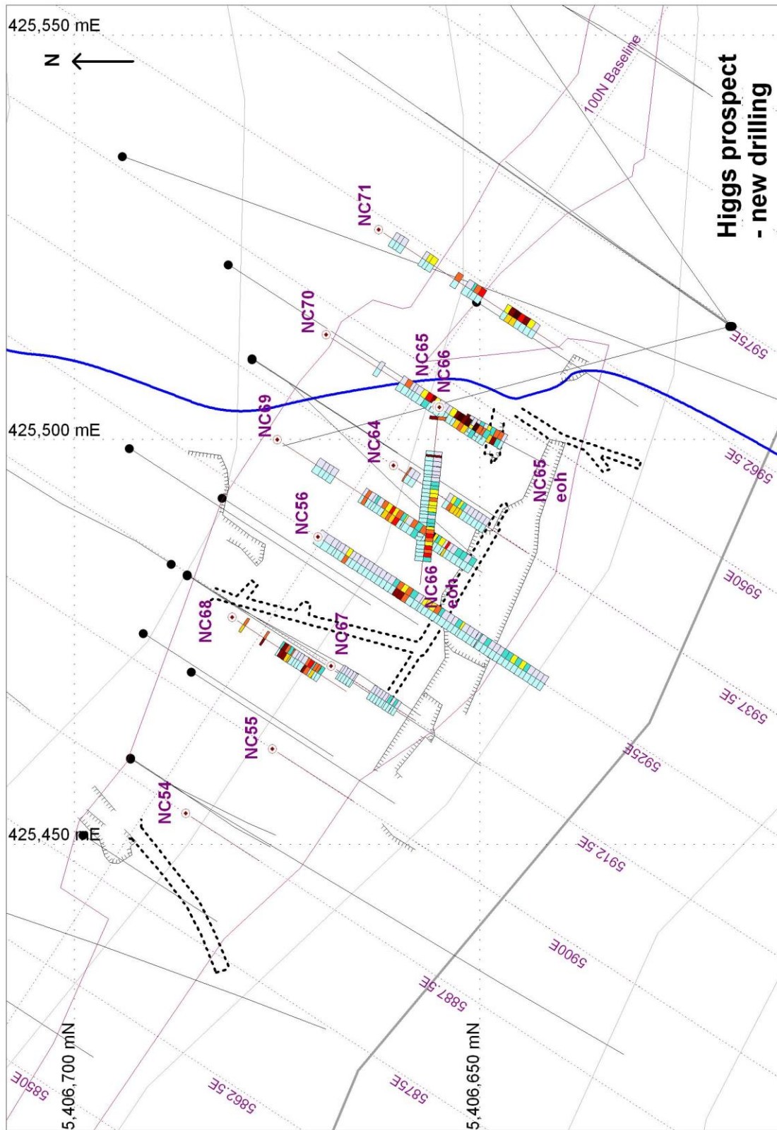
Figure 2.6: Plan view Higgs prospect showing new DDH's NC54 to NC71, Higgs resource outline (red), old workings and channel samples with both drill holes and channel samples showing Au on LHS of drill trace and Pb + Zn on the RHS of drill trace. Legend in figure 2.5.
