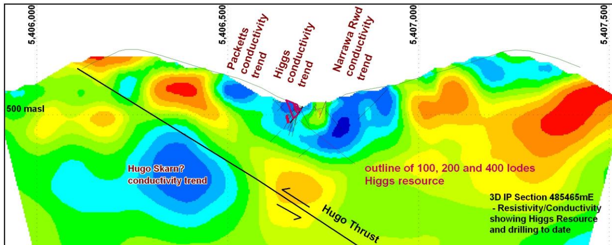
Figure 2.1: Large scale cross-section looking true west showing correspondence of Higgs resource (maroon outline in upper central figure) and resistivity low blue (= conductivity high). Note also Packetts and Narrawa Reward conductivity trends near surface and the Hugo Skarn conductivity anomaly (anomaly lies along strike from TNT Mines Hugo Skarn deposit) beneath the Hugo Thrust Fault.
