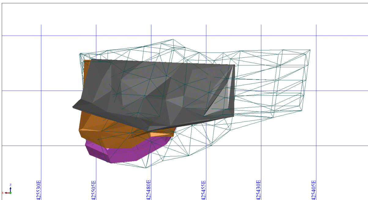
Figure 2.9: Higgs remodelling. No.2 Lode (grey), Main HW Lode (yellow) and Main FW lode (pink) within 100 lode wireframe from Mueller (2009). View looking south.
