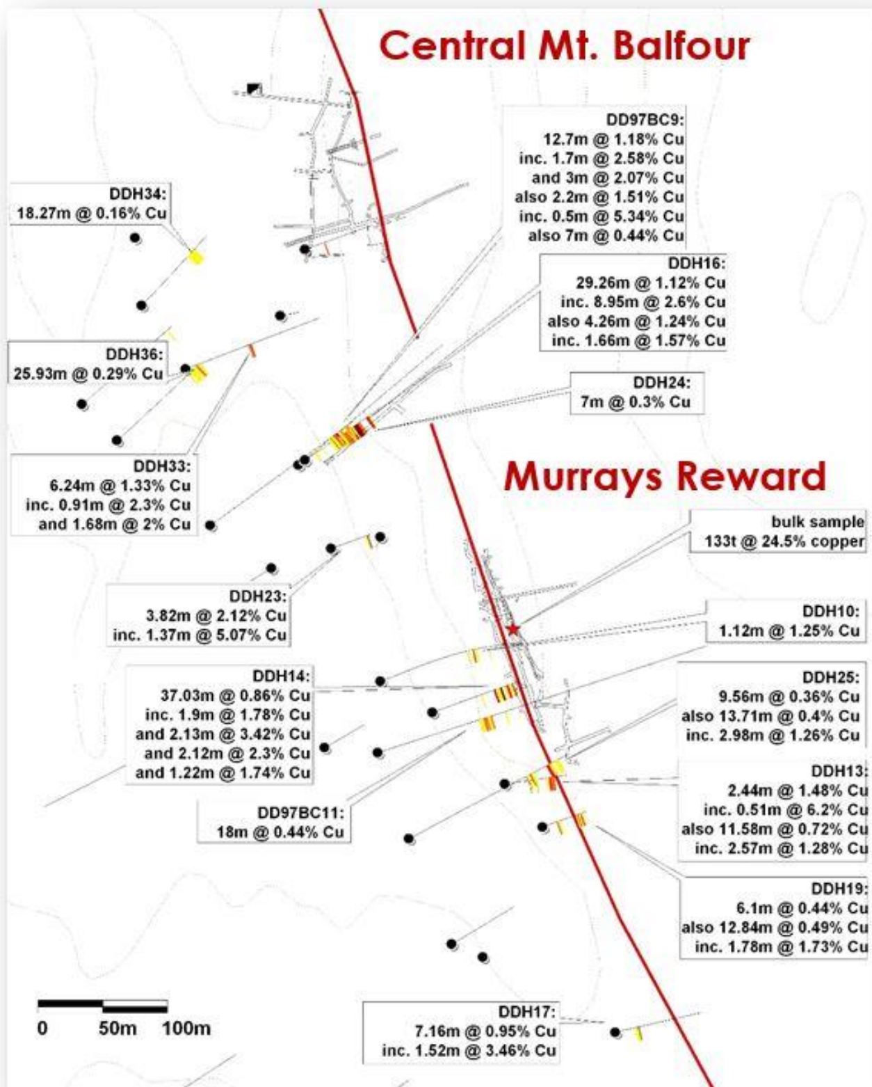
figure 3.10: Plan of drill holes (black dots) and traces (black lines) around the old mine workings of the Murrays Reward and Central Mt Balfour mines. Colour coded copper grades are shown on the drill traces where above 0.1% – for legend see figure 3.11 below.
