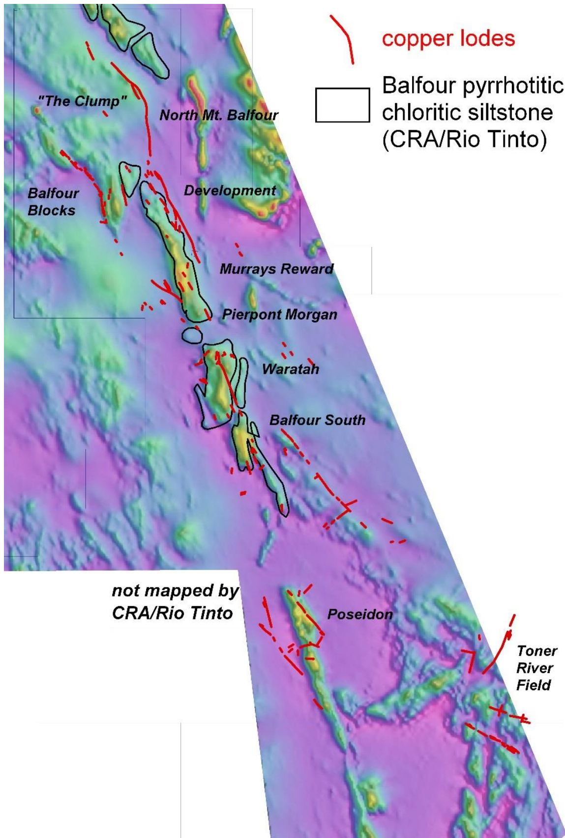
figure 4.4: Regional aeromagnetics image – 1 st vertical derivative showing the extent of the pyrrhotite bearing siltstone unit as mapped by CRA/Rio Tinto.
