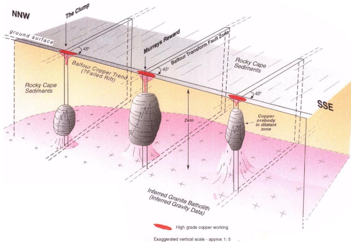
figure 3.9: CRA Proposed Model of Copper ore body
