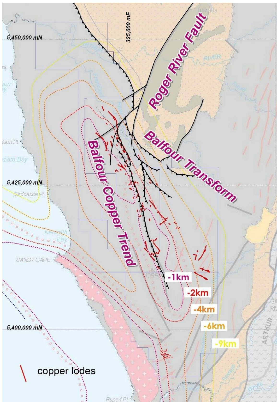
figure 2.2: Simplified geology of the Balfour showing the positions of the major structural elements. Coloured dashes are depth contours to granite and define a shallow ridge coincident with the Balfour Copper Trend. The contours are after and indicate the granite at <1km, shallower than Leamans <2km.
