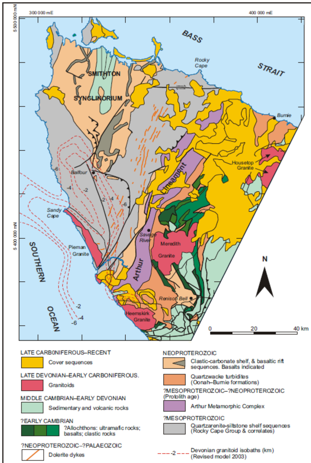
figure 2.1: 1:500,000 scale geology of northwest Tasmania showing the Smithton Synclinorium (or Trough), Arthur Lineament, granite depth contours and Balfour (Taheri and Bottrill, 2004).
