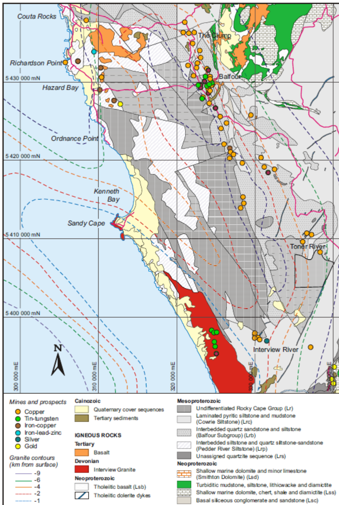
figure 2.3: Local geology of the Balfour copper belt (orange dots) showing the distribution of such units as the Balfour Subgroup and Cowrie Siltstone referred to in text (Taheri and Bottrill, 2004).
