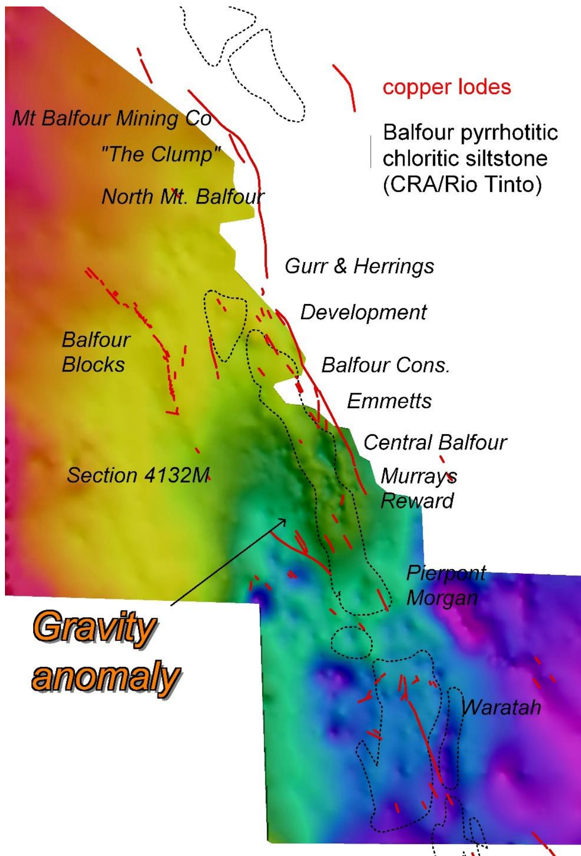
figure 4.5: Regional gravity data set showing gravity anomalism parallel but offset to the west. Gravity low probably represents a ridge of granite. Note association between pyrrhotitic siltstone and gravity high – also magnetics.
