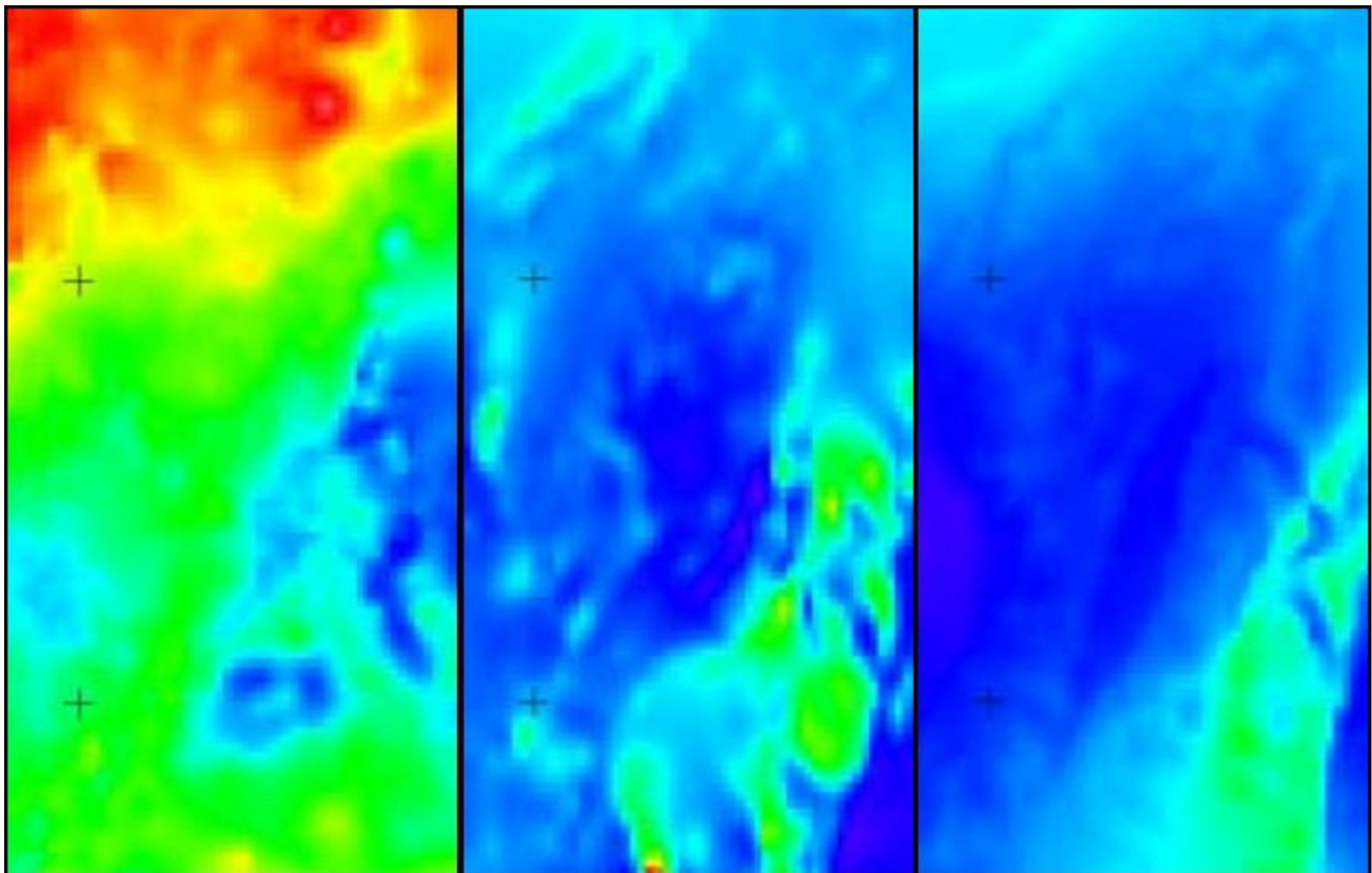
Figure 2. Triptych showing observed Bouguer gravity field derived from the MANTLE-09 2009 program with minimum curvature interpolation (left), observed total magnetic intensity with IGRF removed (middle) and calculated TMI response from the MRT's 2013 inversion model (right). Note the magnetic low in the right image has an en-echelon shape.
