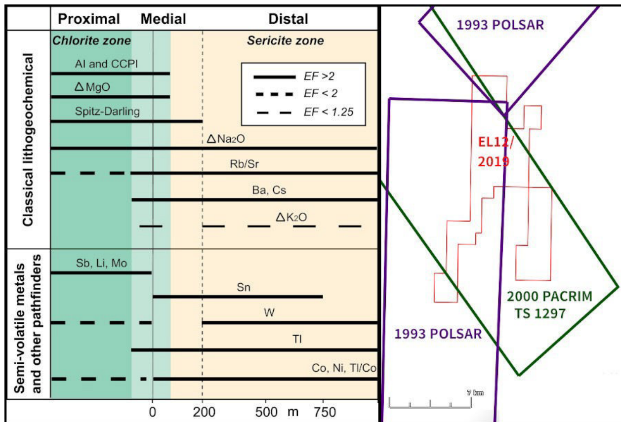
Figure 9 VMS pathfinder minerals (left) and synthetic aperture radar coverage (right)
