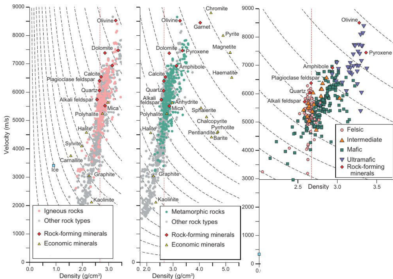
Figure 9 Compilation of published seismic velocity and density measurements of igneous (left) and metamorphic (centre) rocks for pressure-temperature conditions occurring in the upper 1km of the Earth's crust with selected rock-forming minerals and economic minerals identified. The (right) graph shows v/p for igneous rocks and selected minerals showing a rough correlation between how silicic the rocks are and their seismic properties. Also note that the mafic and ultramafic rocks show greater scatter than the other types (due to serpentinisation?).
