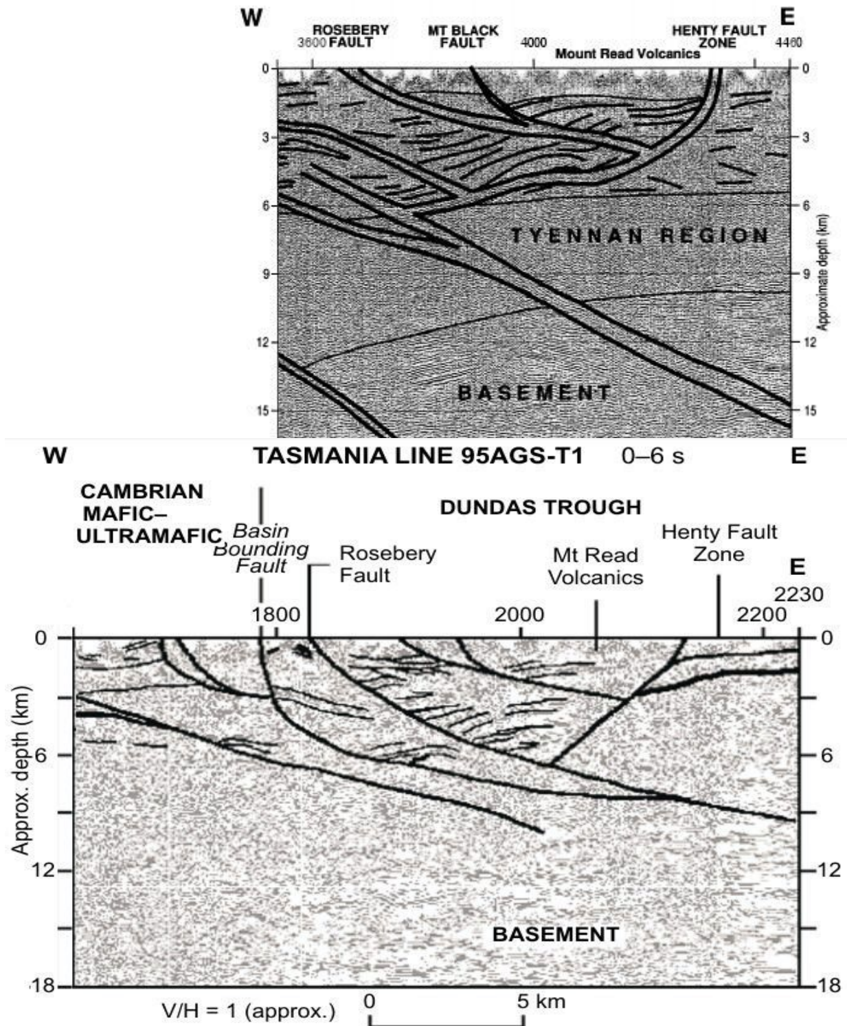
Figure 5 Aligned original interpretations of the eastern half of seismic line 95AGS-T1.
