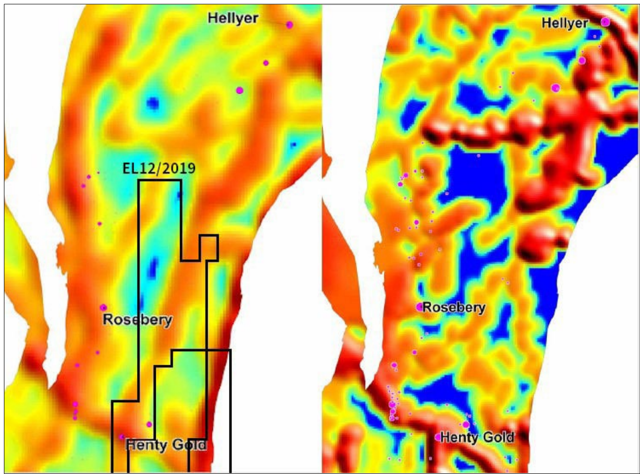
Figure 10 VMS, total edge length and EL12/2019 (left) and total worm relative depth (right)
