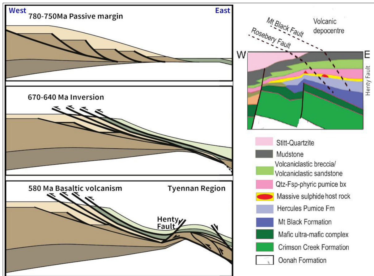
Figure 4 Simplified three-stage tectonic model of the Tyennan Orogeny onset involving collision of the Western Tasmania Terrane (WTT) with an island arc off to the east (left). The pale green unit is ophiolite that has been back-thrust onto the WTT. The coloured cross-section (right) is of the same area but shows the area post-MRV deposition, west-east stratigraphic relationships and principal faults (the low-angle fault Rosebery and Mt Black thrust faults and the high-angle Henty Fault).
