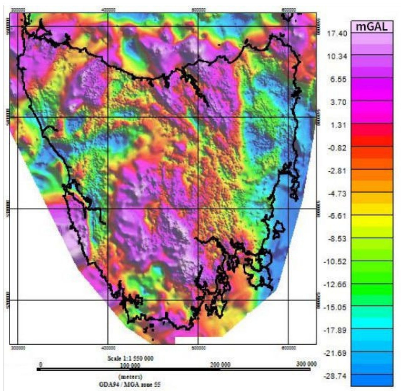
Figure 3 Residual gravity map of Tasmania upon Bouguer anomaly data
