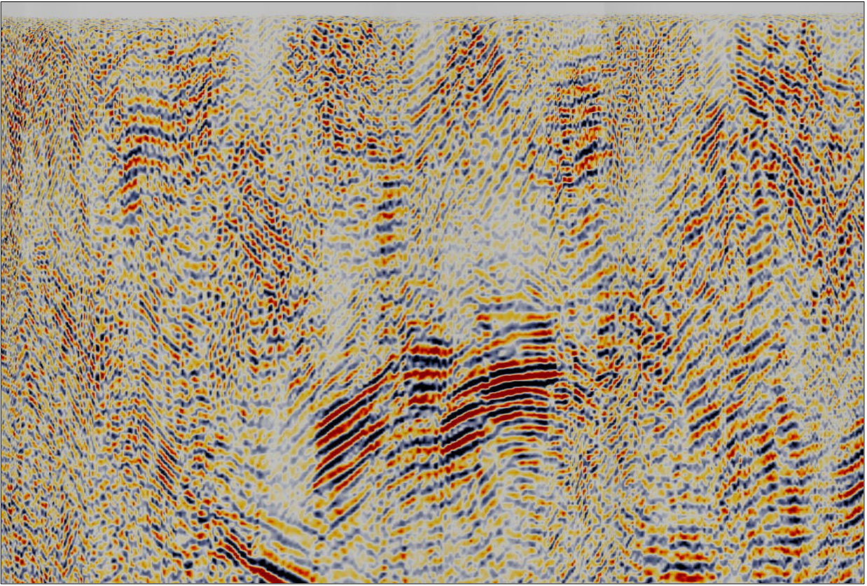
Figure 7. Zoomed segment of 95AGS-T1 1995 (above) and 2020 (below). Horizontal distance is 6.3km. Vertical scale: top of image is 250m AHD and bottom of image -2250m AHD. Ground surface is indicated by the continuous black line near the top of the 2020 reprocessed image.
