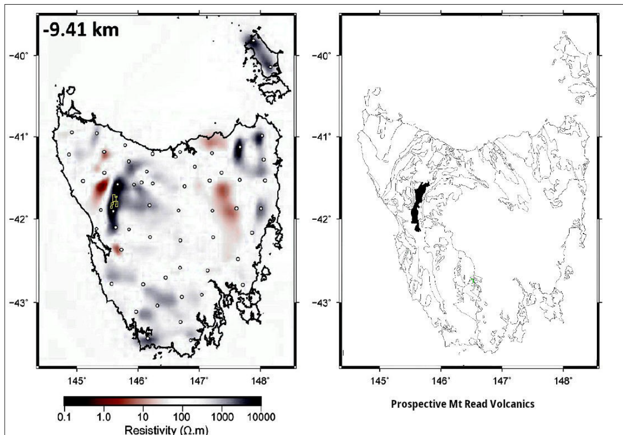
Figure 10. Deep 9.41km resistivity depth slice of Tasmania from the AusLAMP MT project.
