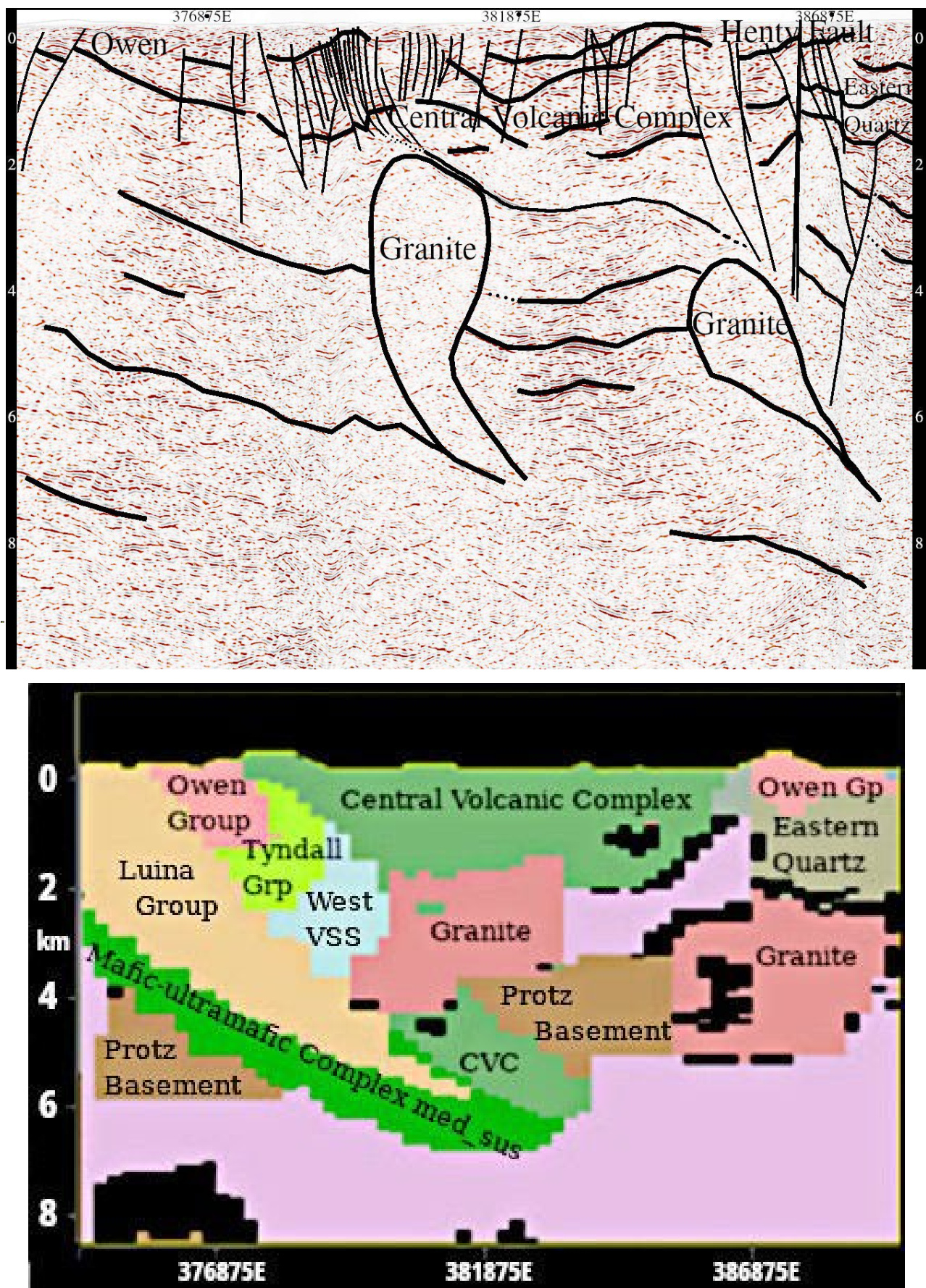
Figure 8 Seismic interpretation of 95AGS-T1 (above) and magnetotelluric interpretation (below)
