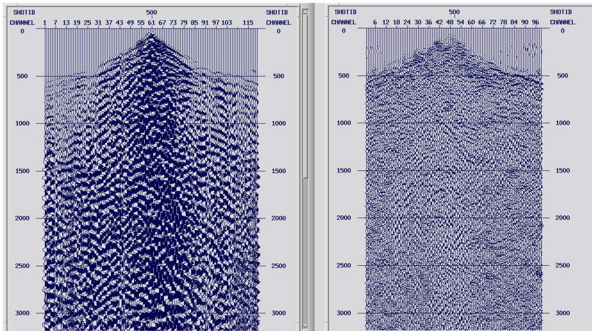
Figure 4 Shot records before (left), after (right) shot domain noise attenuation and dip filter.
