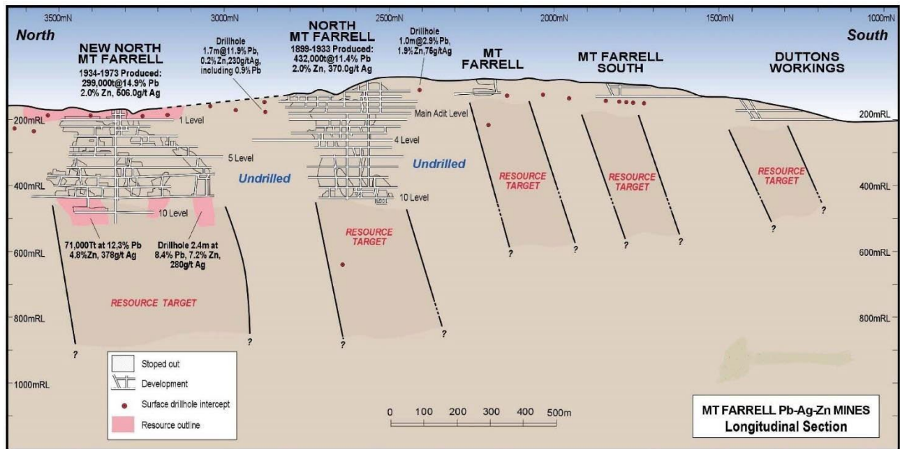
Figure 3. Longitudinal Section running North to South along Mineralised Trend
