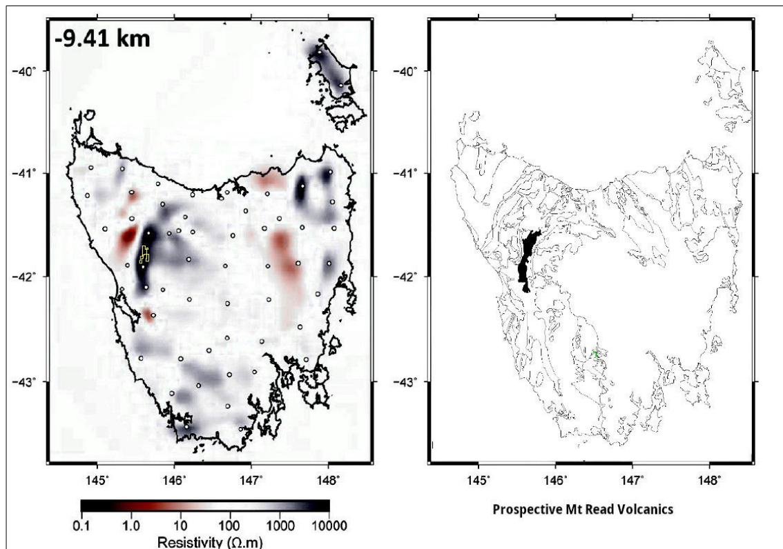
Figure 8 AusLAMP magnetotelluric results showing a) resistivity depth slice at -9.41km with yellow tenement location (left) and geological map with MRV in black (right).
