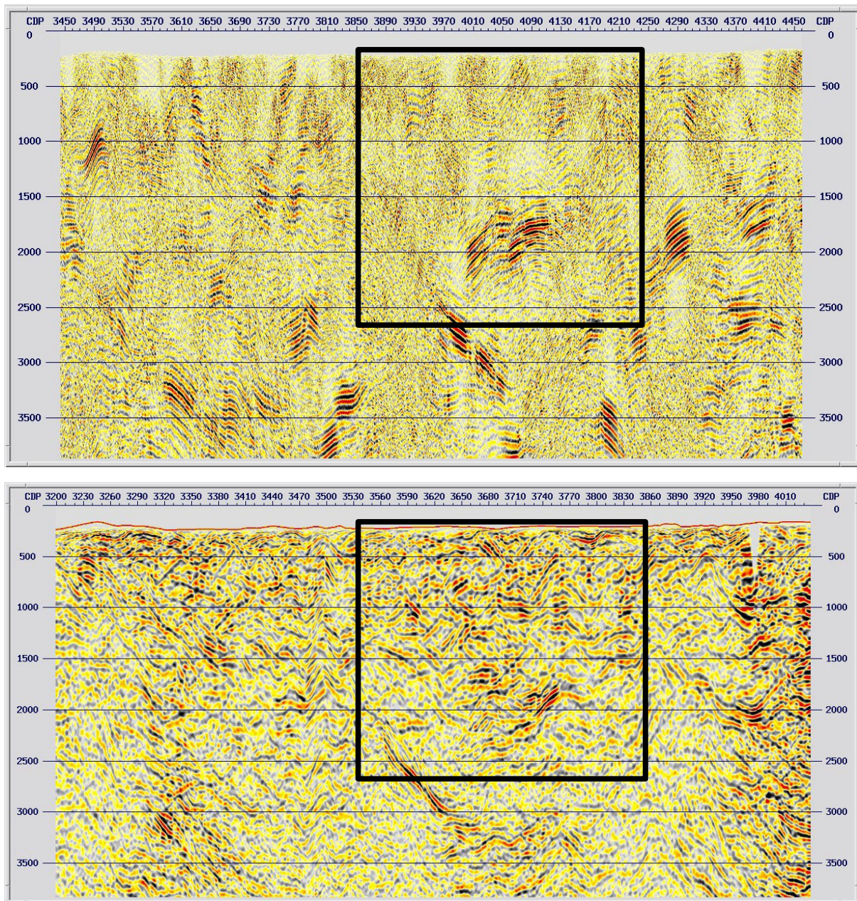
Figure 6. Migration in depth of the 1995 reprocessing (above) and 2020 reprocessing (below). The black box indicates the area zoomed in Figure 7.
