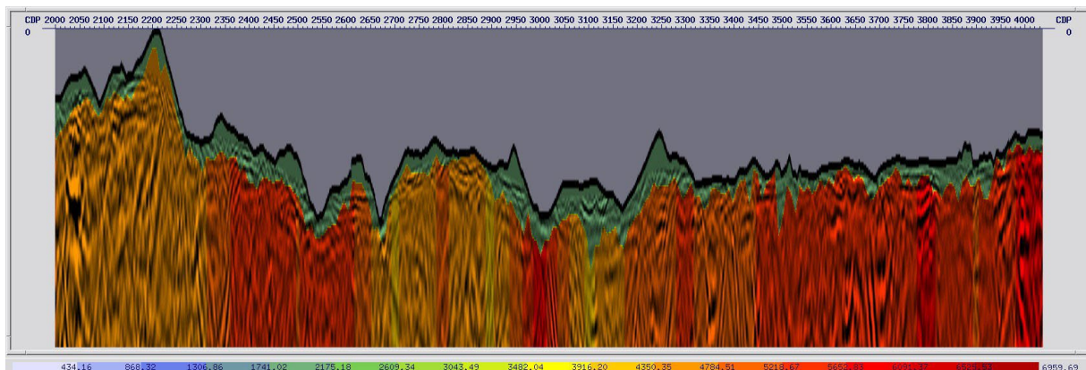
Figure 5 Line 95AGS-T1 with interval velocity overlain. Note velocity scale on the bottom.
