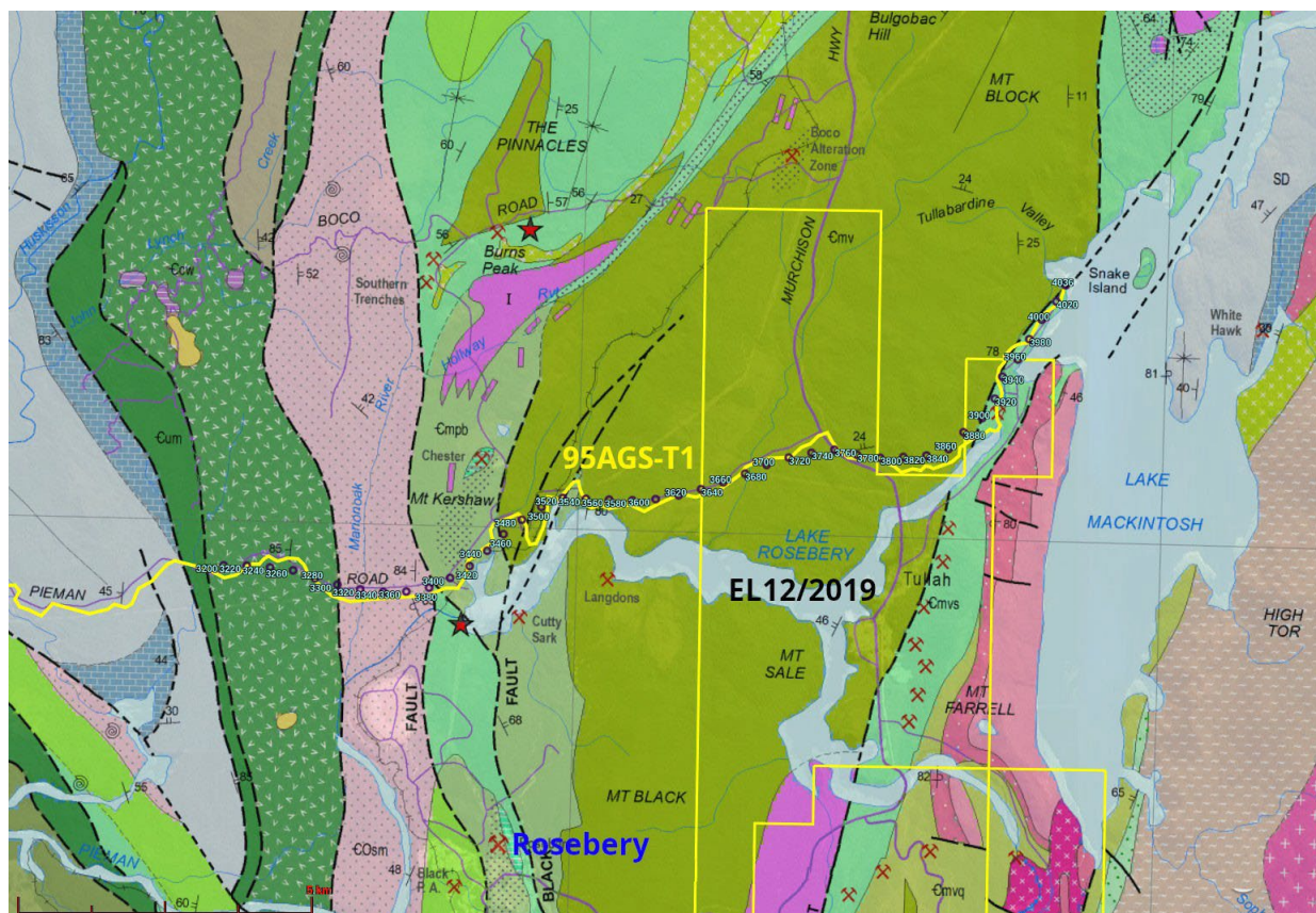
Figure 1. Location maps of seismic line 95AGS-T1, tenement EL12/2019, mines and geology.
