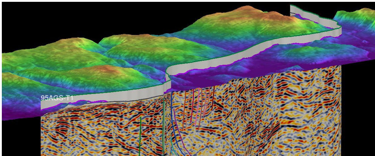
Figure 2. Seismic line 95AGS-T1 with 3D, coloured, elevation profile, looking north.
