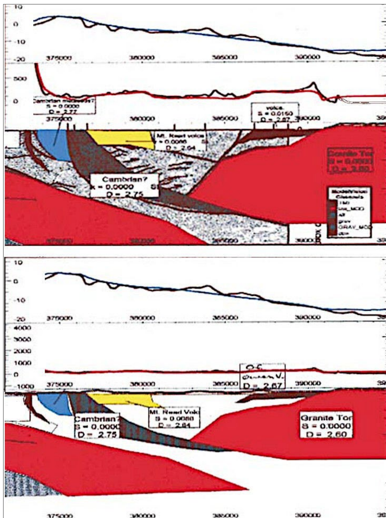
Figure 6 Modelling of gravity (above) and TMI data (below) eastern part of line 95AGS-T1.
