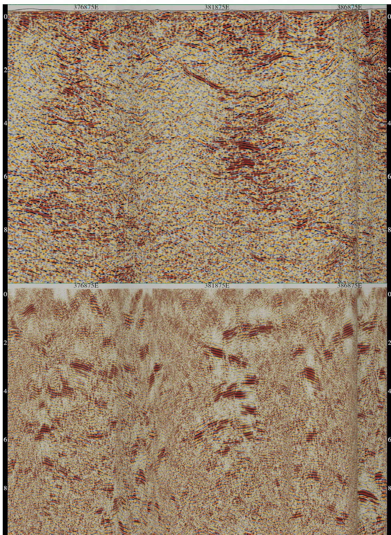
Figure 7 Seismic reprocessing 2020 (above) and original 1995 processing of 95AGS-T1 (below)
