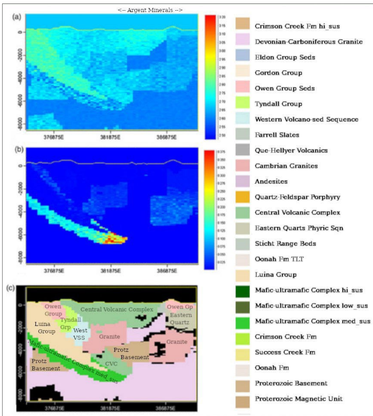
Figure 7 AusLAMP magnetotelluric results showing a) Density (t/m 3 ), b) Magnetic susceptibility (SI) and c) Geology across Rosebery with longitude indicated.
