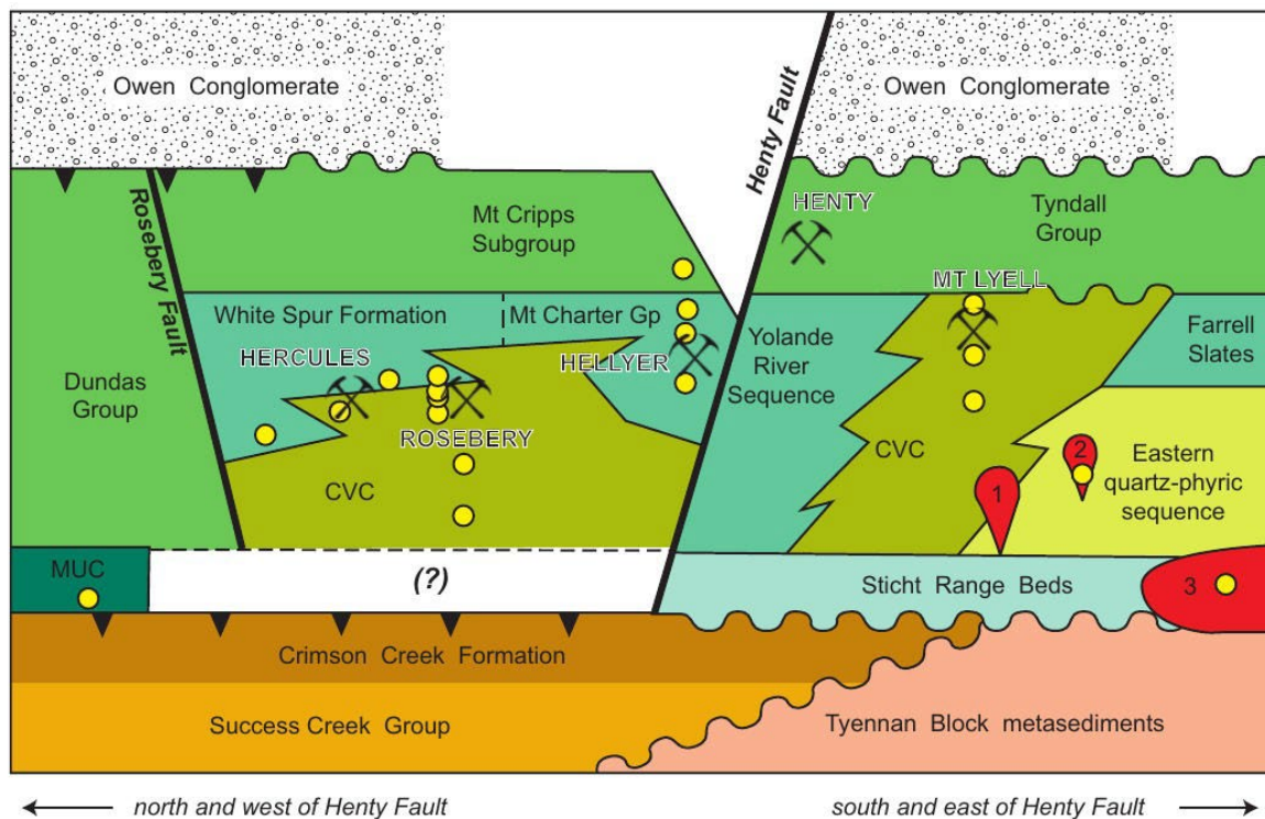
FIG. 2. Simplified stratigraphic relationships within the Mount Read Volcanic belt, showing the approximate stratigraphic position of the main VHMS deposits in the belt, as well as each of the samples dated in this study (modified after Martin, 2004). The numbered units are the Darwin (1) and Murchison (2) granites and the Bonds Range Porphyry (3).
