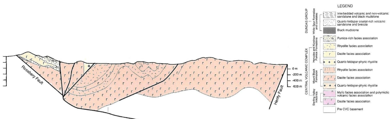
Figure 11 from Gifkin's PhD of cross-section through 5380000m S, parallel to the seismic section.
