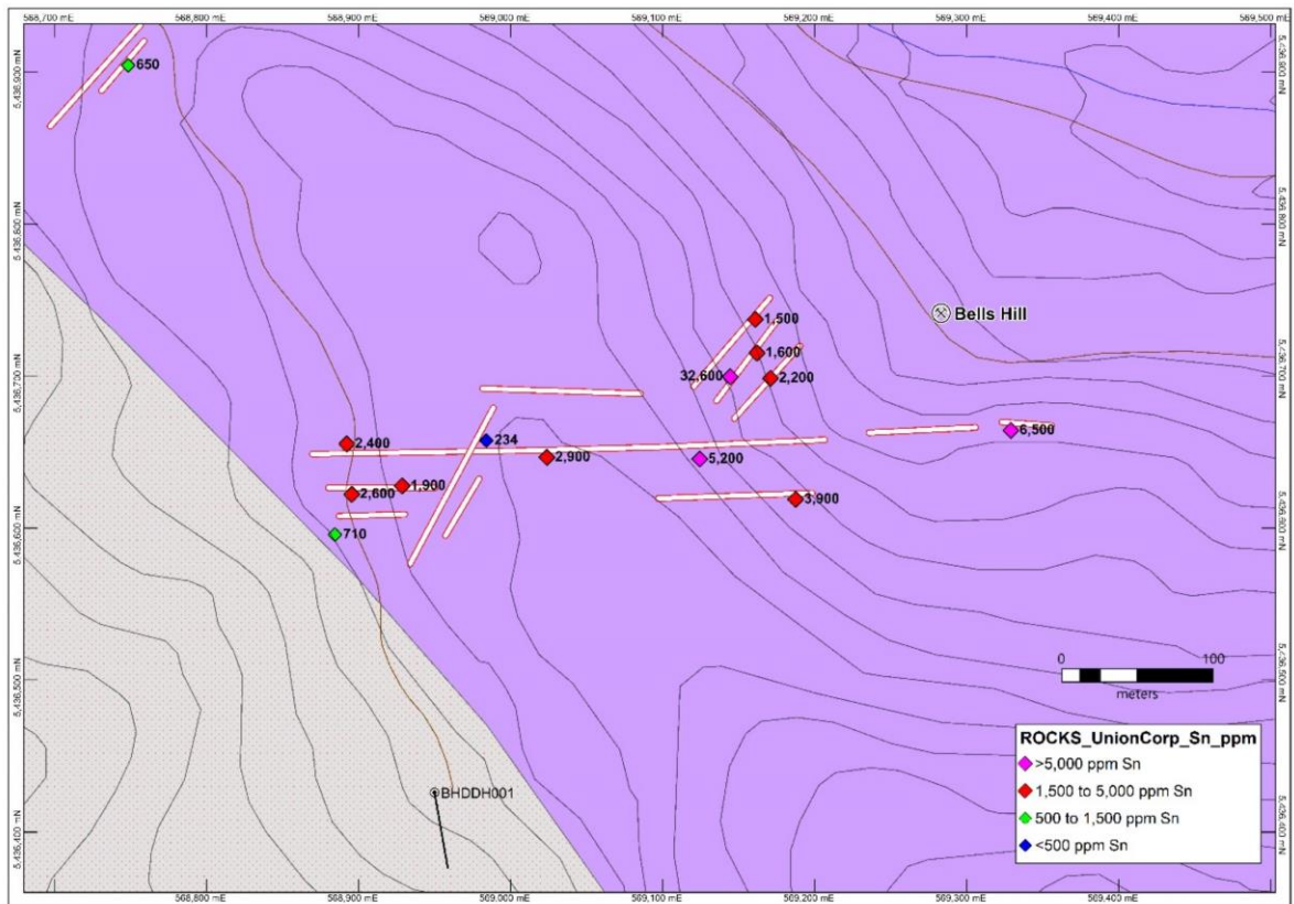
Figure 6. Bells Hill prospect area with surface rock sampling Sn assays by Union Corp (1982). See Figure 2 for legend. Adapted from Winnall (1982).
