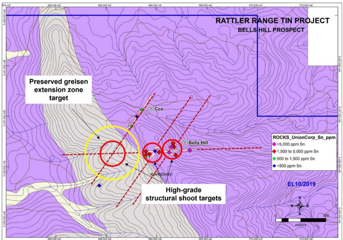
Figure 7. Summary of possible target zones at the Bells Hill prospect.
