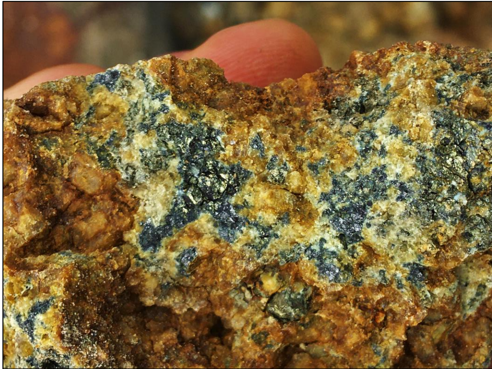
Figure 10. Sulphide-bearing greisen from Mammoth prospect.
