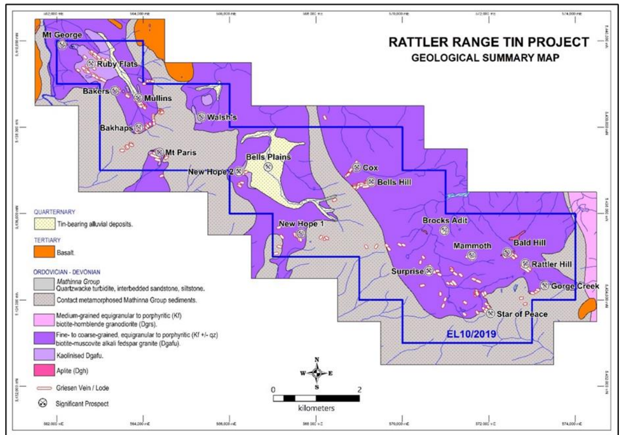
Figure 2. Geology map of the tenement area (adapted from the MRT 1:25,000 scale digital geology and other sources).
