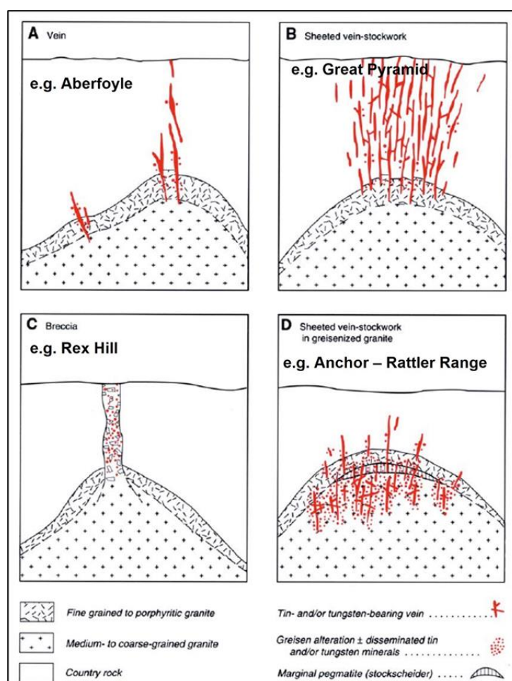
Figure 3. Generalised models of tin mineralisation styles in northeast Tasmania.
