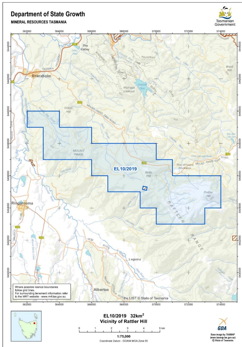
Figure 1. Location plan showing the EL10/2019 tenement area (MRT supplied).
