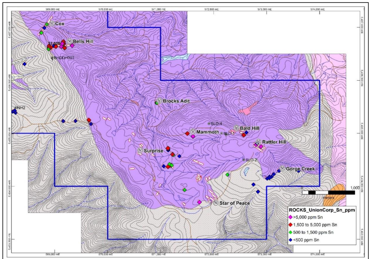
Figure 4. Geological map of priority exploration target areas with surface sampling Sn assays by Union Corp (1982). See Figure 2 for legend.
