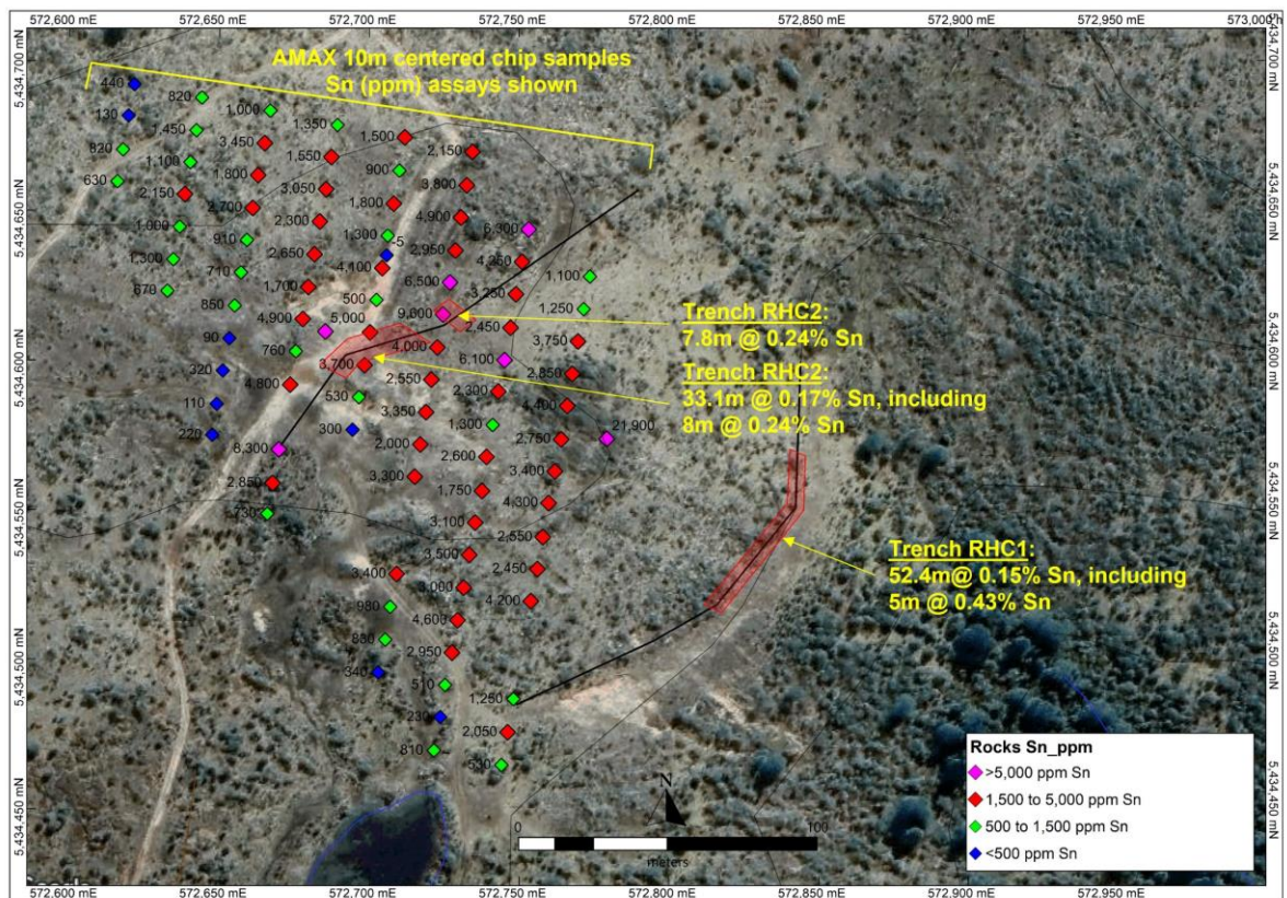
Figure 8. Summary of surface gridded rock sampling and costeaning by Amax Australia (1982-83) at the Rattler Hill prospect (adapted from Yeates (1982) and Vivian (1983)).
