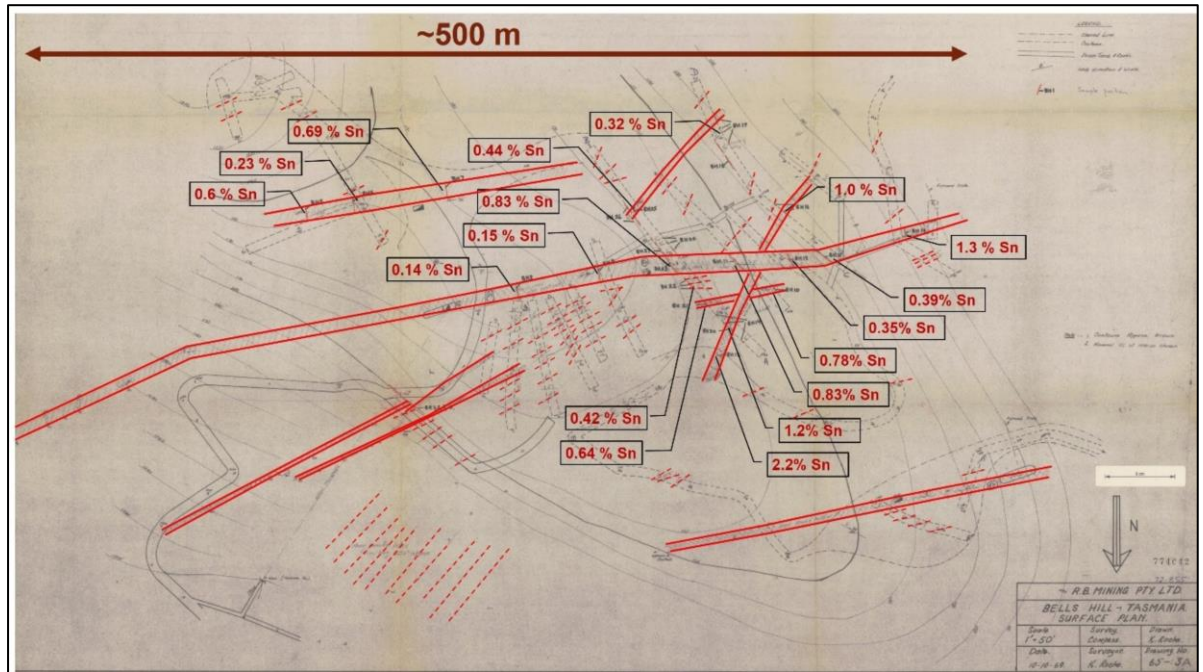
Figure 5. Ringarooma Mining costeaning and sampling plan map (1969) with sampling assays shown. Note: north is towards the bottom of page. Adapted from Groves (1972).
