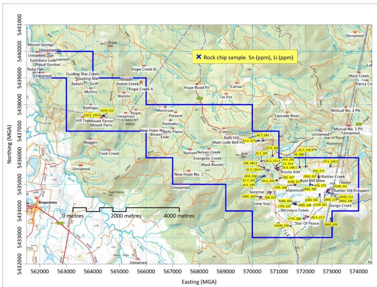
Figure 11. Rock chip sample geochemistry – Sn (ppm), Li (ppm). MRT deposit locations labelled with white shading.
