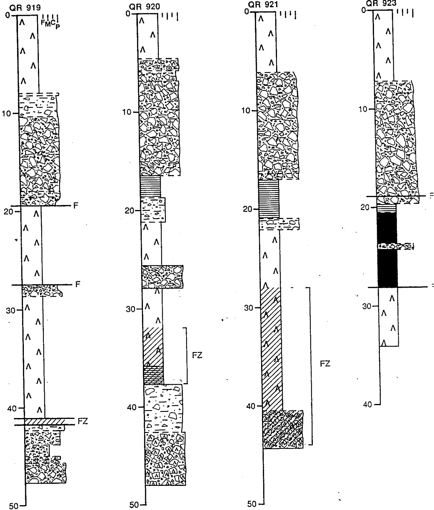
7212.5 N SECTION SCHEMATIC DRILL HOLE LOGS
