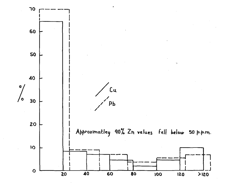
STATISTICAL DISTRIBUTION OF Cu AND Pb RESULTS
